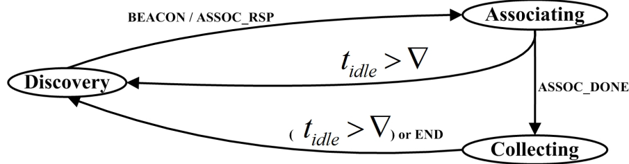
Fig. 5. State Transition Diagram of Mobile Node
