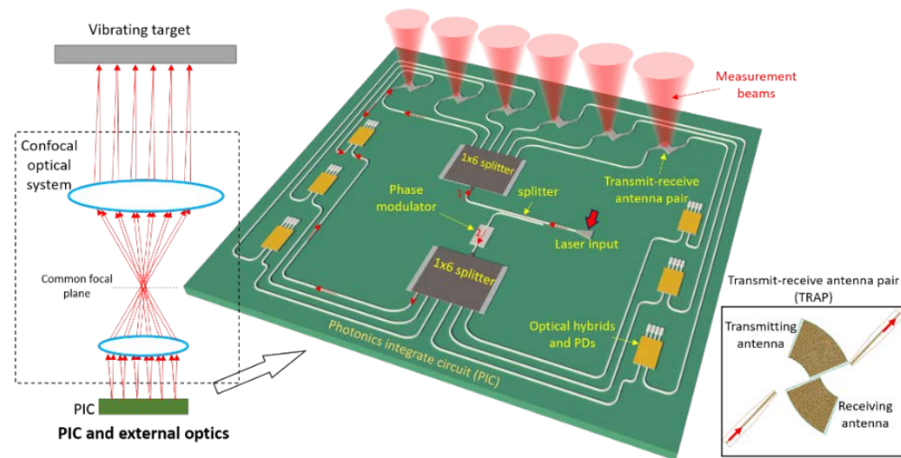
Fig. 1. Schematic show of the external confocal optical system, the six-beam LDV on an SOI-based photonics integrate circuit (PIC) and a transmit-receive antenna pair. The drawing of the confocal system is exaggerated to make the design easier to understand.
