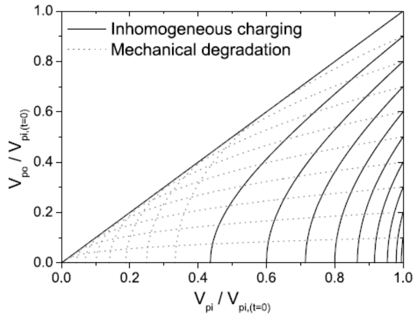
Figure 3.15: Two distinct trends are observed in the decrease of V_{po} (normalised to V_{pi} at t = 0 ) as a function of the normalised V_{pi} as a switch degrades due to non-uniform charging and mechanical degradation [100].
