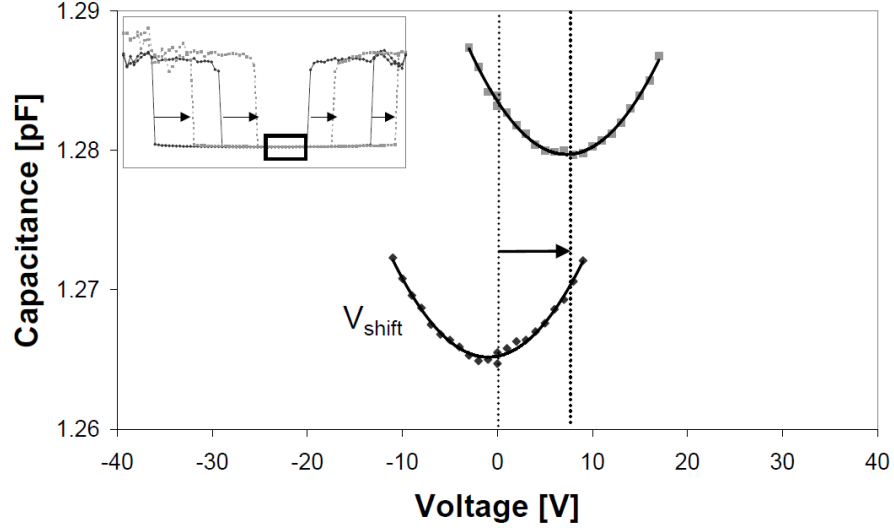
Figure 3.6: A right-shift in the V_{Cmin} of a capacitive switch following DC stress at 65 V for 727 seconds. Inset: the corresponding full C-V curve, from [124].
