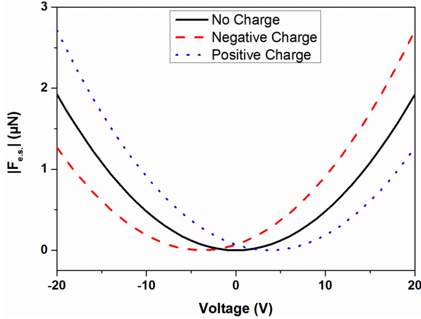
Figure 3.5: The electrostatic force exerted on the top membrane of a capacitive switch as a function of the applied voltage for a fixed air-gap of 3 \mu\text{m} and three different parasitic charge densities of zero (solid black line), -10 \times 10^{-4} C/m 2 (dashed red line) and +10 \times 10^{-4} C/m 2 (dotted blue line).
