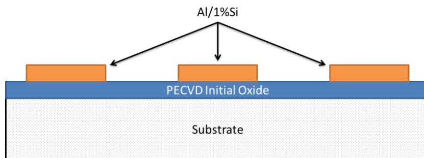
Figure 2.8: Schematic representation of the first three layers of a fabricated device.
