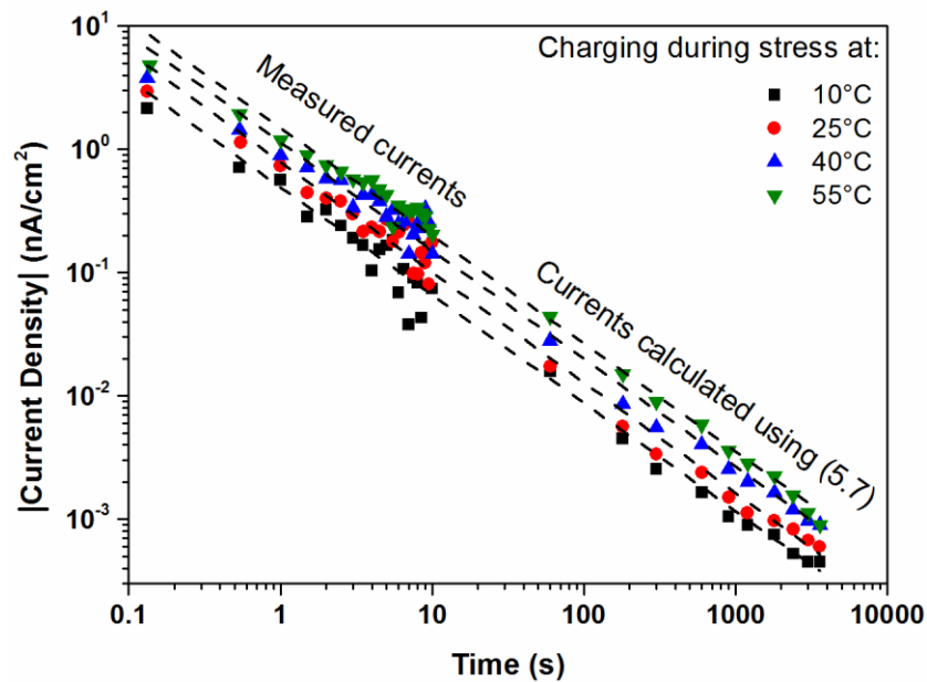
Figure 5.14: Measured and calculated MEMS charging current densities recorded over a range of temperatures at a constant electric field of -2.3 MV/cm. The dashed lines correspond to linear fitting across each data set.
