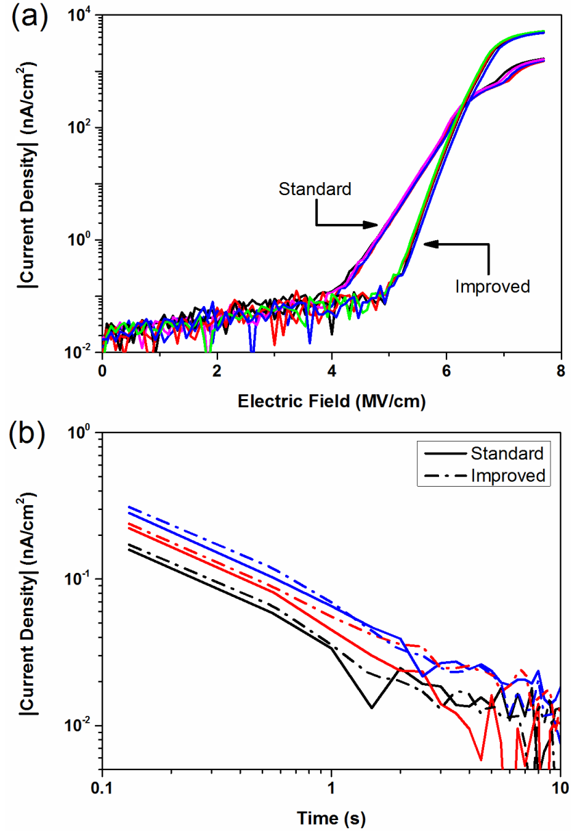
Figure 6.8: J-E characteristics measured on the standard and modified oxides (a) and DCTs recorded on both dielectrics after being charged at 1.9 MV/cm (black), 2.5 MV/cm (red) and 3 MV/cm (blue) (b).
