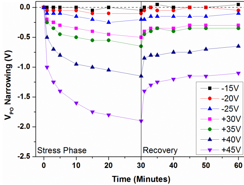
Figure 6.4: Voltage-dependence of the transient and partially-recoverable pull-out voltage narrowing effect.
