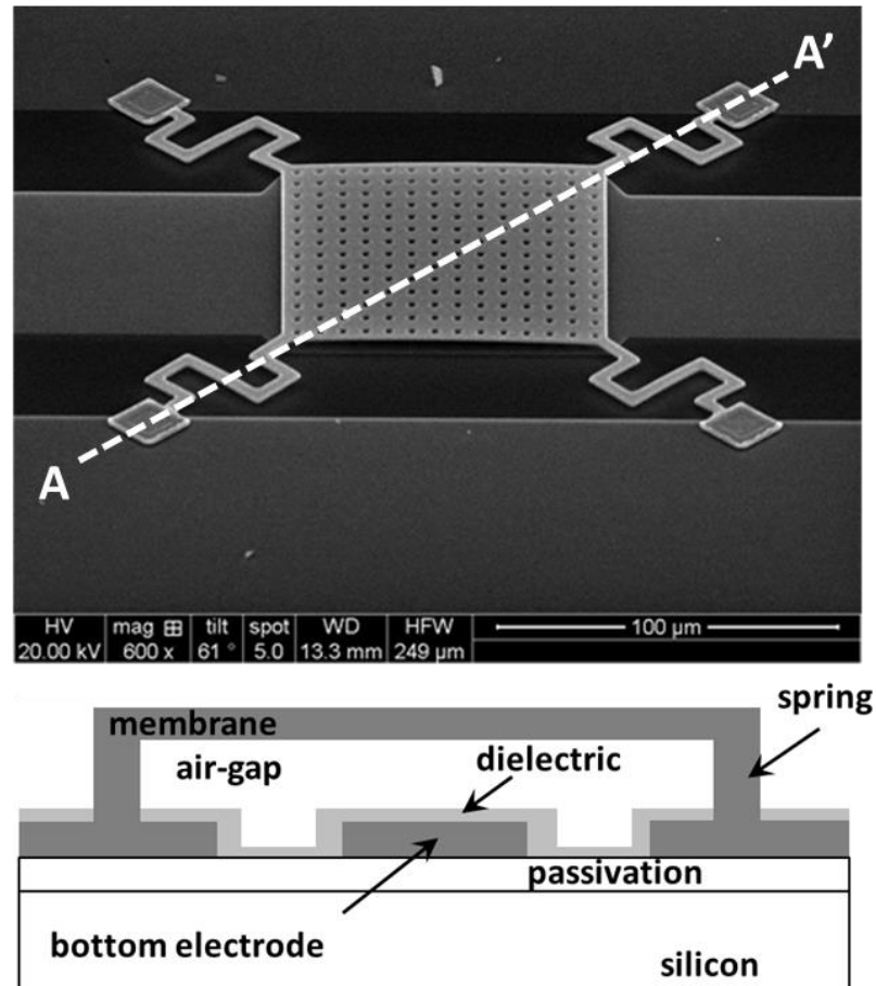
Figure 2.7: SEM image and cross-section of a capacitive switch with meander tethers fabricated at Tyndall. The cross-section is measured along the line A-A' as shown in the SEM image.
