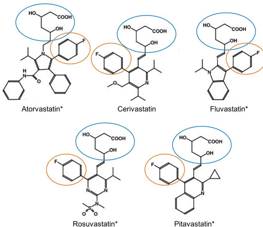
Figure 1: Chemical structures of the statins. Type 1 statins are characterised by a conserved lactone ring (highlighted in blue), a decalin structure (not highlighted) and a butyryl side chain (highlighted in red), which is different in each statin. The type 2 statins differ from type 1 statins due to the replacement of the butyryl side chain with a fluorenyl group (highlighted in orange), and although the lactone ring structure is conserved in all
