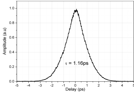
Figure 3. Autocorrelation trace of the output pulses. The pulses duration is about 1.16ps assuming a sech2 profile.
