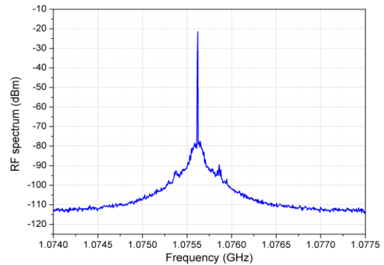
Figure 4. RF spectrum of the output pulses. The repetition rate of 1.0755 GHz is in agreement with the cavity length.
