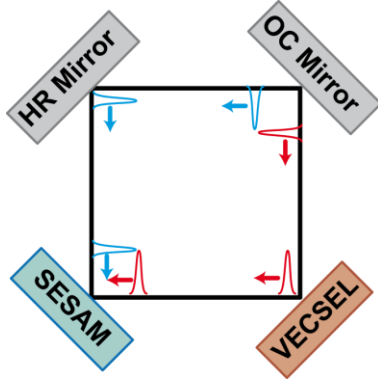
Figure 1. Circulation of the two pulses in a ring cavity system. The two counter-propagating pulses cross in the SESAM.
