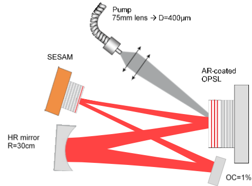
Figure 2. Schematic layout of the colliding pulse modelocked VECSEL.
