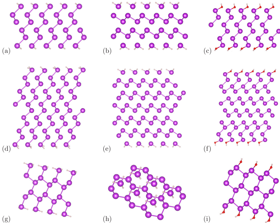
FIG. 4. Thin films with alternative surface terminations. (a), (b), and (c) show the three-bilayer thick films terminated with two H atoms, three H atoms and one -OH molecule per surface atom, respectively. Only the termination with three H deviates from the previous results significantly because it keeps the bilayer orientation intact. (d), (e), and (f) show the corresponding six-bilayer thick films. Here the termination with two hydrogens induces a full reorientation while three H atoms keep the Bi(1 1 1) orientation. The middle bilayers of the -OH-terminated structure have a Bi(1 1 1) orientation, just like in the case of a single hydrogen where the transition occurred between five and six bilayers. Finally, (g), (h), and (i) show a single bilayer of the above three bilayer films including the termination to elucidate the bonding scheme within the structures. This corresponds to a side view or—in case of the three H termination which has a different orientation—a top view of the films.
