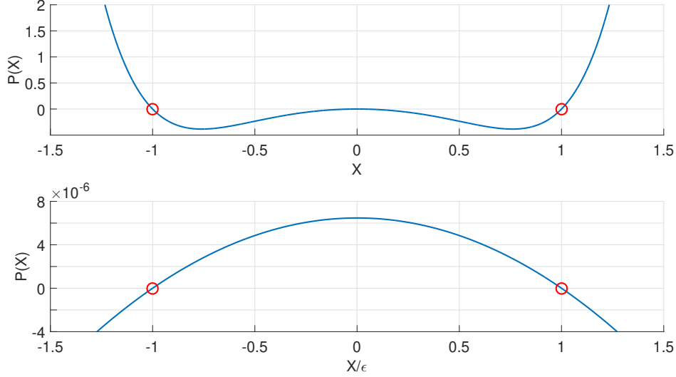
Figure 4: The plot of the polynomial P(X) evaluated at 45^\circ N for (\rho_+ - \rho_0)/\rho_0 = 4 \times 10^{-3} , k = 6.28 \times 10^{-2} \text{ m}^{-1} . The upper plot shows two roots of order O(1) , whereas the lower plot presents two roots of order O(\epsilon) .
