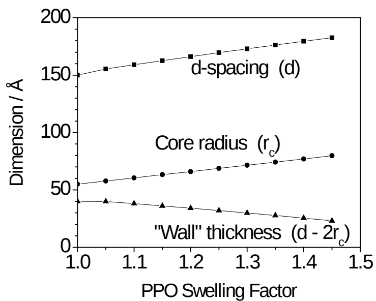
Figure 5 Physical parameters calculated from the SANS model (equation (9)) for the P123 LC micelles at a constant temperature of 40 °C. The PPO swelling factor scale depends on the size of the PPO micelle core.
