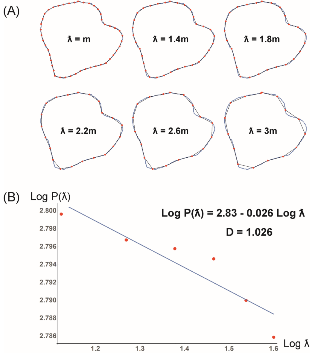
Figure 3.7: Fractal dimension calculation for a grain using the divider method. (a) show the boundary length P(\lambda) of grain measured using increasing unit length \lambda . (b) Plot of \text{Log } P(\lambda) versus \text{Log } \lambda . Slope of the best fit line over the points gives the fractal dimension of the grain D as 1.026.
