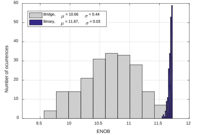
Fig. 10. Monte-Carlo simulation with \sigma_{cu} = 0.5\% .
