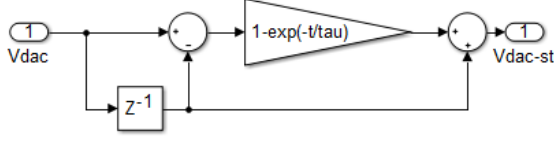
Fig. 5. CDAC finite settling modelling.
