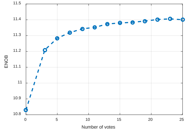
Fig. 11. Majority voting compensation.
