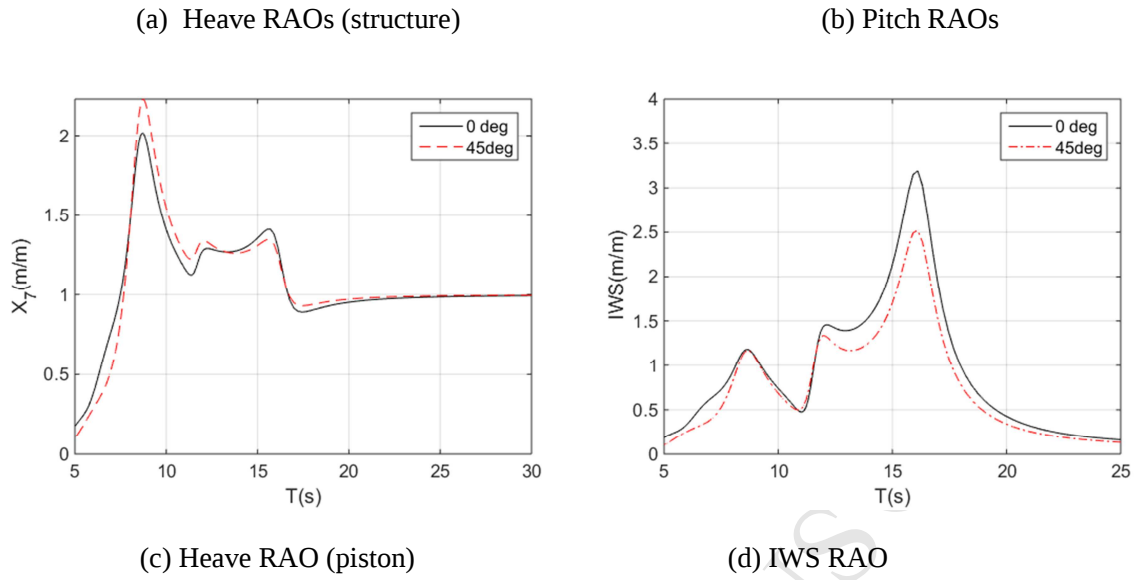
Figure 13 RAO comparisons in head wave and in waves of 45°
