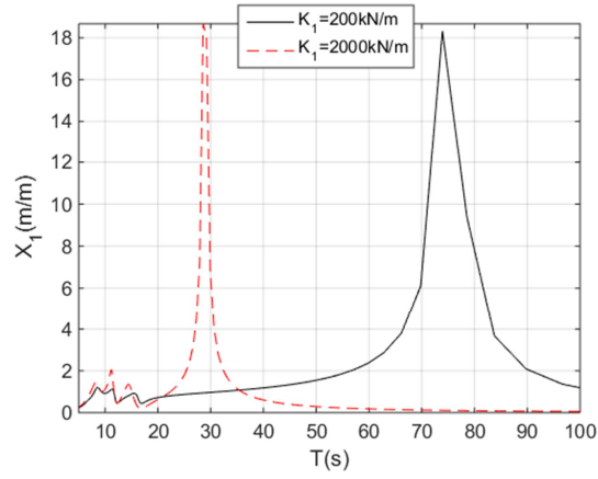
(a) Surge RAOs
