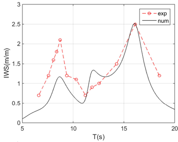
Figure 11 IWS motions in the BBDB RM6 wave energy converter
