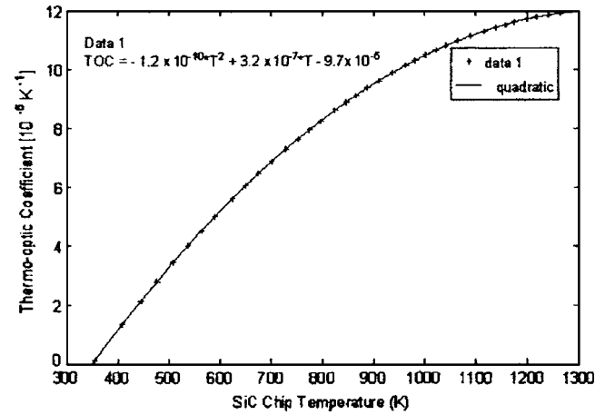
FIG. 4. Calculated 6H-SiC thermo-optic coefficient (TOC) versus SiC temperature at 1550 nm using the Fig. 3 measured cubic fit data for the phase \phi(T) change with temperature. The TOC expression shows a quadratic dependence on the temperature.
