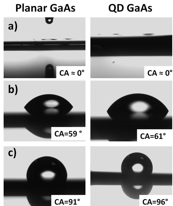
FIG. 3. Photographs of water droplet silhouette on top of epitaxial structures; left panel corresponds to planar GaAs, right to QD GaAs : a) sample after oxygen plasma treatment; b) sample after oxygen plasma treatment and subsequent storage for 1 day; c) sample after HCl etching.
