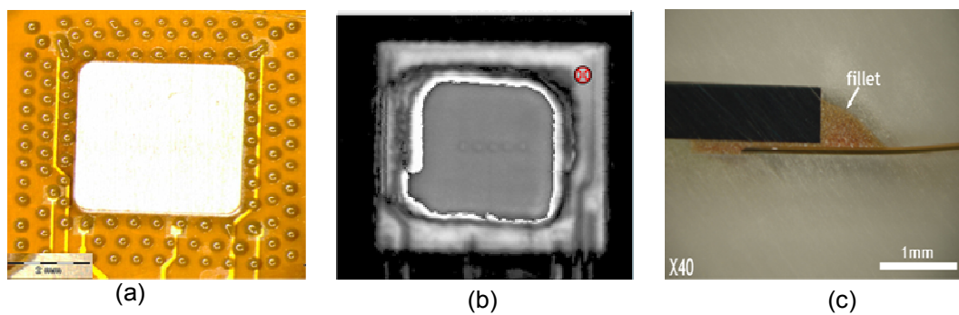
Figure 3.12. The dispense pattern; (a) micrograph of the dispense pattern; (b) SAM image of the dispense pattern and; (c) cross-section showing the filet for the dispense pattern.
