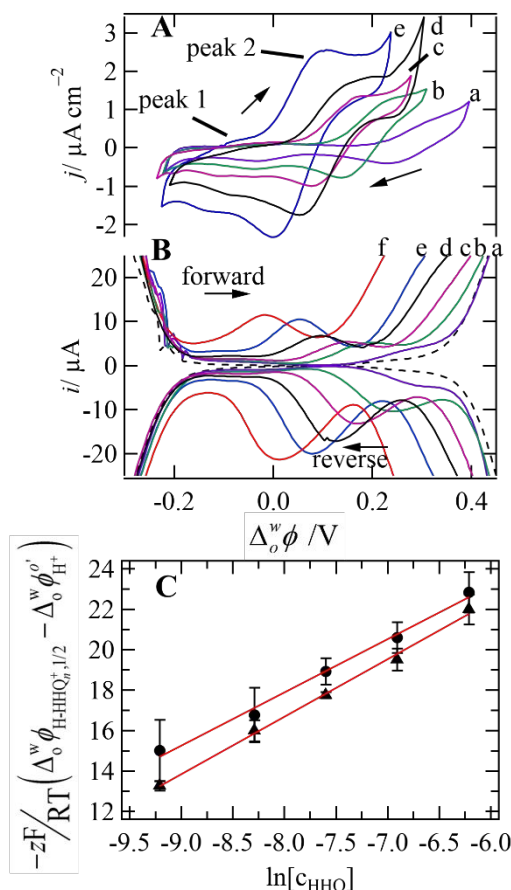
Figure 5: [A] CVs and [B] DPVs recorded using Cell 1 with X = [HHQ] = 10 \mu M - 2 mM (traces a-f); the black dashed curve in B is Cell 1 without HHQ added. See the main text for DPV parameters; CV parameters are the same as described for
