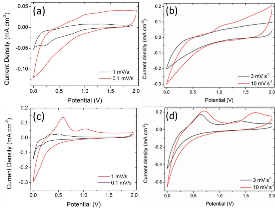
Figure 5. (a) CVs of p-type Si NWs at scan rates of 0.1 \text{ mV s}^{-1} and 1 \text{ mV s}^{-1} and (b) at scan rates of 3 \text{ mV s}^{-1} and 10 \text{ mV s}^{-1} . (c) CVs of n-type Si NWs at scan rates of 0.1 \text{ mV s}^{-1} and 1 \text{ mV s}^{-1} and (d) at scan rates of 3 \text{ mV s}^{-1} and 10 \text{ mV s}^{-1} .
