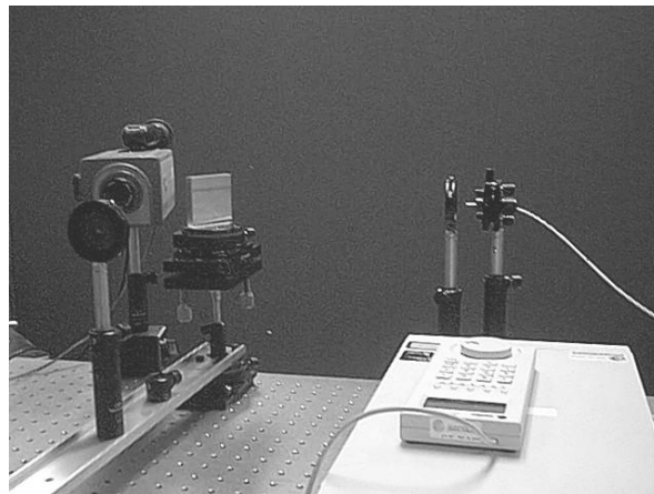
Fig. 2 Experimental setup to validate the theoretical angular scans obtainable from free-space W-MOS.
