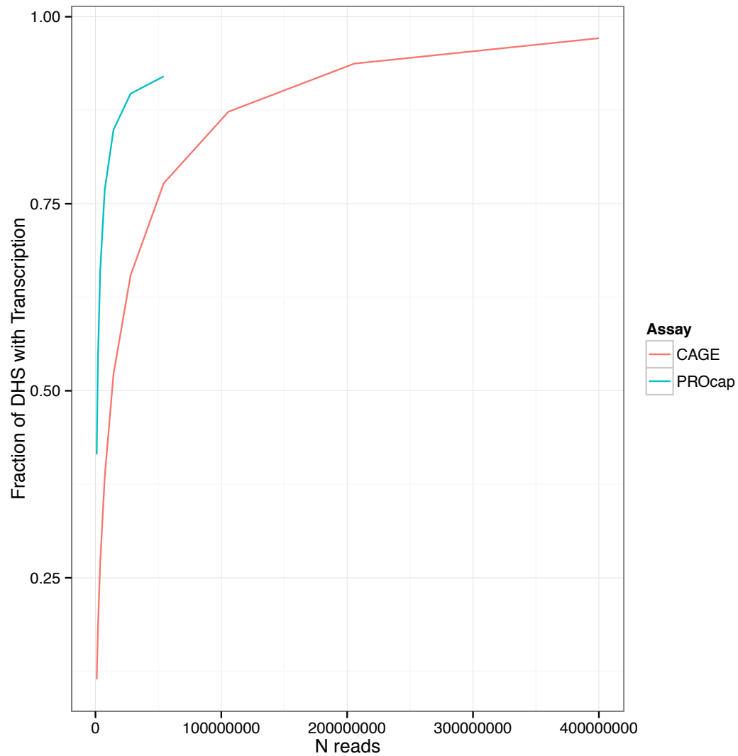
Figure 2.20 False positive rate vs threshold for expression assays – whole embryo
