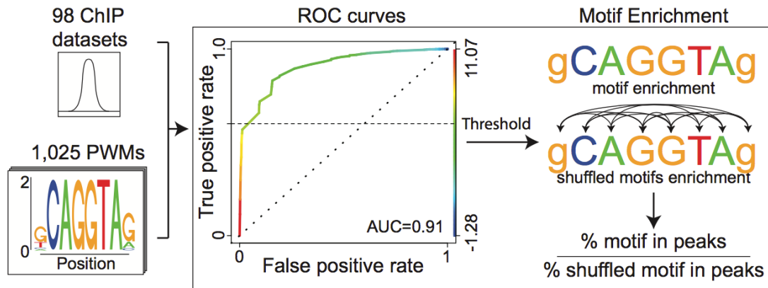
Figure 3.2 Diagram showing procedure for filtering TF motifs.
