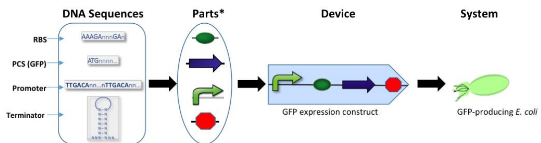
Figure 5. Schematic representation of an abstraction hierarchy. Here, a genetic component, (a gene, transcription factor or a promoter) is defined as a ‘part’; a collection of parts that together have a defined function = a ‘device’; a collection of devices integrate to create ‘systems’. (RBS: Ribosome binding site; PCS: Protein coding sequence).
