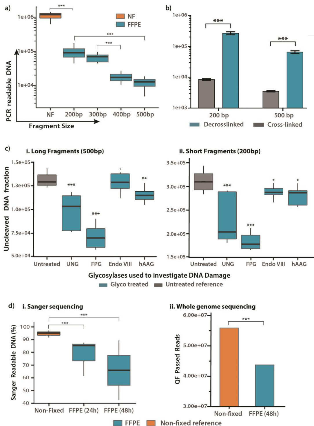
Figure 1. Analysis of DNA damage.
