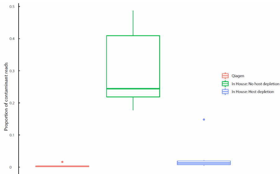
Figure 7. Proportion of reads lost due to environmental contamination introduced during processing.
