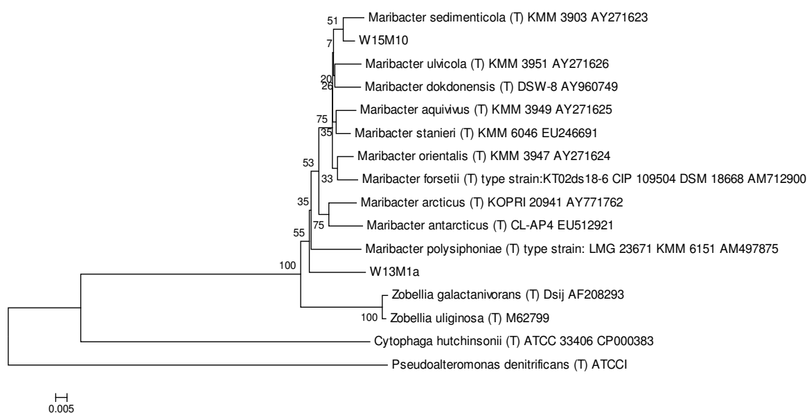
Figure 5.2: Minimum evolution bootstrap-consensus (1000 iterations) phylogenetic tree of Maribacter type strains, novel species and reference outgroup taxa.
