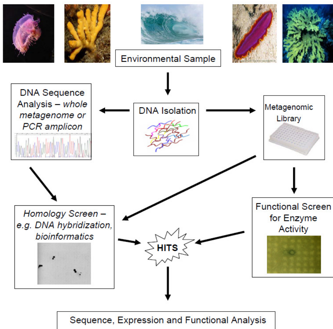
Figure 1.6: Sequence based and function based metagenomics (Kennedy et al. , 2010).
