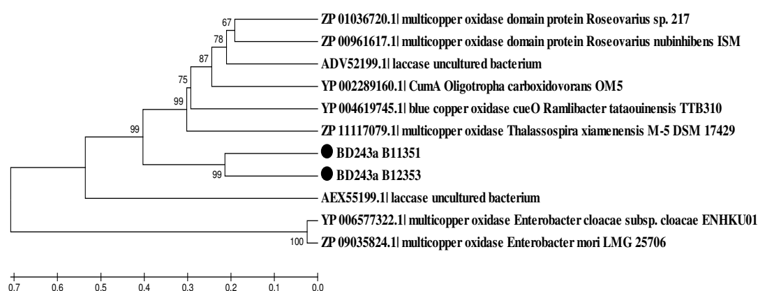
Figure 4.5: Bootstrap-consensus UPGMA tree showing the evolutionary relationships between the inferred amino acid sequences of partial putative laccase genes cloned from the metagenome of the marine sponge S. normani with the closest known protein sequences as determined by DELTA-BLAST. ‘●’ – denotes sponge derived sequences.
