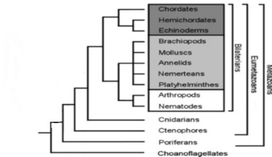
Figure 1.1: Phylogeny of metazoa, adapted from Degnan et al. , 2005.
