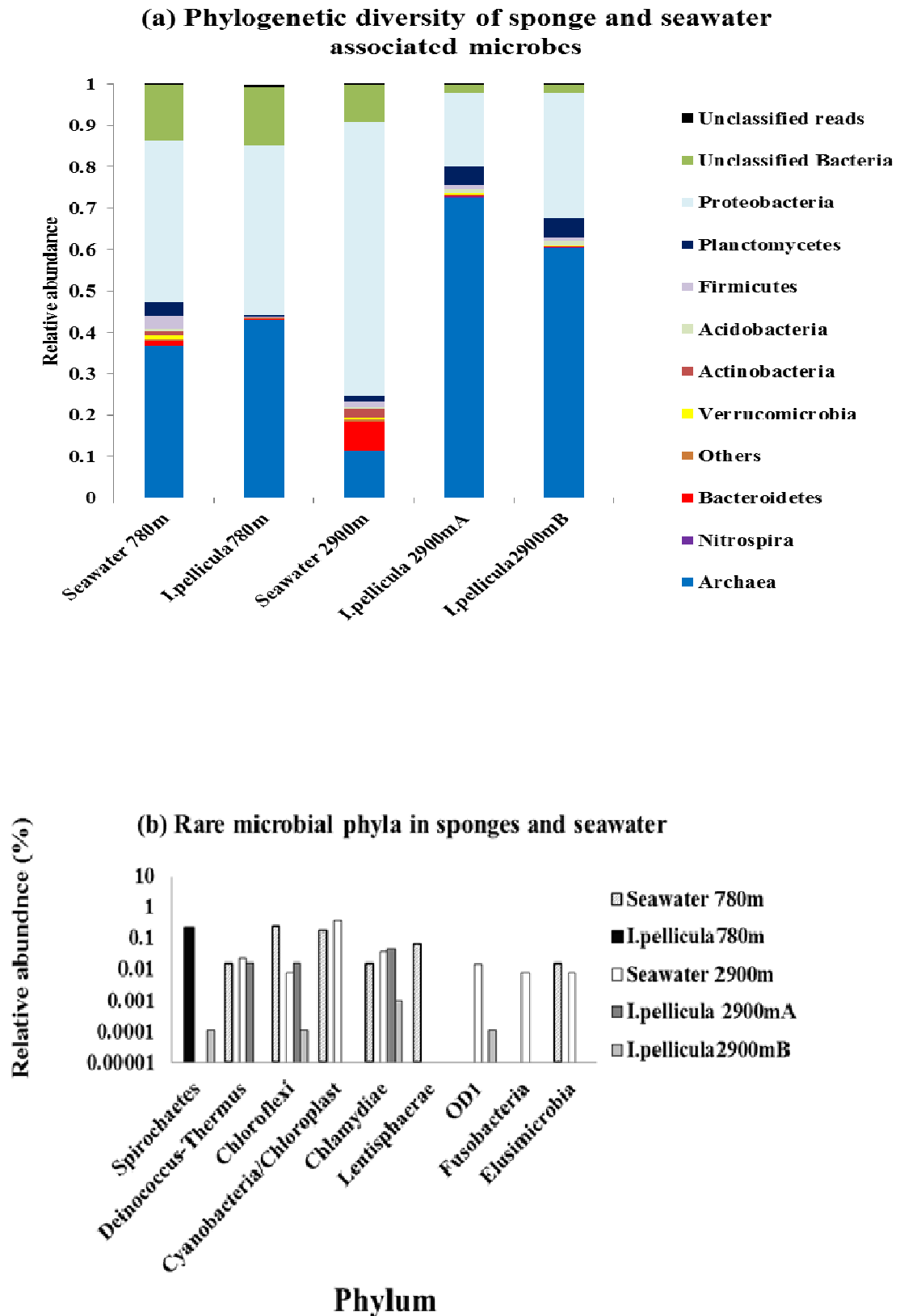
Figure 3.2: Phylogenetic affiliations of pyrosequencing reads assigned to (a) abundant microbial phyla. ‘Others’ in (a) represent (b) - rare microbial phyla associated with marine sponges and seawater.
