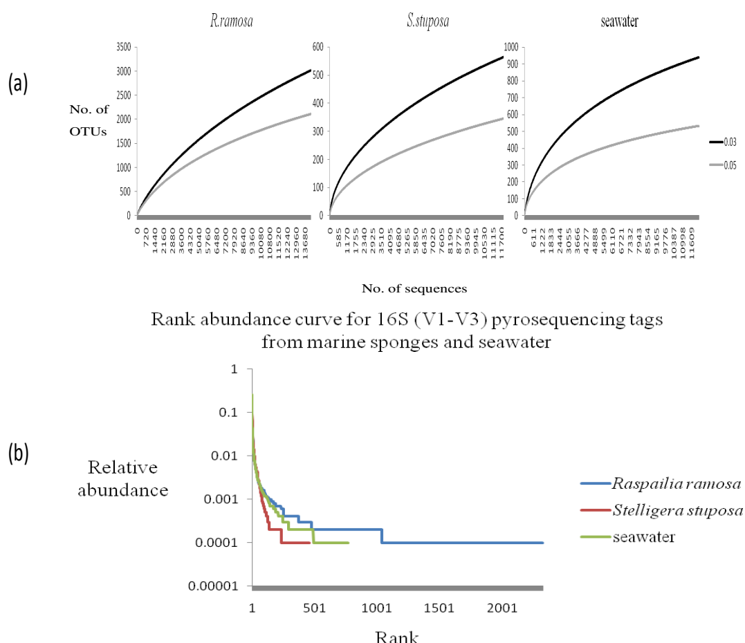
Figure 2.5: (a) Rarefaction curves and (b) rank abundance curves for marine sponge and seawater derived pyrosequencing reads.
