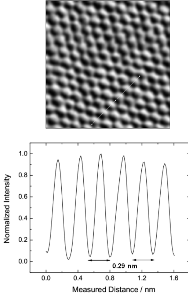
Fig. 3. (a) 3 \text{ nm} \times 3 \text{ nm} constant current STM image of the MoS 2 surface showing the (\sqrt{3}a \times \sqrt{3}a) hexagonal packing arrangement of the outermost S atoms of the basal (0001) plane of the S-Mo-S stacked compound. (b) The corresponding cross-sectional line scan profile where the repeat distances, as a function of the reduced interatomic S-S distance, a = 0.29 \text{ nm} , are also highlighted.
