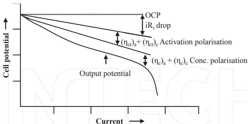
Figure 2. Cell potential as a function of current.
