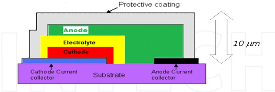
Figure 12. Typical lithium thin film microbattery cross sectional schematic.
