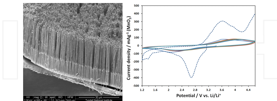
Figure 11. Free standing ramsdellite \text{MnO}_2 electrodeposited on Cu nanotubes in an AAO template following removal of the template.
