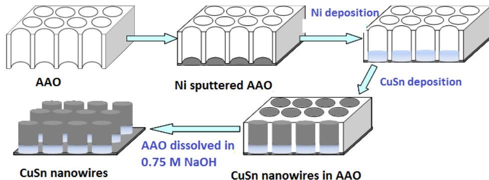
Figure 8. Schematic of templated CuSn nanowire fabrication process using Ni backed AAO.
