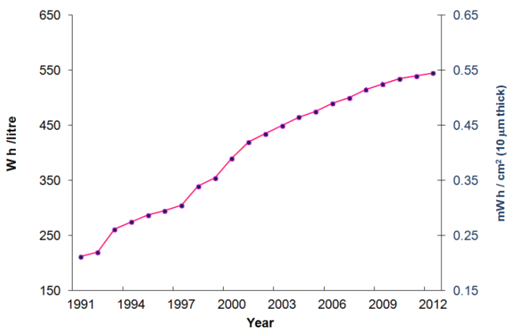
Figure 4. Li ion energy density improvements since 1991.
