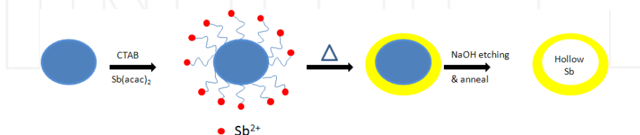
Figure 5. (a) Schematic illustration of the preparation of hollow Sb nanospheres from the CTAB (cetyltrimethylammoniumbromide) functionalised \text{SiO}_2 templates.[40]
