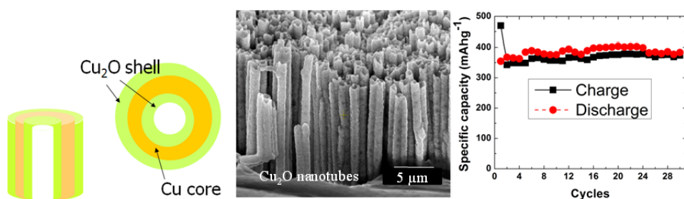
Figure 10. \text{Cu}_2\text{O} nanotubes for core/shell battery anode materials.
