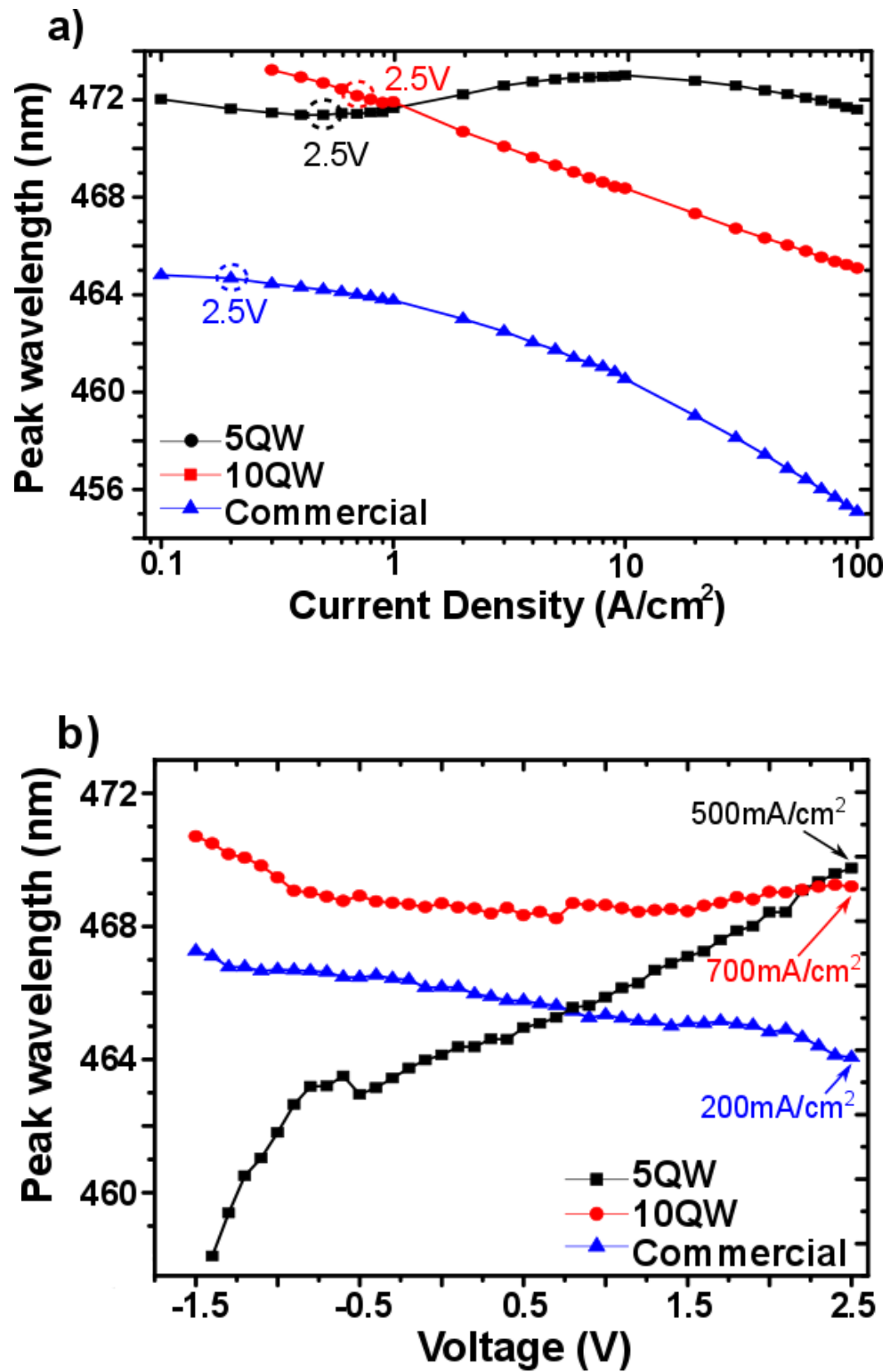
Figure 5.7: a) Peak wavelength versus current under electrical excitation, b) peak wavelength versus voltage under optical ( 200 \text{ W}/\text{cm}^2 ) and electrical excitation.
