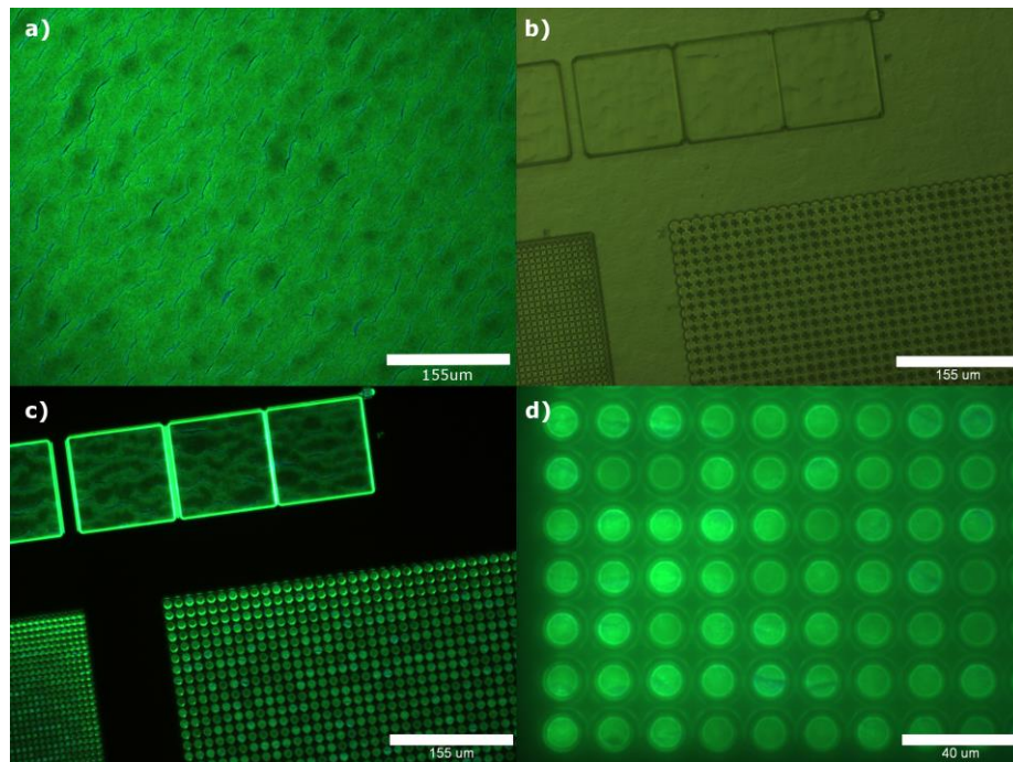
Figure 4.7: a) Fluorescence image of the spatial variation in a commercial green sample ( \sim 530\text{nm} ) before processing. b) Optical image of the same sample after patterning with small squared and circular contacts. c) Fluorescence image of the same areas as in b). d) Close-up of the circular contacts on the right hand side of c). Selected wavelength for excitation cut-off was 400\text{nm} .
