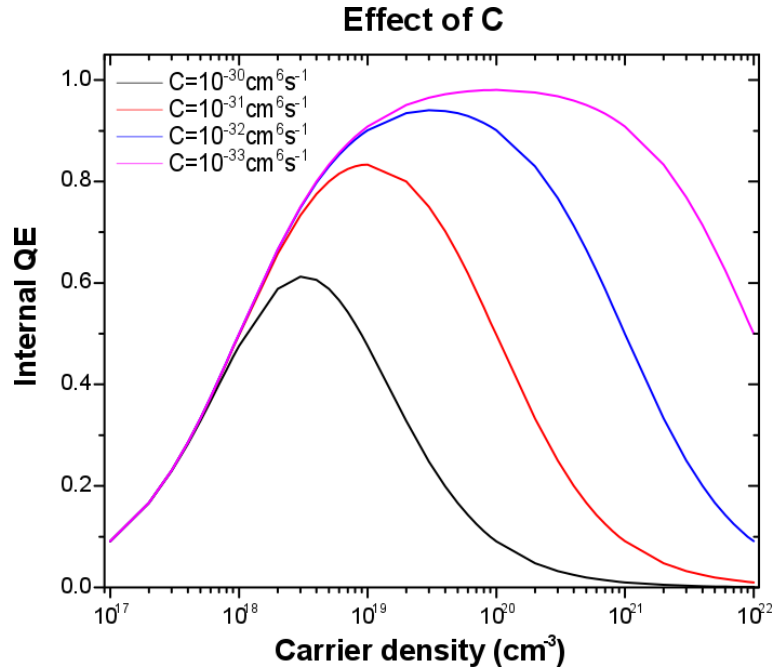
Figure 5.20: Calculated IQE values for different values of the Auger coefficient C . The A and B coefficients were held at A = 10^7 \text{ s}^{-1} [28] and B = 10^{-11} \text{ cm}^3 \text{ s}^{-1} [27].
