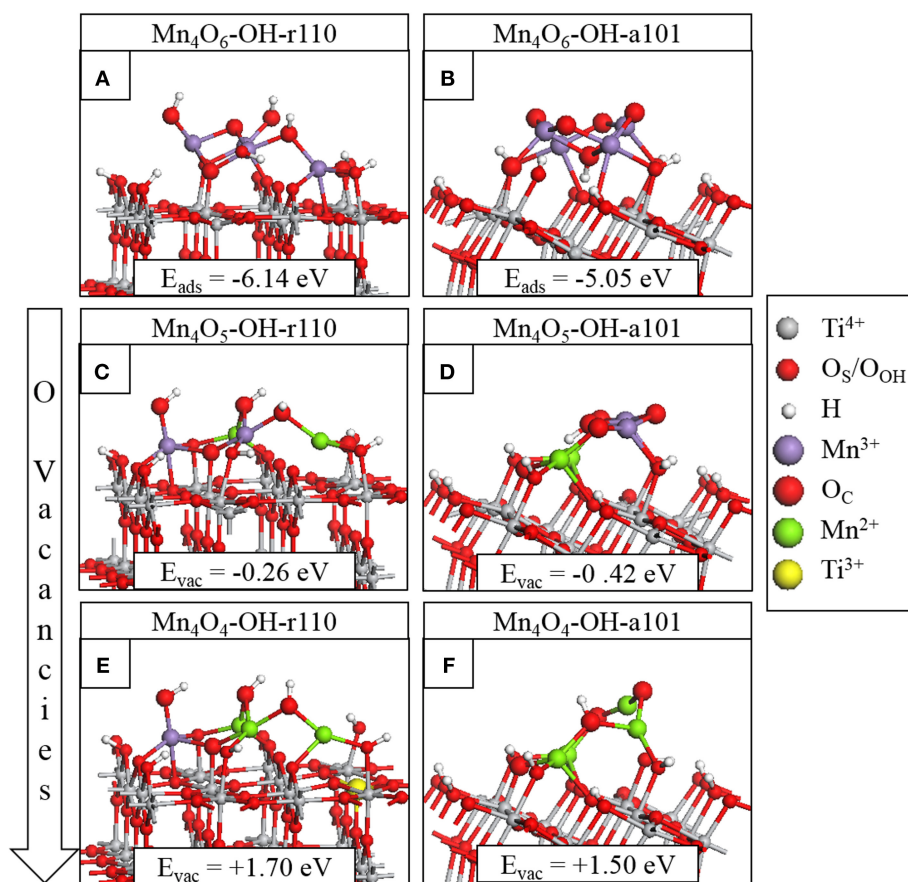
FIGURE 1 | Relaxed atomic structures of \text{Mn}_4\text{O}_x modifying the hydroxylated titania surfaces. The stoichiometric composites are shown in (A) for \text{Mn}_4\text{O}_6 -OH-r110 and (B) for \text{Mn}_4\text{O}_6 -OH-a101; the nanocluster adsorption energies are included in the inset. The atomic structures after formation of the most stable single \text{O}_V are shown in panels (C) for \text{Mn}_4\text{O}_5 -OH-r110 and (D) for \text{Mn}_4\text{O}_5 -OH-a101. The atomic structures of the most stable composites with two \text{O}_V are shown in panels (E) for \text{Mn}_4\text{O}_4 -OH-r110 and (F) for \text{Mn}_4\text{O}_4 -OH-a101. The energy costs to produce \text{O}_V are included and computed relative to the structure with one less \text{O}_V . Atomic species and oxidation states are indicated by the colors in the legend on the right hand side.
