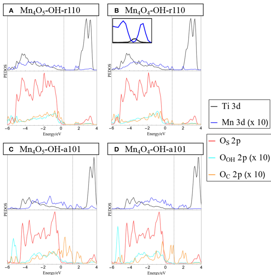
FIGURE 2 | Projected electronic density of states (PEDOS) plots for (A) \text{Mn}_4\text{O}_5 -, and (B) \text{Mn}_4\text{O}_4 -OH-r110 and (C) \text{Mn}_4\text{O}_5 -, and (D) \text{Mn}_4\text{O}_4 -OH-a101. The computed valence band max is set to 0 eV and the Fermi energy is indicated with a dashed line. The top half of each panel displays Ti and Mn 3d derived states. The bottom halves of the panels show contributions to the DOS from oxygen 2p states of the surface ( \text{O}_\text{C} ), surface bound hydroxyls ( \text{O}_\text{OH} ) and nanocluster ( \text{O}_\text{C} ). Inset in panel (B) shows the mid-gap occupied Ti 3d states in the range [0 eV, 1 eV].
