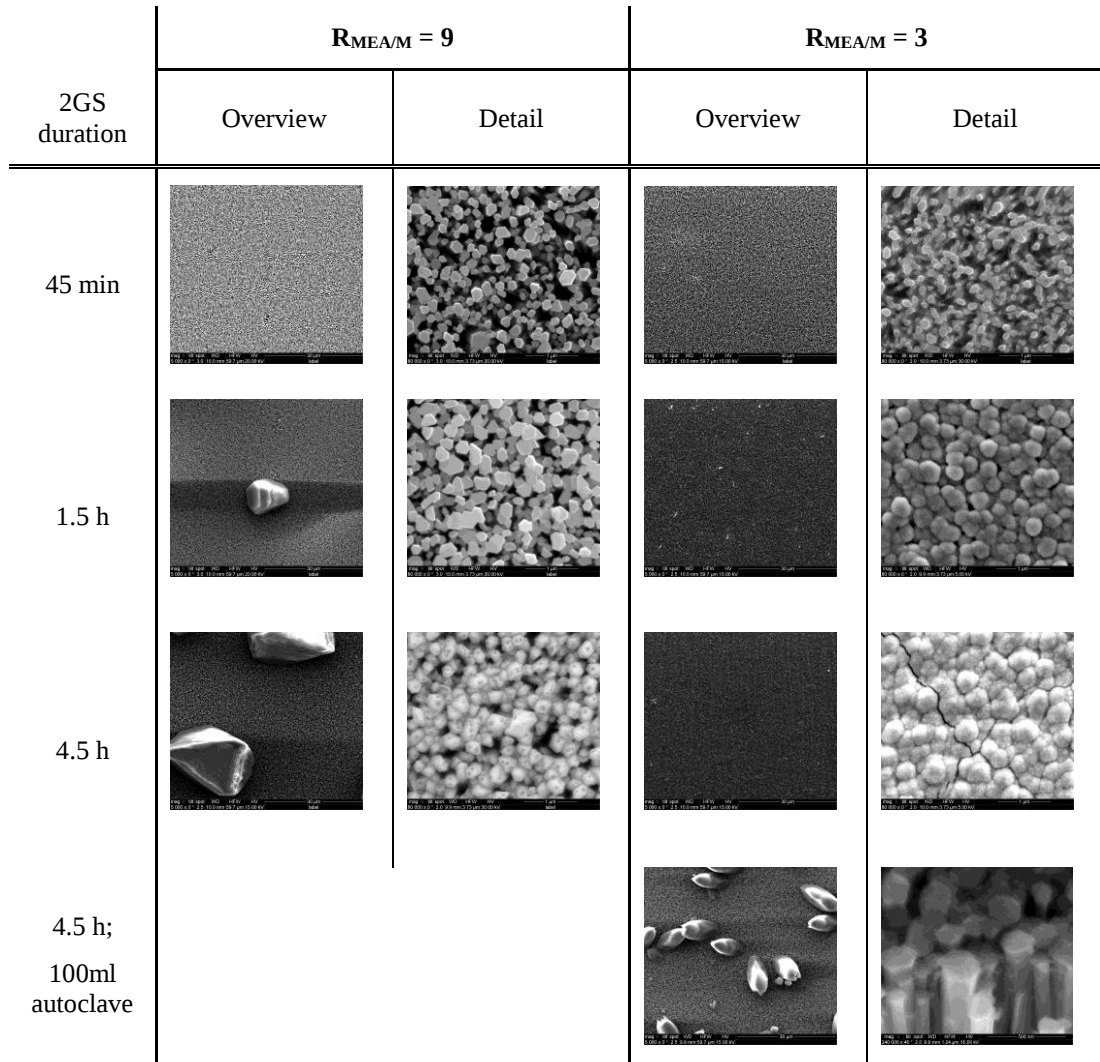
Figure A4- 2 SEM top-view images of samples subjected to a second growth stage (2GS; 150 °C). The samples were grown from varying MEA concentrations ( R_{\text{MEA/M}} = 9 or 3) and the duration of the 2GS was 45 min, 1.5 h or 4.5 h. Furthermore, one sample was grown in a 100 ml autoclave (all other growths in 200 ml autoclave). Overview and detail images were taken at a magnification of x5k and x80k, respectively (detail of 4.5 h in 100 ml autoclave at x240k).
