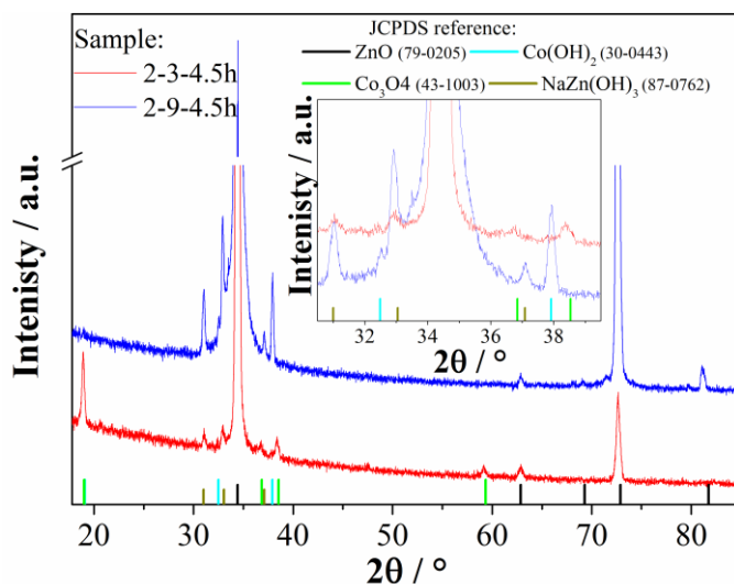
Figure 6-5. XRD spectra of decorated ZnO:Co NR arrays grown from R_{\text{MEA/M}} = 3 or 9. The duration during the second growth stage was 4.5 h. The inset magnifies the range 2\theta = 30 - 40^\circ .
