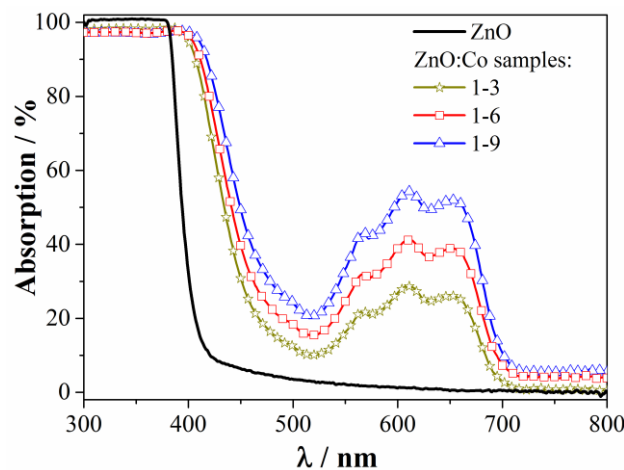
Figure 6-3. UV-Vis absorption spectra of ZnO:Co NR arrays grown at 90 °C for 16 h from solutions of R_{\text{MEA}/M} = 3, 6 or 9.
