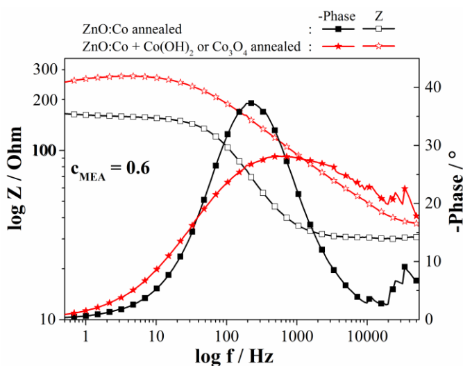
Figure A4- 4. Bode plots of annealed decorated/undecorated ZnO:Co NR arrays grown from c_{\text{MEA}} = 0.6 ( R_{\text{MEA/M}} = 9 ). Annealing was carried out at 400 °C for 3h – please note that \text{Co(OH)}_2 (decoration of the as-grown sample) was thus converted to \text{Co}_3\text{O}_4 .
