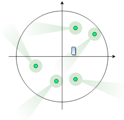
Fig. 5. Snapshot of the indoor mmWave hotspot layout with five transmitters. The reference receiver location is marked with a rectangle and the transmitter locations are the small circles. The direction of transmissions for all the transmitters is illustrated as rotation of the 2D- projection of the cone bulb antenna gain model in (4).
