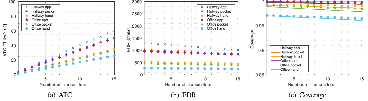
Fig. 6. Impact of the number of transmitters n_{TX} . Where n_{TX} = 1 represents the scenario with a single serving transmitter and no other transmitters within a given area. Other network settings are: \omega_{TX} = 30^\circ , r_0 = 1 m, and p_{LOS} = 0.5 .
