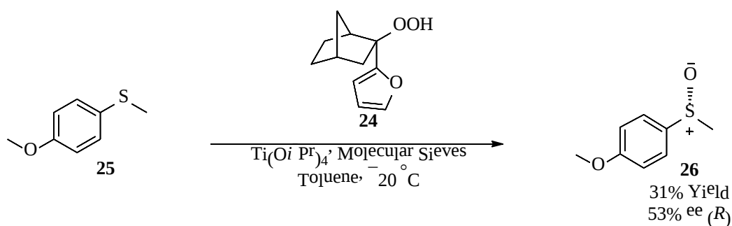
Scheme 5 Chiral Hydroperoxides
