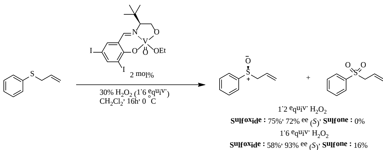
Scheme 17 Asymmetric Oxidation of Allyl Phenyl Sulfide using a Vanadium Complex
