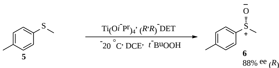
Scheme 2 Modena Oxidation
