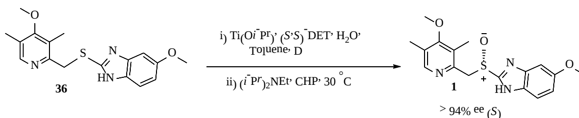
Scheme 9 Synthesis of Esomeprazole using a modified Kagan Procedure
