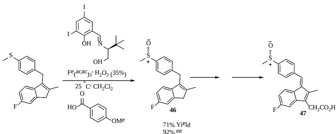
Scheme 25 Asymmetric Synthesis of Sulindac using an Iron Complex
