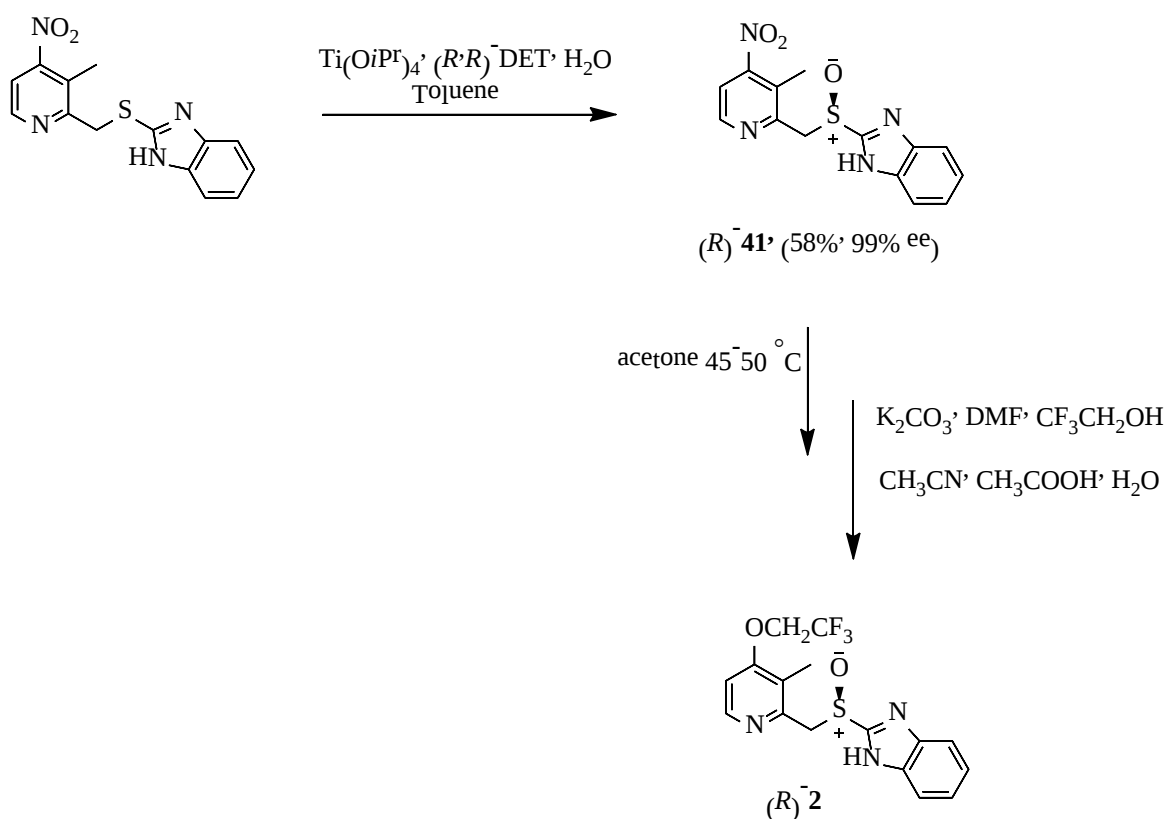
Scheme 11 Asymmetric Synthesis of Dextansoprazole using a Titanium Complex
