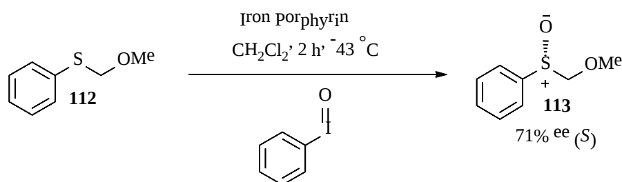
Scheme 22 Iron Porphyrin-Catalyzed Asymmetric Oxidation of Sulfides
