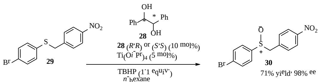
Scheme 6 Chiral Diol in Titanium-mediated Oxidation
