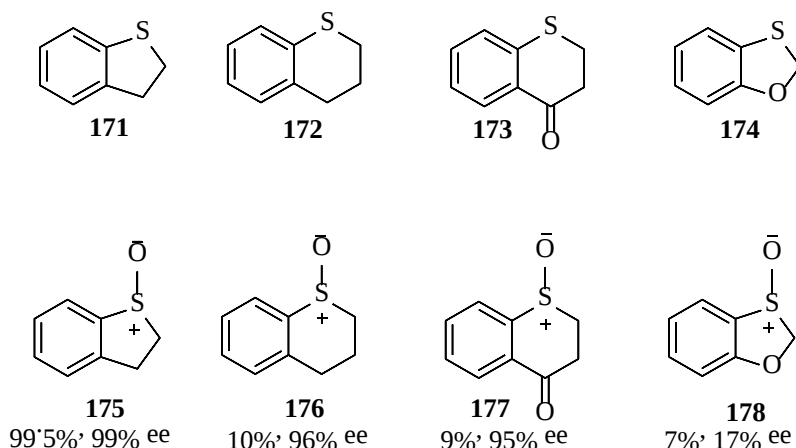
Scheme 33 Asymmetric Sulfoxidation using a CPO Enzyme
