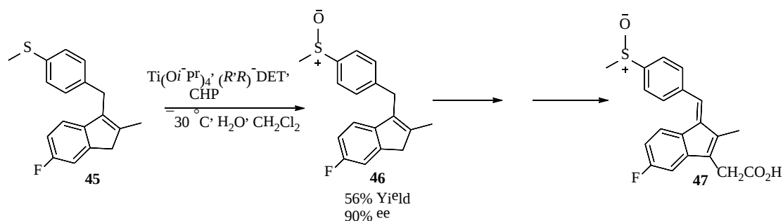
Scheme 12 Asymmetric Synthesis of Sulindac using a Titanium Complex
