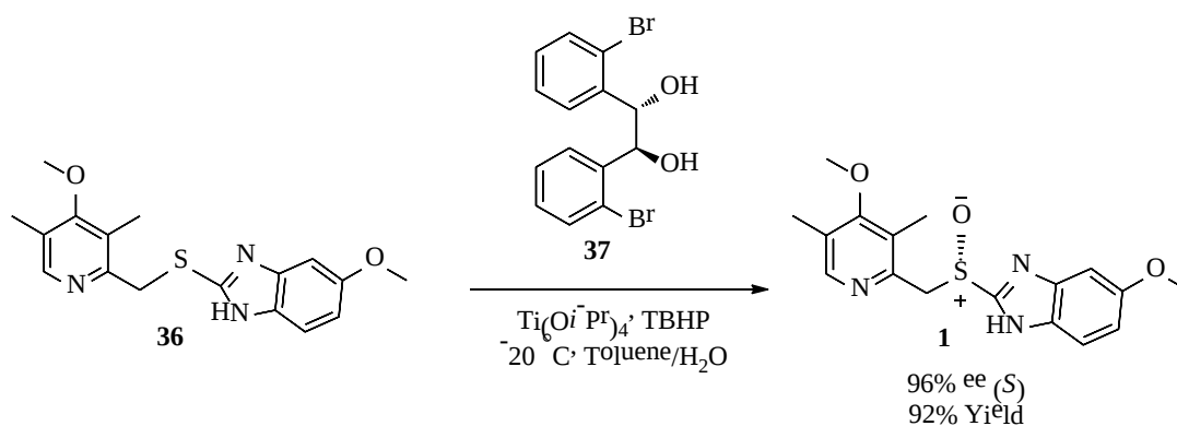
Scheme 10 Synthesis of Esomeprazole using Brominated Aromatic Diol
