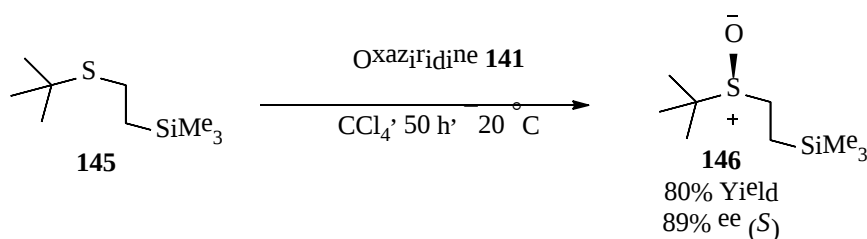
Scheme 29 Asymmetric Sulfoxidation of Sterically Bulky Sulfides using a Chiral Oxaziridine
