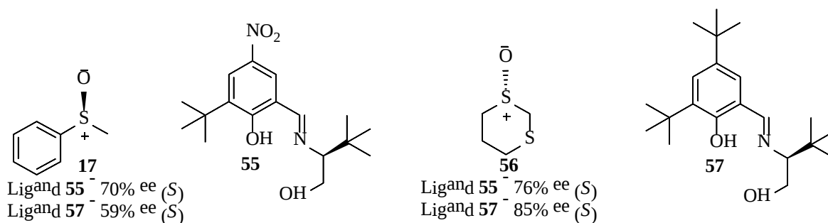
Scheme 14 Optimum Ligand is Substrate Specific
