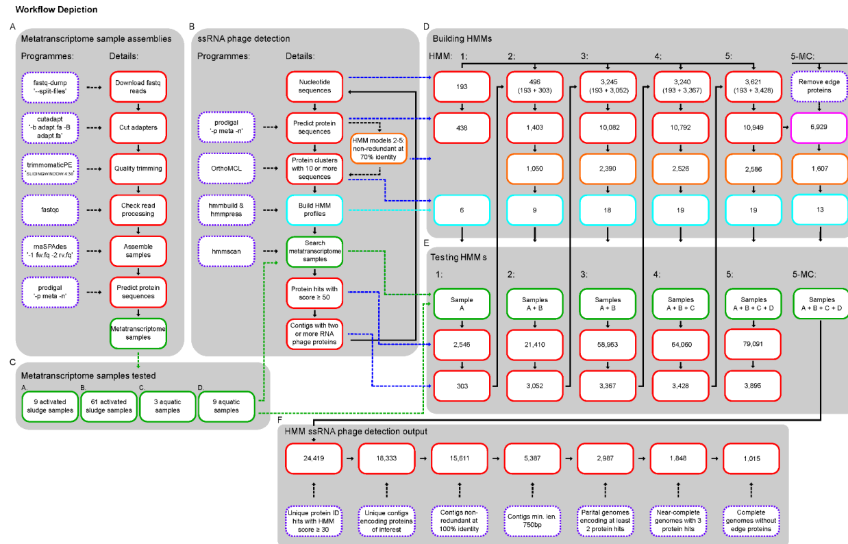
Figure 1. Workflow depiction of the study pipeline, outlining: (A) metatranscriptome sample assemblies, (B) the detection of +ssRNA phages, (C) samples tested, and the breakdown of the (D) building, (E) testing, and (F) output of the HMM iterations.
