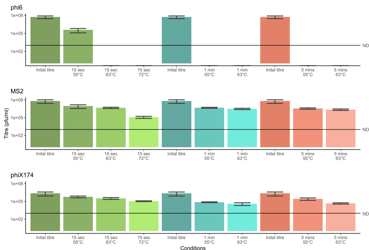
Figure 6. Effect of different time-temperature conditions on the phages phi6, MS2 and phiX174. The titre of phi6 dropped by two logs following 55°C at 15 seconds and was undetectable at every other time-temperature combination. In comparison, MS2 and phiX174 titres dropped in a time- and temperature-dependent manner – as the time and temperature increased, the titre of the phage decreased. The error bars indicate \pm standard deviation. (ND = not detectable; level of detection was >10^3 pfu/ml).
