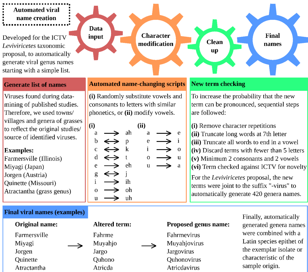
Figure 1. Graphical overview simplifying the automated name creation strategy employed to generate genus names for the Leviviricetes taxonomic proposal recently ratified by the ICTV.
