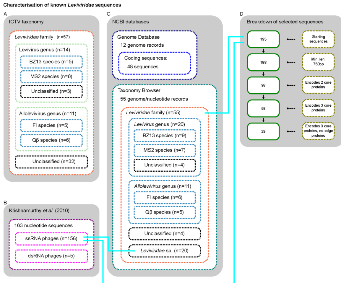
Figure 2. Workflow depiction of known +ssRNA phage sequences, outlining: (A) ICTV taxonomy, (B) Krishnamurthy et al. (2016), (C) NCBI Genome and Taxonomy database available sequences, and (D) the breakdown of the identifiable +ssRNA phage sequences used in this study.
