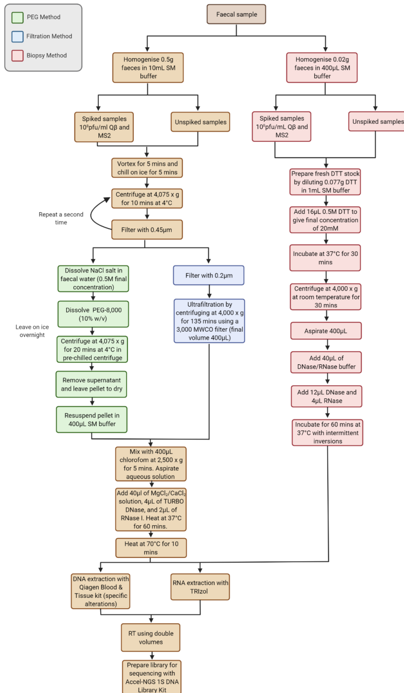
Figure 1. Overview of the different extraction methods used in this study. A common faecal sample was used in all three methods, with both a spiked (a final titre of 10 8 pfu/ml of MS2 and Qbeta) and unspiked fraction, to enable direct comparison across the results.
