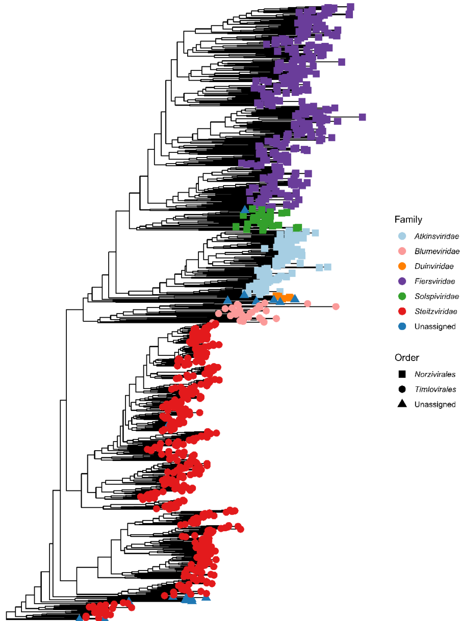
Figure 2. Hidden Markov model (HMM) predictions of leviviricetes taxonomy. While expanding and restructuring positive-sense single-stranded RNA (+ssRNA) viruses, nine genera could not be assigned with confidence to a family or an order, as the RNA-directed RNA polymerase (RdRP), and coat protein (CP) genome-encoded combinations did not adhere to established combinations. Additionally, there were ten instances (out of 882 species representative sequences) for which the hidden Markov model (HMM) predicted taxonomy of
