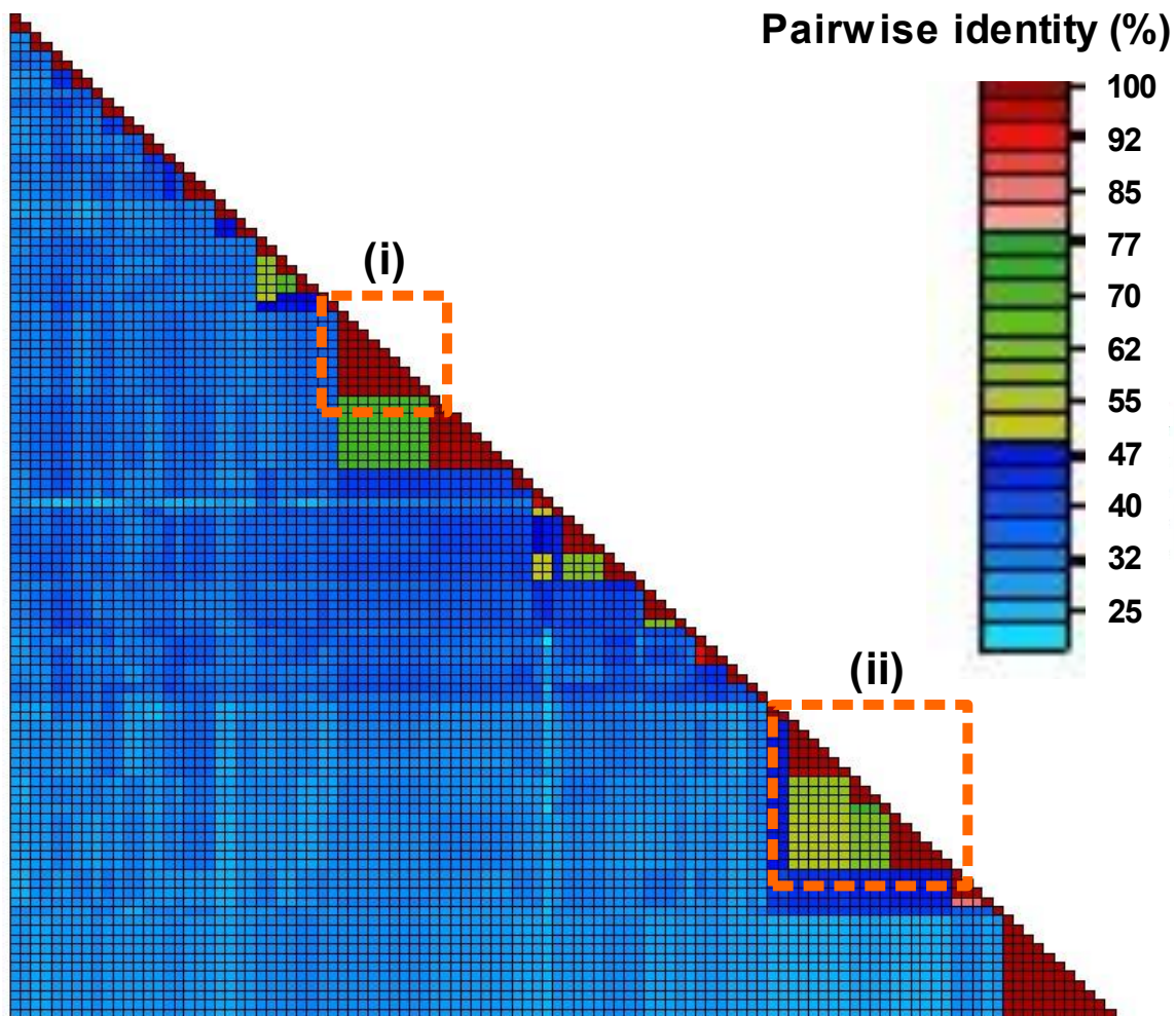
Figure 3. Examples of Leviviricetes genus and species demarcation cutoffs of 50% and 80%, respectively, applied to pairwise RNA-directed RNA polymerase (RdRP) amino-acid sequence comparisons for members of norziviral Atkinsviridae . Inset (i) shows a distinct species clustering (red coloring), whereas inset (ii) shows three species represented by multiple sequences, and a species representing a single sequence, clustered into a genus (yellow-green coloring). Pairwise comparisons in shades of blue do not meet the set genus or species clustering criteria.
