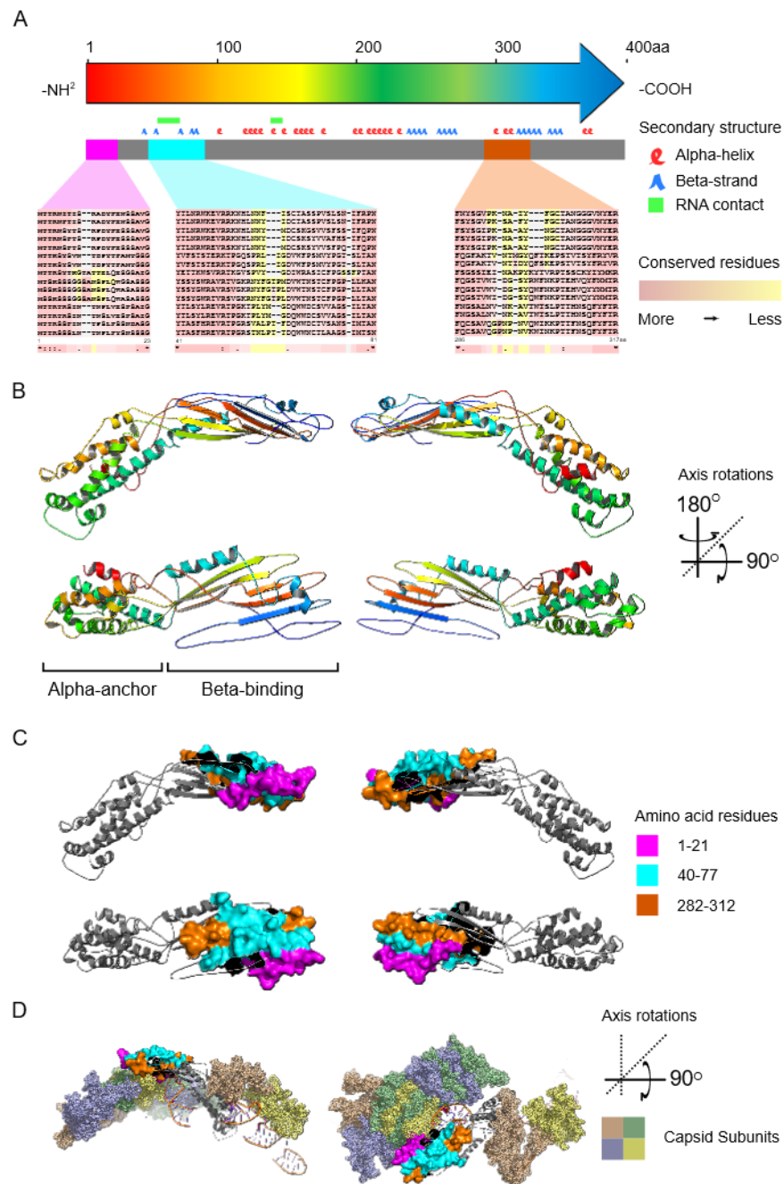
Figure 10. Structural investigation of +ssRNA phage-host interactions. (A) A cartoon representation of the MP of +ssRNA phages, with amino acid (aa) length, predicted secondary structure, RNA contact sites, and variable regions highlighted. (B) The MP has an alpha-helical
