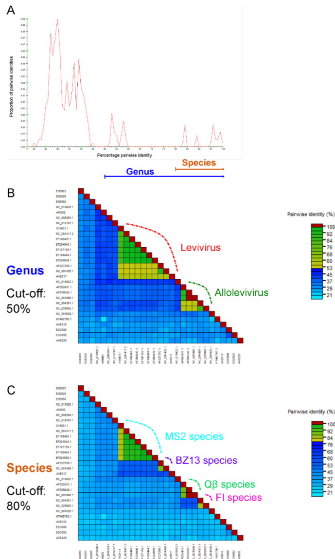
Figure 6. Taxonomic cut-off values for +ssRNA phage genera and species. (A) Pairwise RdRP amino acid identity (PAAI) comparisons. Four currently recognised species had PAAI \geq 80\% , while the two genera had PAAI \geq 50\% . Visualisation of PAAI at (B) genera level, and (C) species level with taxonomic groups depicted.
