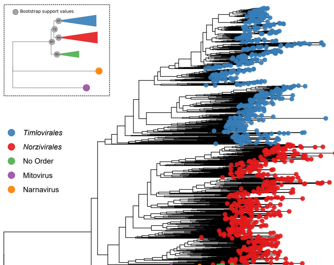
Figure 3. Phylogenetic analysis of bacterial positive-sense single-stranded (+ssRNA) virus RNA-directed RNA polymerase (RdRP) protein sequences. Mitovirids and narnavirids were used to root the bacterial +ssRNA viral RdRP tree, generated using maximum-likelihood-based phylogenetic reconstruction in IQ-TREE with the VT+F+R10 model and 1,000 bootstrap replicates. RdRP sequences used to generate the tree were made non-redundant at 95% BLASTp identity across 95% of coverage length. The image inset, top left, shows a simplified version of the phylogenetic tree with bootstrap support values for the major branches. Sequences without specific corresponding coat protein and RdRP sequences, and which were not assigned order and familial taxonomic ranks (see text), are highlighted as “No Order”. RdRP phylogeny is the demarcation criteria proposed for establishing the Norzivirales and Timlovirales +ssRNA viral orders.
