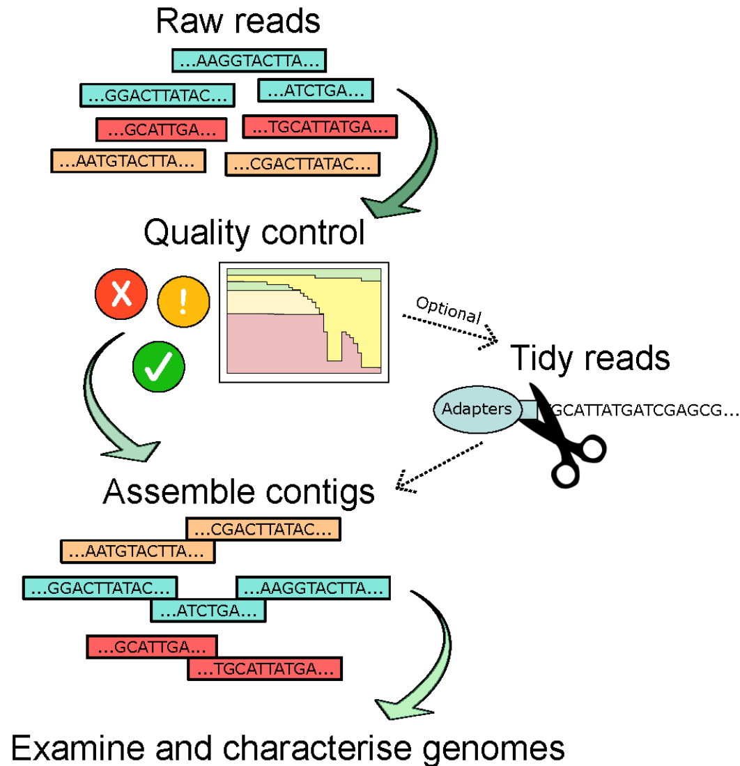
Figure 3. Overview of genome assembly in as part of the bioinformatic pipeline used for virome/phageome analyses.
