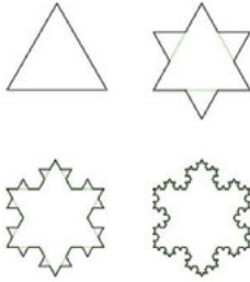
Figure 1: The Koch Snowflake
