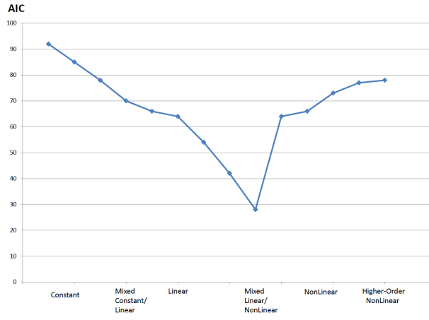
Fig. 6. Comparison of AIC scores for extended models
