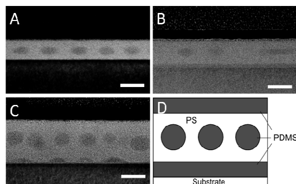
Figure 9. Various (A – C) images of PS-b-PDMS on substrates of different surface chemical functionality. A schematic (D) describes the arrangement shown in C. See text for details. Scale bar is 40 nm in all cases.
