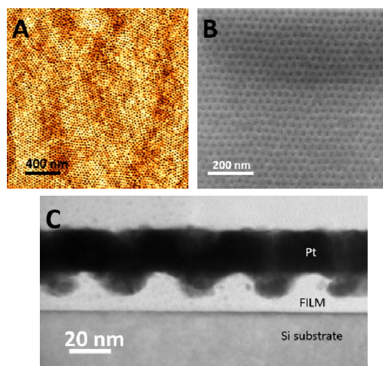
Figure 5. AFM (A), SEM (B) and TEM (C) images of PS- b -PEO. See text for details. In the TEM image, Pt is an e-beam layer deposited during cross-section FIB preparation to protect the mechanical weak polymer layer.
