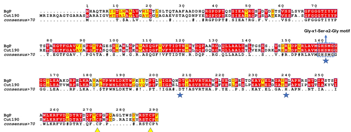
FIGURE 2 | Amino acid sequence structural alignment of BgP and Cut190 generated with T-COFFEE Expresso and rendered using ESPrnt 3.0. Cut190 was indicated as a suitable structural homolog for BgP by the Phyre2 server. Amino acid residues shaded in red represent the ones strictly conserved between BgP and Cut190, while residues highlighted in yellow depict areas with an average level of homology. Catalytic triad residues are marked with a blue star, and disulfide bond cysteines are marked with a yellow triangle. The pentapeptide Gly-x1-Ser-x2-Gly serine hydrolase motif is outlined with a blue box.
