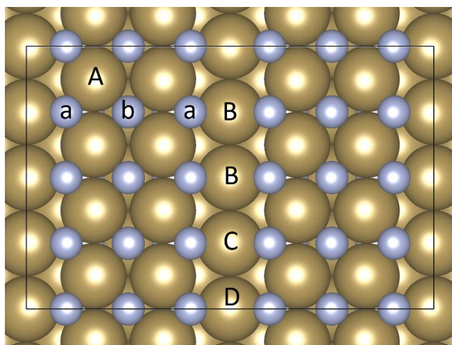
Figure 7.1. Top view of the \epsilon -TaN (110) surface. Colour scheme is: Ta = brown and N = blue.
