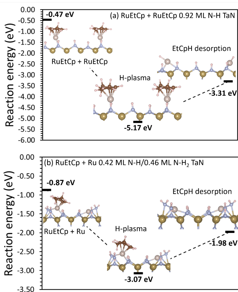
Figure 8.18 Reaction pathway of 'H radical treated (a) (RuEtCp) 2 0.92 ML N-H \epsilon -TaN (110) and (b) RuEtCp & Ru 0.42 ML N-H/0.46 ML N-H 2 \epsilon -TaN (110). Colour scheme is the same as in Figure 8.1.
