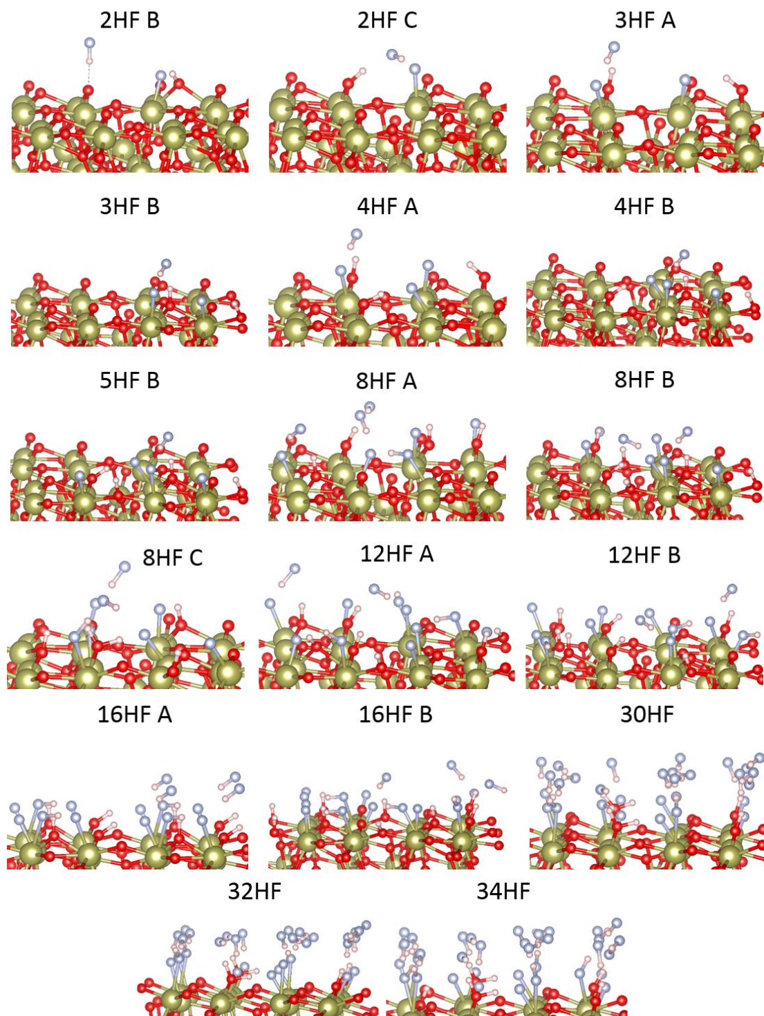
Figure A 1: Relaxed geometries for different HF coverages of \text{HfO}_2 where a mixture of molecular and dissociative adsorption of HF is observed. Colour scheme: Hf = gold, O = red and H = white.
