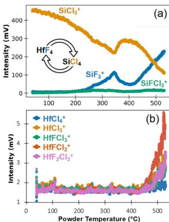
Figure 2.4 Temperature dependence of the ligand exchange reaction between \text{SiCl}_4 and \text{HfF}_4 powder. Taken from ref. 81 .
