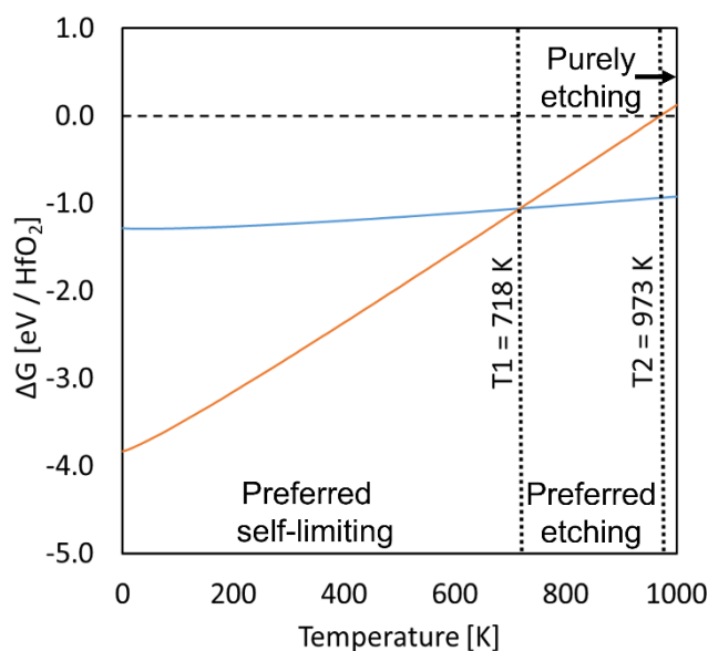
Figure 5.1: Free energy profile for the SE1 (blue) and SL1 (orange) reactions of aHfO 2 from 0 to 1000 K at the pressures given in the text. T1 is where the SL and SE reactions cross over for the 8O/16F model, and T2 is where spontaneous etching is preferred.
