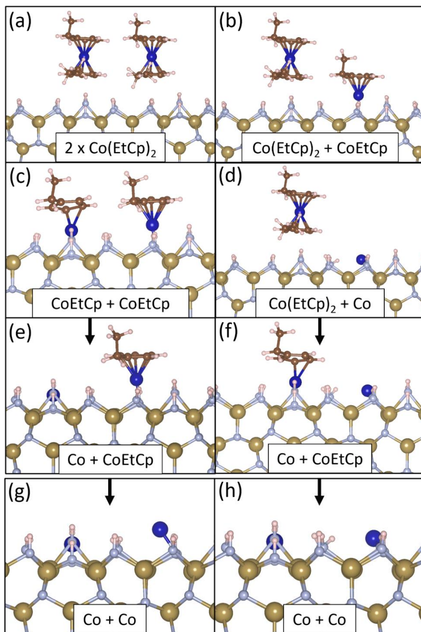
Figure 8.45 Geometries of two \text{Co}(\text{EtCp})_2 adsorbed on the 0.5 \text{ ML N-H}/0.5 \text{ ML N-H}_2 \epsilon\text{-TaN (110)} surface. Colour scheme is the same as in Figure 8.27.
