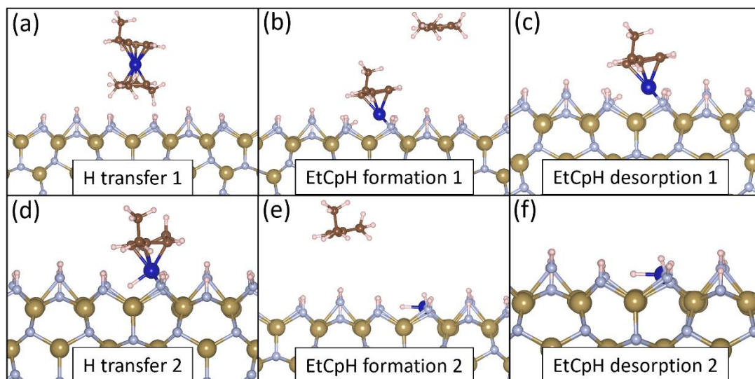
Figure 8.41. Geometries of the individual reaction pathway steps for the upright interaction mode of \text{Co}(\text{EtCp})_2 on 0.5 ML N-H/0.5 ML N-H 2 \epsilon -TaN (110). Colour scheme is the same as in Figure 8.27.
