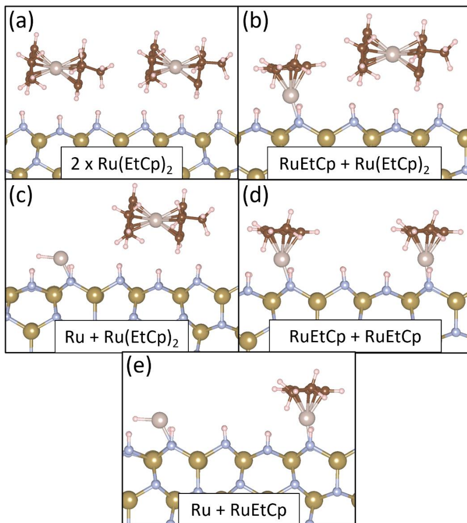
Figure 8.15 Geometries of two \text{Ru}(\text{EtCp})_2 on the 1 ML N-H \epsilon -TaN (110) surface. Colour scheme is the same as in Figure 8.1.
