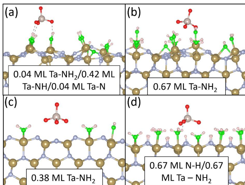
Figure A 6. RuO 4 adsorption at NH x -terminated TaN surfaces. Colour scheme is Ta = brown, N = light blue & green, H = pink, O = red and Ru = grey.
