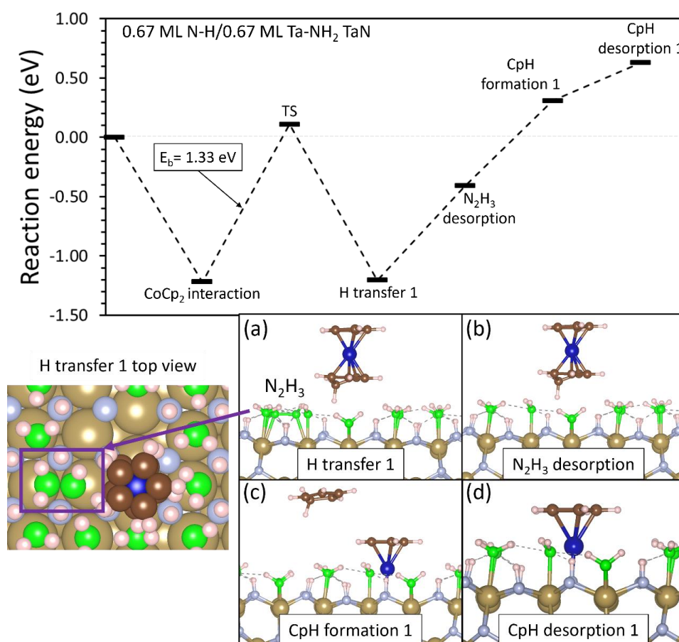
Figure 8.31: \text{CoCp}_2 reaction pathway on 0.67 ML N-H/0.67 ML Ta-NH 2 \epsilon -TaN (110) surface with the geometries shown. Colour scheme is the same as in Figure 8.27
