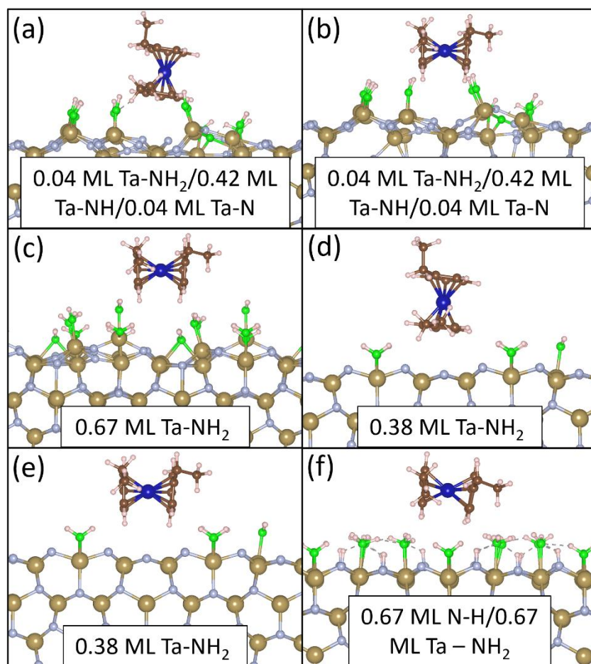
Figure A 9. Co(EtCp) 2 adsorption at NH x -terminated TaN surfaces. Colour scheme is the same as in Figure A 8.
