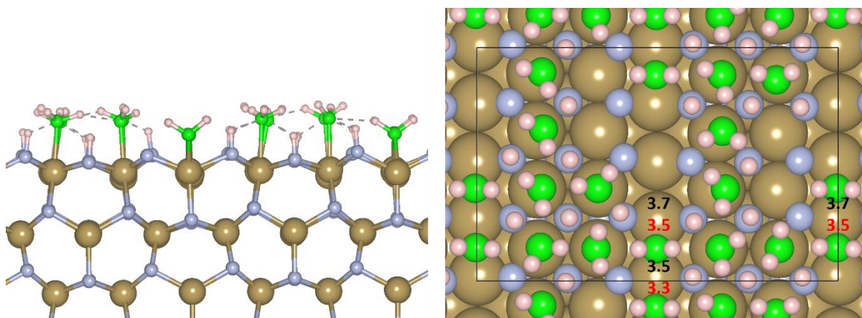
Figure 7.12: Side and top view of 0.67 ML N-H/0.67 ML Ta-NH 2 with computed Bader charge for Ta c included. (red = Ta charge after NH 2 adsorption and black = Ta charge for bare \epsilon -TaN (110)). Colour scheme is the same as in Figure 7.3.
