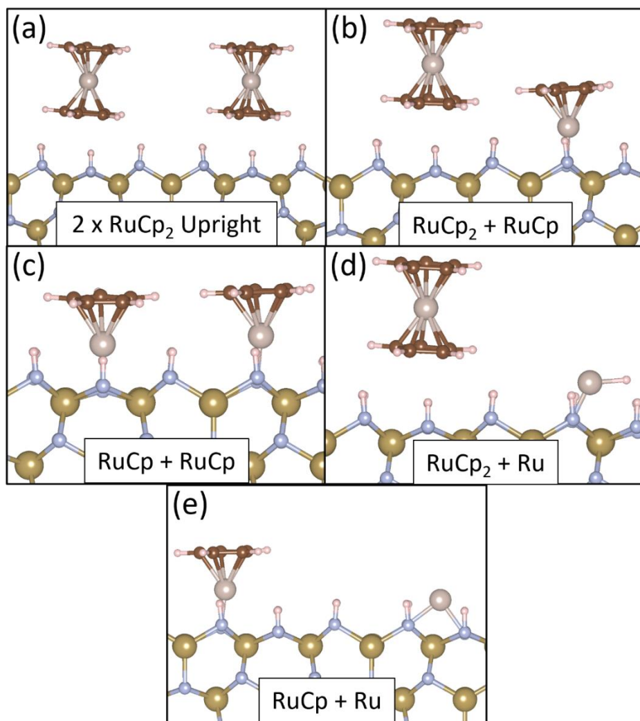
Figure 8.6. Geometries of the reaction pathway of two \text{RuCp}_2 precursors on 1 ML N-H \epsilon -TaN (110) surface for the upright interaction mode reaction pathway shown in panel (a) in Figure 8.5. Colour scheme is the same as in Figure 8.1.
