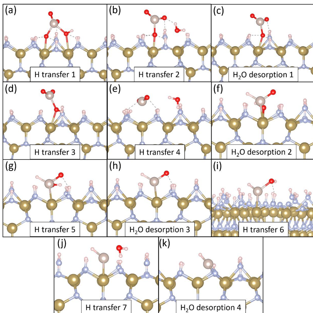
Figure 8.22. Geometries of the individual reaction pathway steps for RuO 4 on 0.5 ML N-H/0.5 ML N-H 2 \epsilon -TaN (110). Colour scheme is the same as in Figure 8.19.
