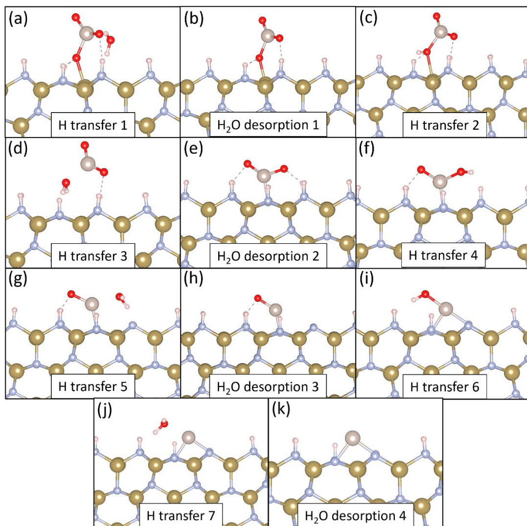
Figure 8.21. Geometries of the individual reaction pathway steps for \text{RuO}_4 on 1 ML N-H \epsilon -TaN (110). Colour scheme is the same as in Figure 8.19.
