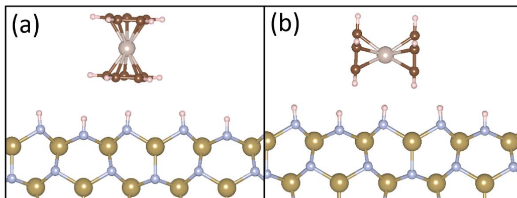
Figure 8.1. RuCp 2 interaction on 1 ML N-H terminated \epsilon -TaN (110) surface. (a) Upright interaction mode and (b) horizontal interaction mode.
