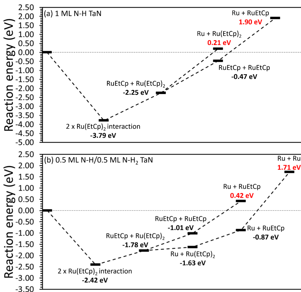
Figure 8.14 Reaction pathway for two Ru(EtCp) 2 precursors on (a) 1 ML N-H \epsilon -TaN (110) surface and (b) 0.5 ML N-H/0.5 ML N-H 2 \epsilon -TaN (110) surface.
