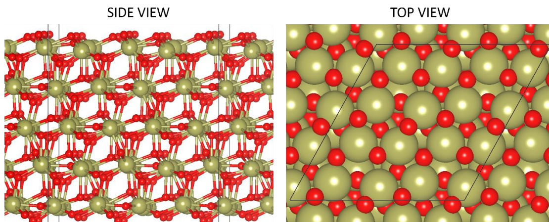
Figure 3.4: Side view and top view of orthorhombic (111) surface supercell of \text{HfO}_2 . Colour scheme is the same as in Figure 3.2.
