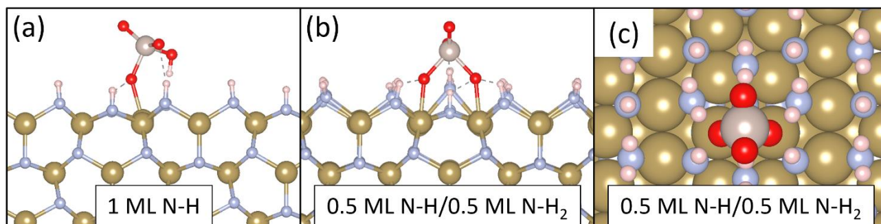
Figure 8.19. RuO 4 adsorption on (a) 1 ML N-H and (b) 0.5 ML N-H/0.5 ML N-H 2 \epsilon -TaN (110) surfaces. (c) Top view of RuO 4 on 0.5 ML N-H/0.5 ML N-H 2 \epsilon -TaN (110). Colour scheme is Ta = brown, N = light blue, H = pink, O = red and Ru = grey.
