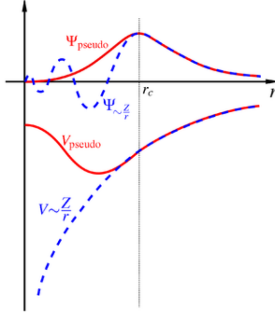
Figure 3.1: Graph illustrating the pseudopotential methodology where the pseudopotential replaces the real potential for \vec{r} < \vec{r}_c to reduce the number of basis set functions needed to describe the wavefunction.
