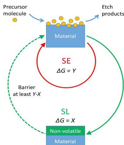
Figure 3.12: Schematic representation of the relationship between continuous spontaneous etch (SE, red) and self-limiting (SL, green) processes. \Delta G represents the reaction free energy. 57
