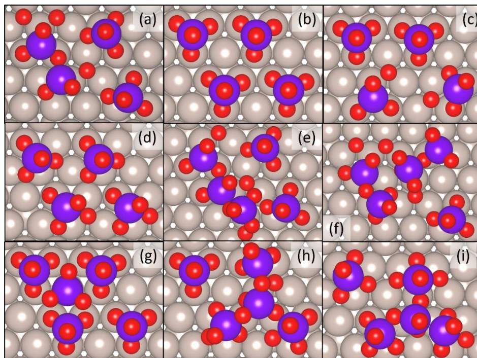
Figure 9.5 RuO 4 coverages for four RuO 4 (a) - (d) and five RuO 4 (e) - (i). Colour scheme is the same as in Figure 9.3.
