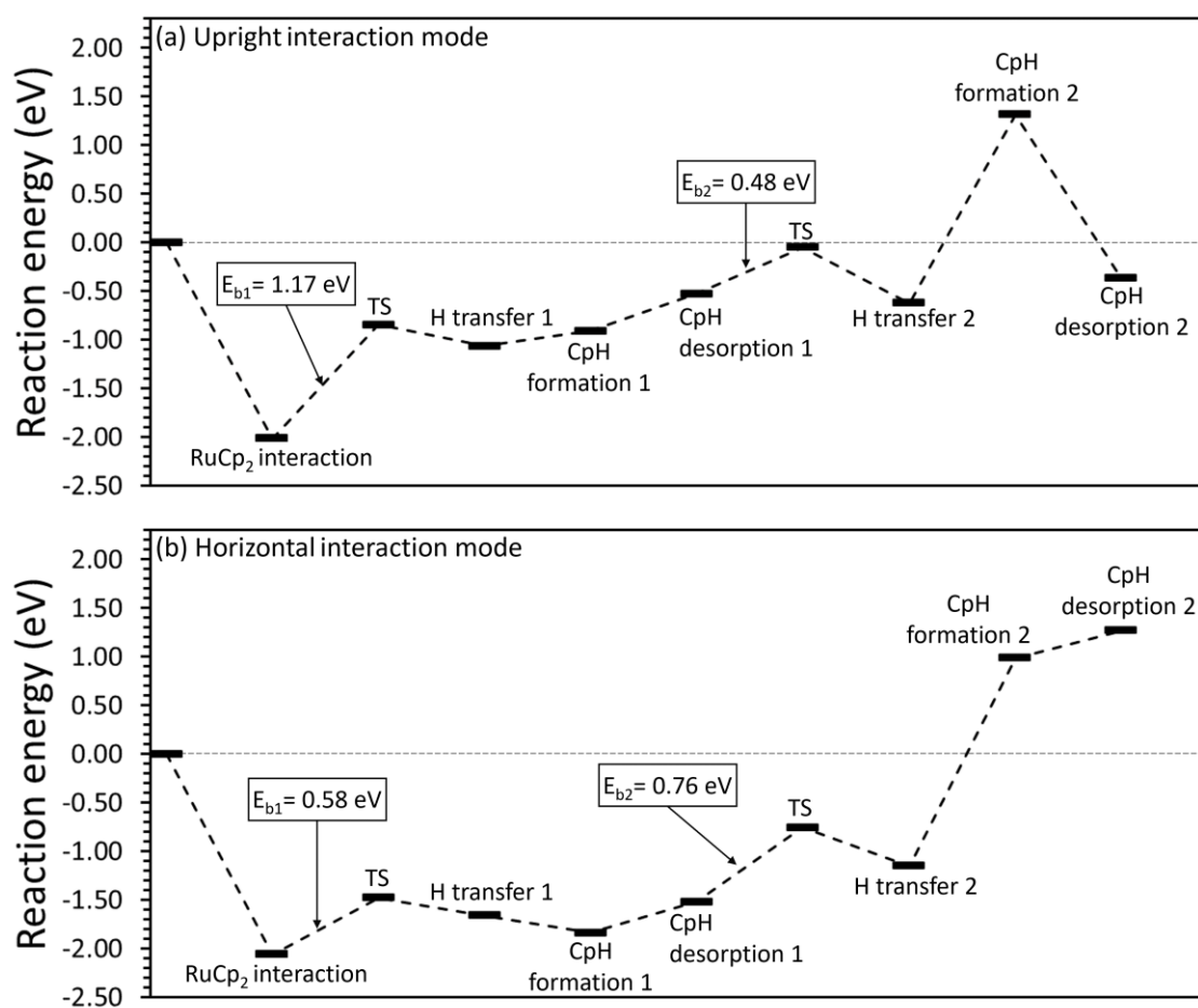
Figure 8.2. RuCp 2 reaction pathway on 1 ML N-H \epsilon -TaN (110) for (a) upright interaction mode and (b) horizontal interaction mode with activation barriers ( E_b ) highlighted in boxes. TS corresponds to the transition state energy for hydrogen transfer. H in H transfer stands for hydrogen.
