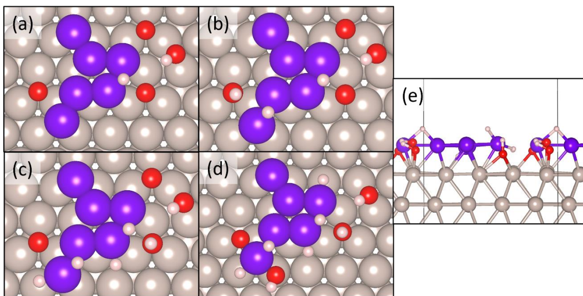
Figure 9.11 Interaction of the 21 st - 24 th added \text{H}_2 where \text{H}_2 dissociated into O-H and \text{Ru} -H bonds. Colour scheme is the same as in Figure 9.9
