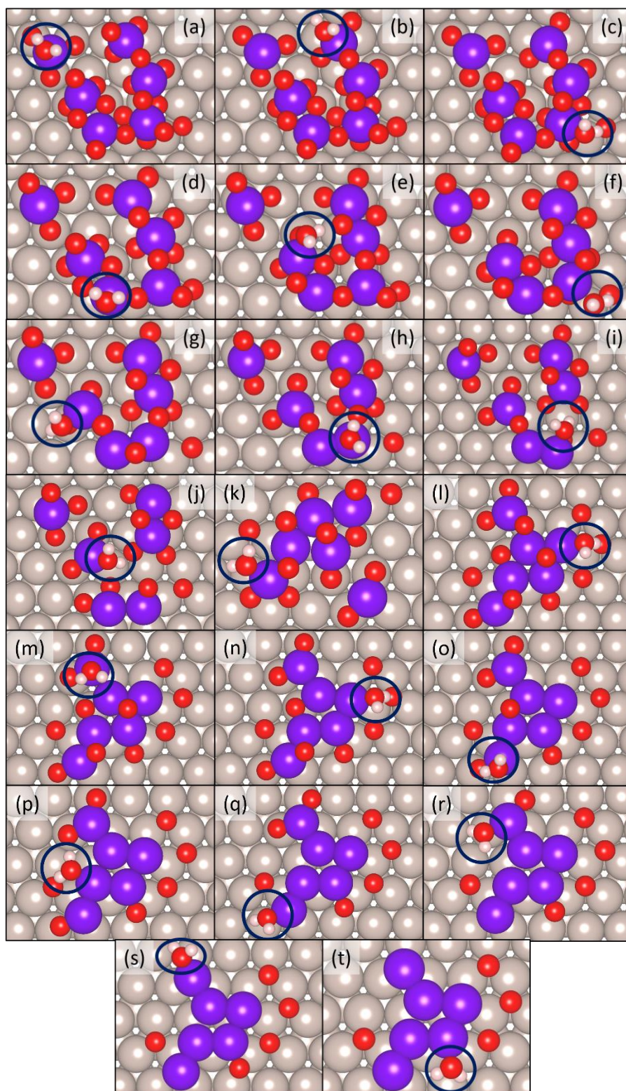
Figure 9.9 Interaction of up to 20 H 2 with the 5.09 RuO 4 /nm 2 terminated Ru surface where H 2 O spontaneously formed at each H 2 interaction. H 2 O highlighted in a circle in each pane (a) - (t). Colour scheme is: Ru = grey, O = red, H = pink and Ru from RuO 4 = purple.
