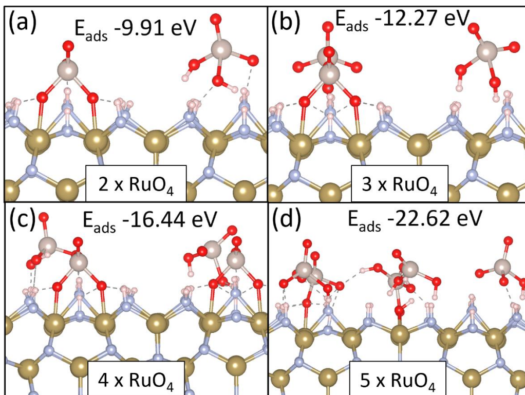
Figure A 7. RuO 4 coverages on 1 ML N-H TaN. Colour scheme is Ta = brown, N = light blue, H = pink, O = red and Ru = grey.
