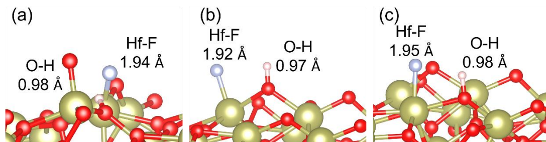
Figure 5.3: Relaxed adsorption structures for one HF molecule interacting with the bare surface of aHfO 2 for (a) 1HF A, (b) 1HF B, and (c) 1HF C. Colour scheme: Hf = gold, O = red H = white and F = light blue.
