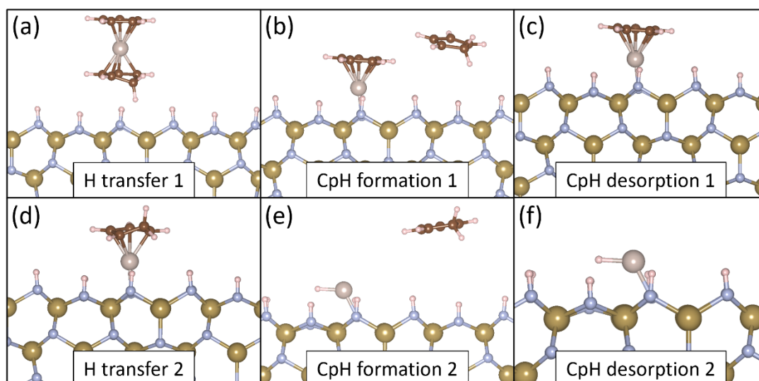
Figure 8.3. Geometries of the individual reaction pathway steps for the upright interaction mode of \text{RuCp}_2 on 1 ML N-H \epsilon -TaN (110). Colour scheme is the same as in Figure 8.1.
