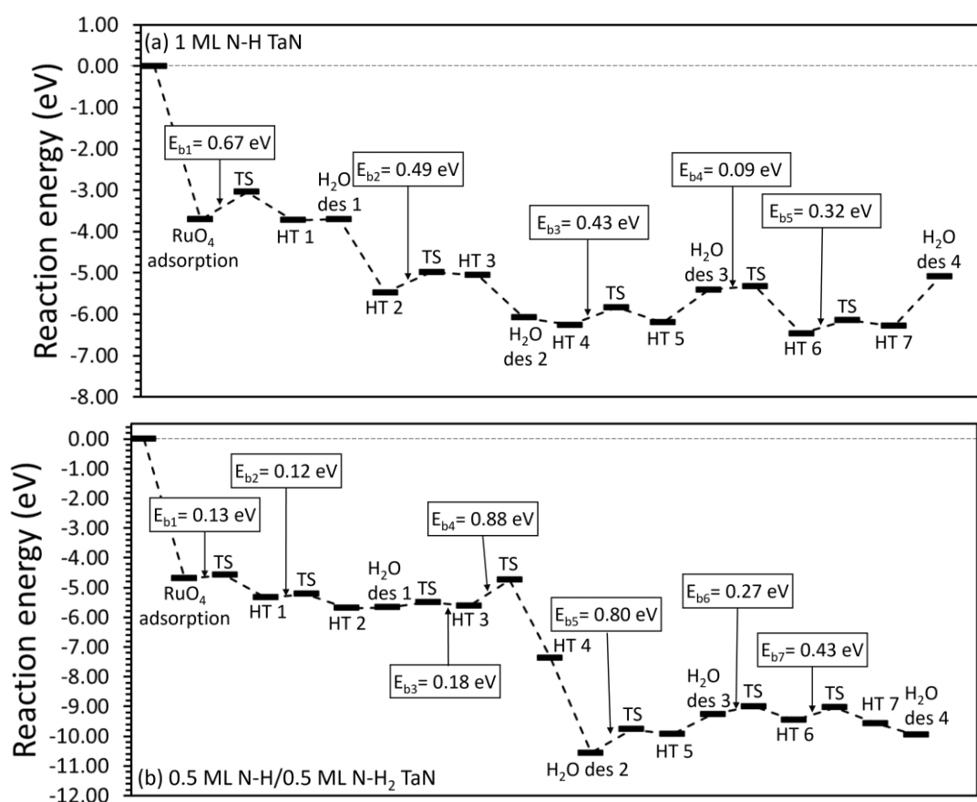
Figure 8.20. RuO 4 reaction pathway on (a) 1 ML N-H and (b) 0.5 ML N-H/0.5 ML N-H 2 ε-TaN (110) surfaces. Note the abbreviations HT = hydrogen transfer and des = desorption.
