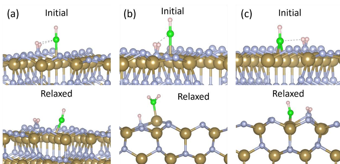
Figure 7.5: Rotated view from Figure 7.4 N-H 2 and Ta-NH terminations on \epsilon -TaN(110). (a) Ta-NH at Ta B , (b) Ta-NH at Ta A and (c) Ta-NH at Ta BC . Colour scheme is the same as in Figure 7.3.
