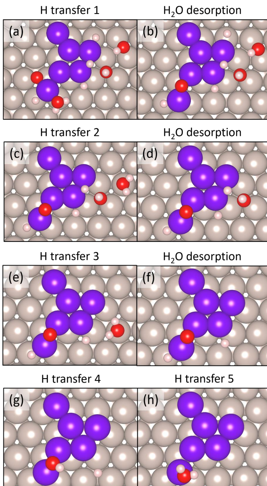
Figure 9.13 Geometries for the reaction pathway steps in Figure 9.12.
