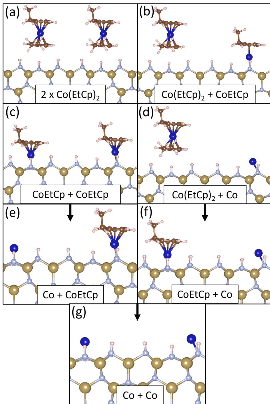
Figure 8.44. Geometries of two \text{Co}(\text{EtCp})_2 adsorbed on the 1 ML N-H \epsilon -TaN (110) surface. Colour scheme is the same as in Figure 8.27.
