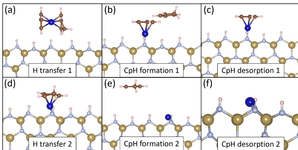
Figure 8.30: Geometries of the individual reaction pathway steps for the horizontal interaction mode of \text{CoCp}_2 on 1 ML N-H \epsilon -TaN (110). Colour scheme is the same as in Figure 8.27.
