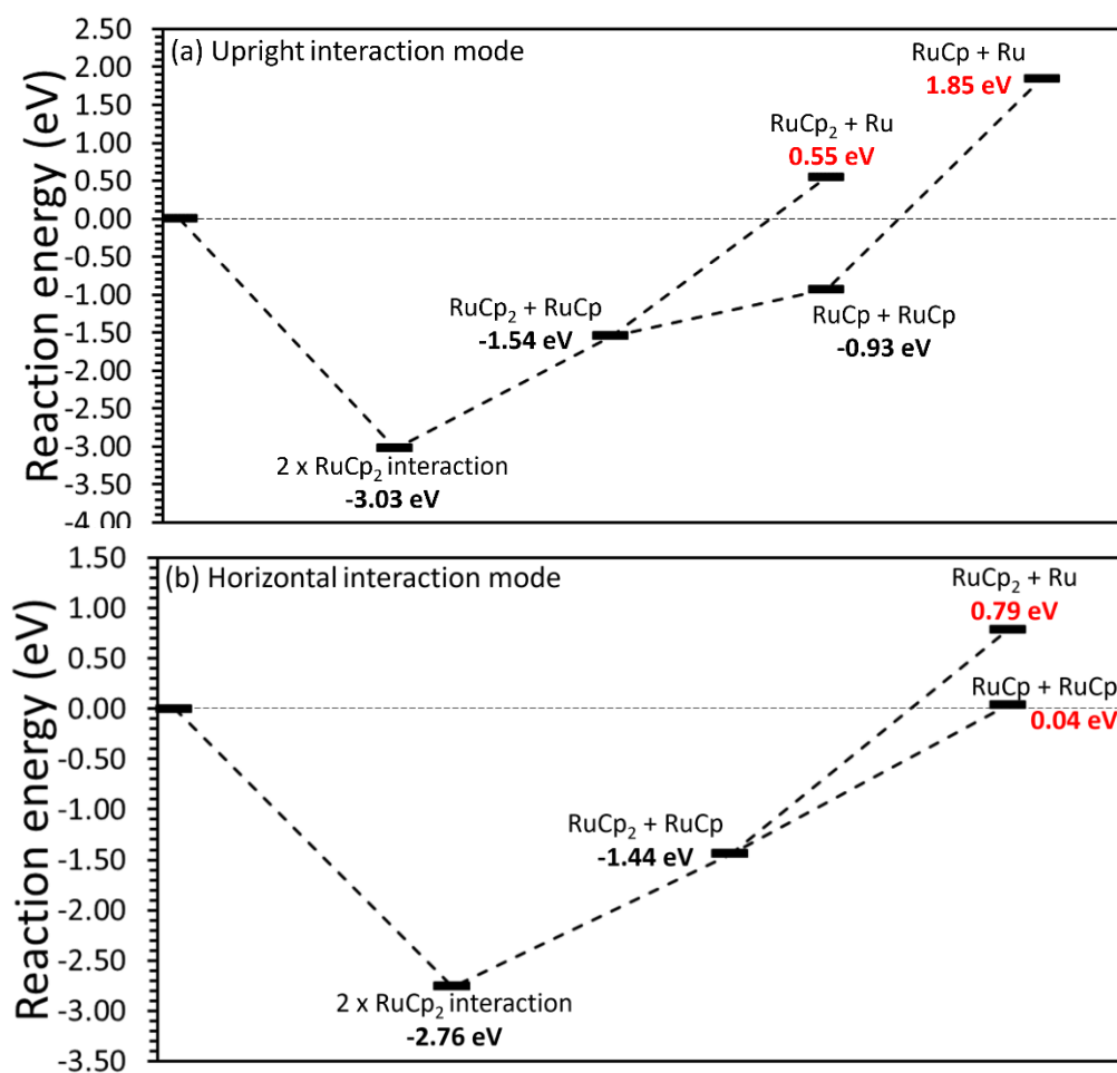
Figure 8.5. Reaction pathway for two RuCp 2 precursors on 1 ML N-H \epsilon -TaN (110) surface for (a) upright interaction mode and (b) horizontal interaction mode.
