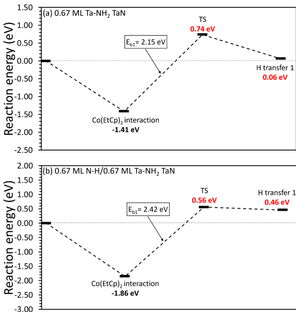
Figure 8.42. \text{Co(EtCp)}_2 reaction pathway on (a) 0.67 ML \text{Ta-NH}_2 and (b) 0.67 ML N-H/0.67 ML \text{Ta-NH}_2 \epsilon -TaN (110) surfaces for the upright interaction mode.
