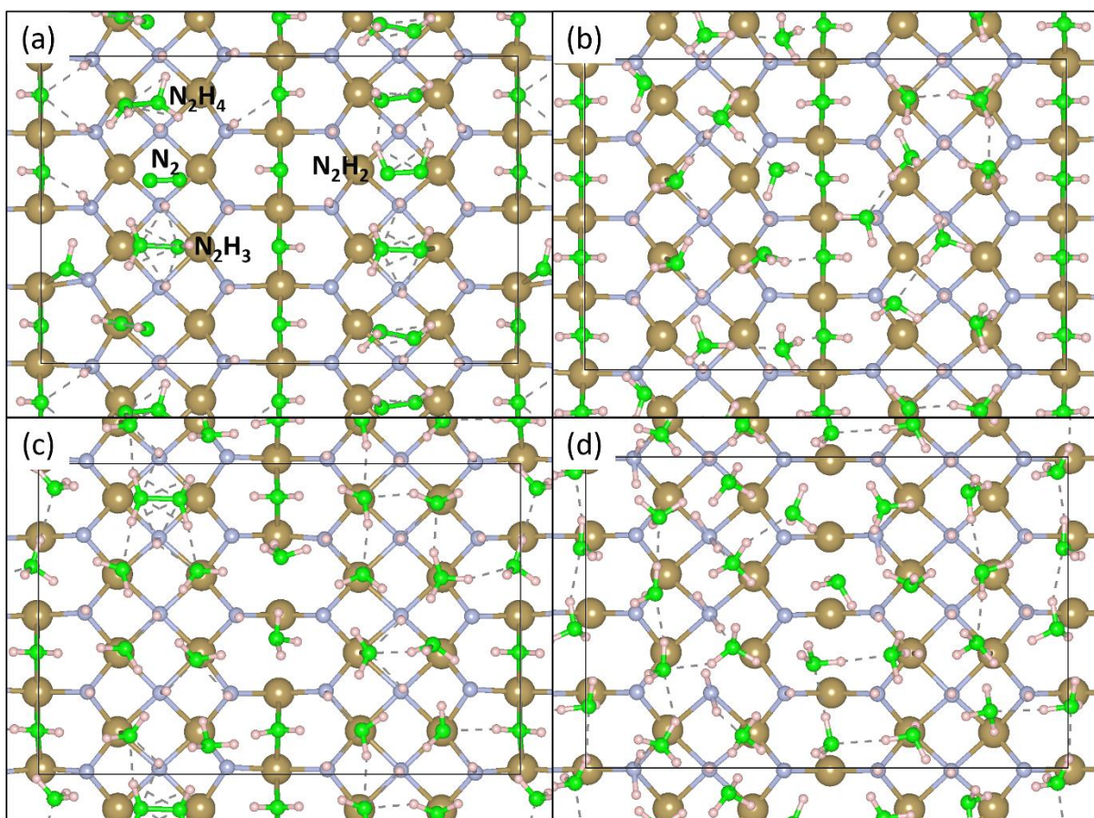
Figure 7.8: Top view of the relaxed structures starting from a coverage of 1ML N-H_x /1ML Ta-NH_x on \epsilon - TaN(110) . (a) 1ML N-H /1ML Ta-NH , (b) 1ML N-H_2 /1ML Ta-NH , (c) 1ML N-H /1ML Ta-NH_2 and (d) 1ML N-H_2 /1ML Ta-NH_2 . Bottom TaN layers have been removed for clarity. Colour scheme is the same as in Figure 7.3.
