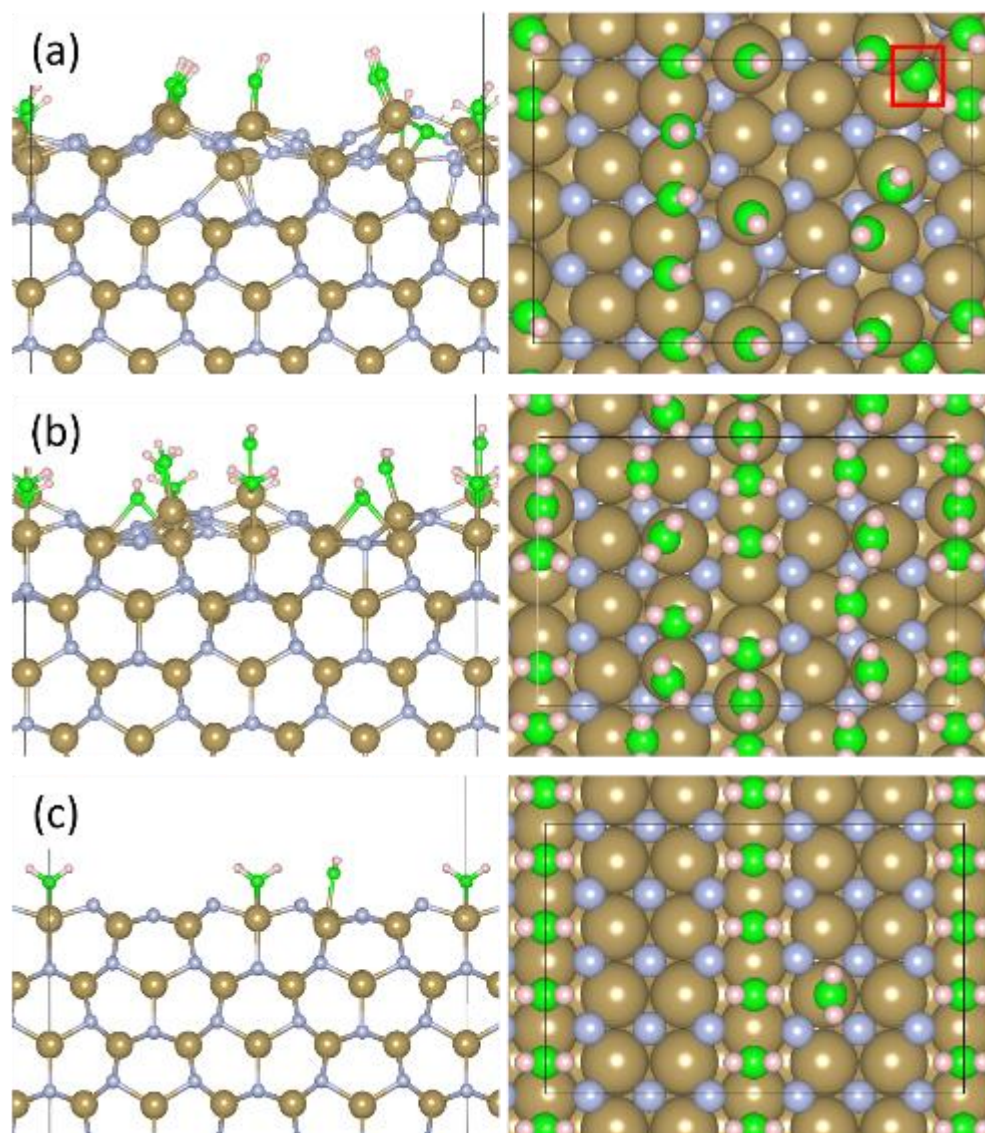
Figure 7.11: Side and top views of Ta-NH x terminated \epsilon -TaN. (a) 0.04 ML Ta-NH 2 /0.42 ML Ta-NH/0.04 ML Ta-N, (b) 0.67 ML Ta-NH 2 and (c) 0.38 ML Ta-NH 2 . Colour scheme is the same as in Figure 7.3.
