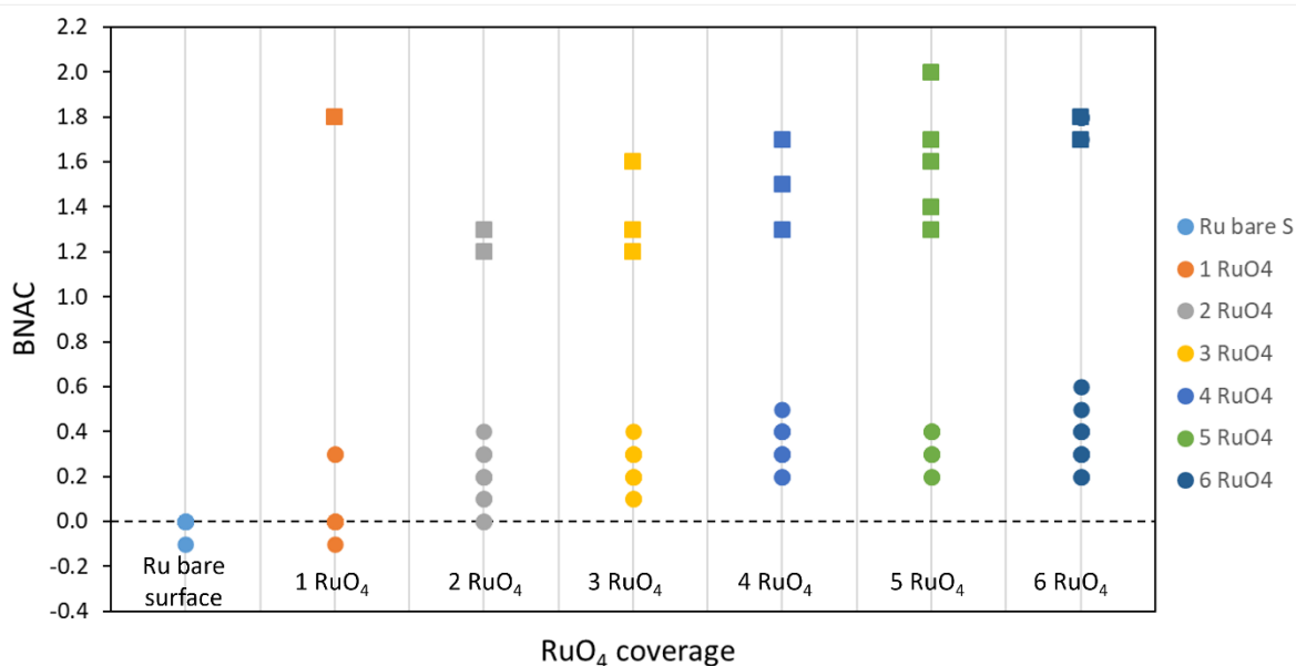
Figure 9.8 Calculated Bader net atomic charge plots for the bare Ru surface and coverages of 0.85 – 5.09 RuO 4 /nm 2 for layer S of the Ru (001) surface. The circle data points refers to Ru S atoms and square data points refers to Ru P atoms. Note that some data points overlap for Ru S and Ru P atoms with the same BNAC value.
