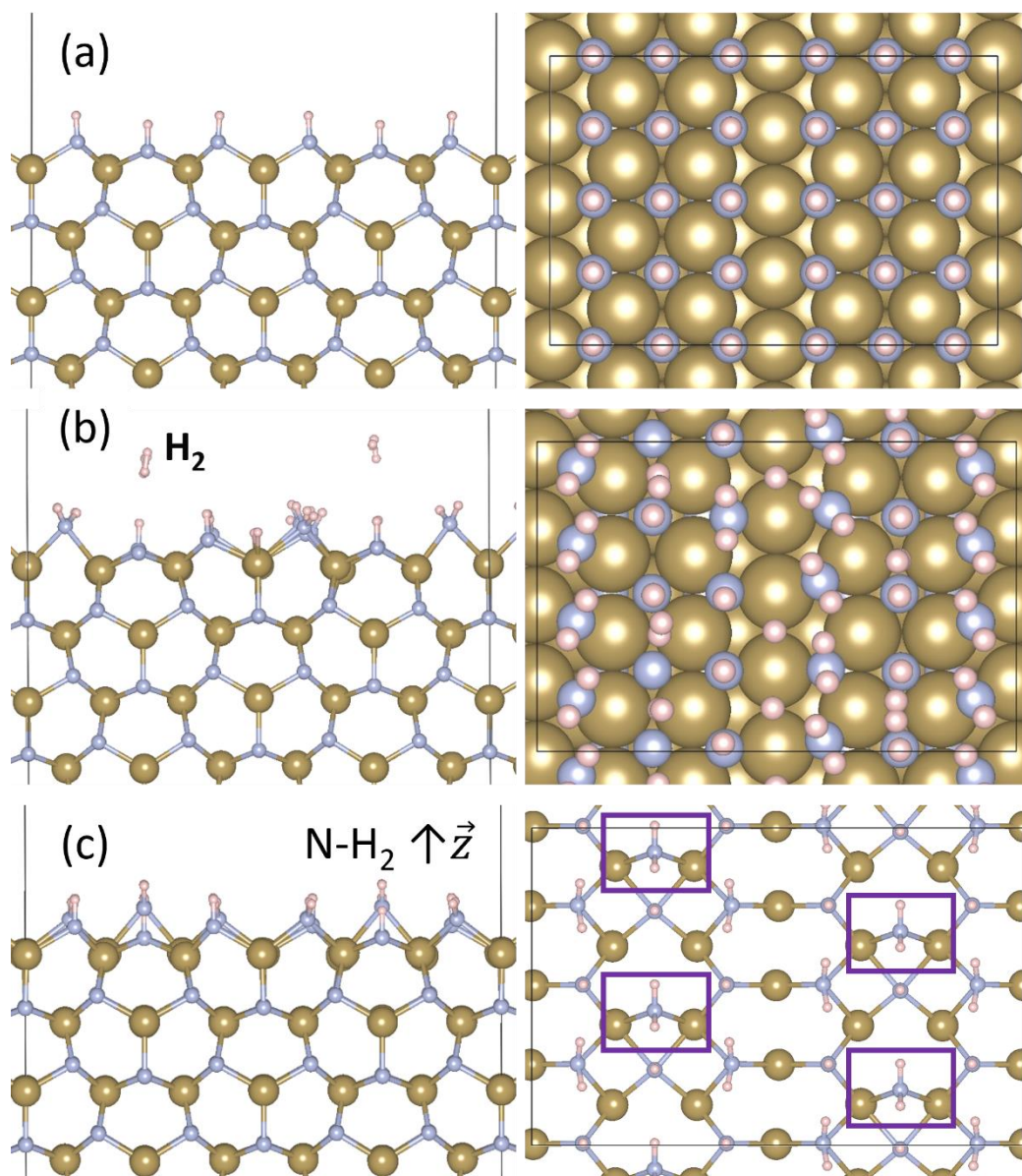
Figure 7.9: Side and top views of N-H_x terminated \epsilon -TaN. (a) 1 ML N-H, (b) 1 ML N-H 2 and (c) 0.5 ML N-H/0.5 ML N-H 2 . Colour scheme is the same as in Figure 7.2.
