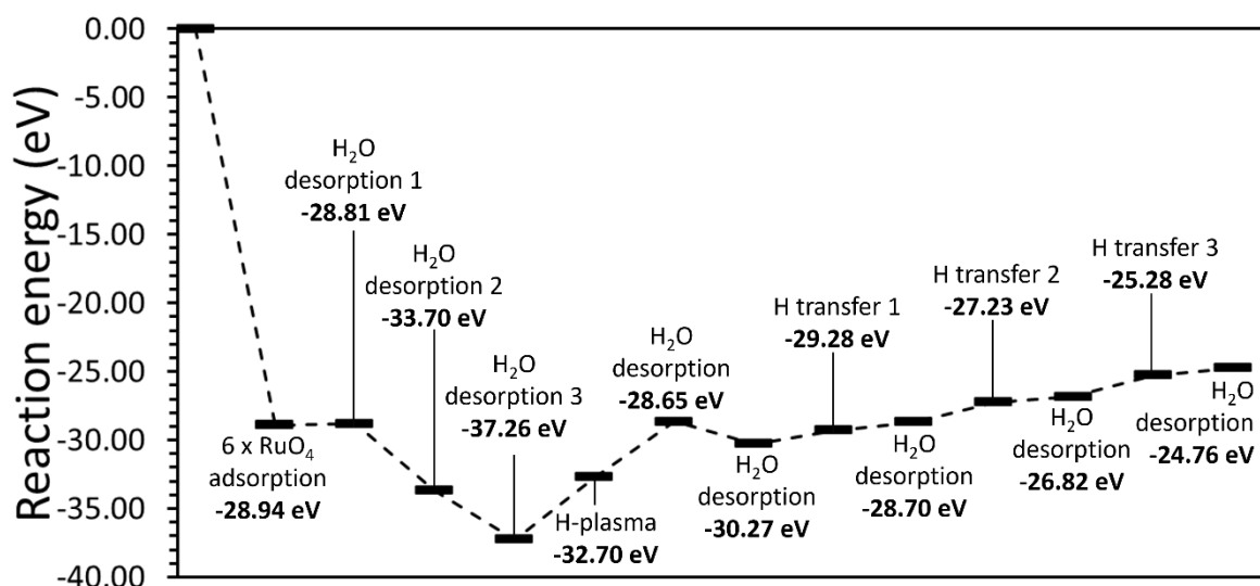
Figure 8.24 Reaction pathway of 6 \times \text{RuO}_4 on 0.5 ML N-H/0.5 ML N- \text{H}_2 \epsilon -TaN (110) surface.
