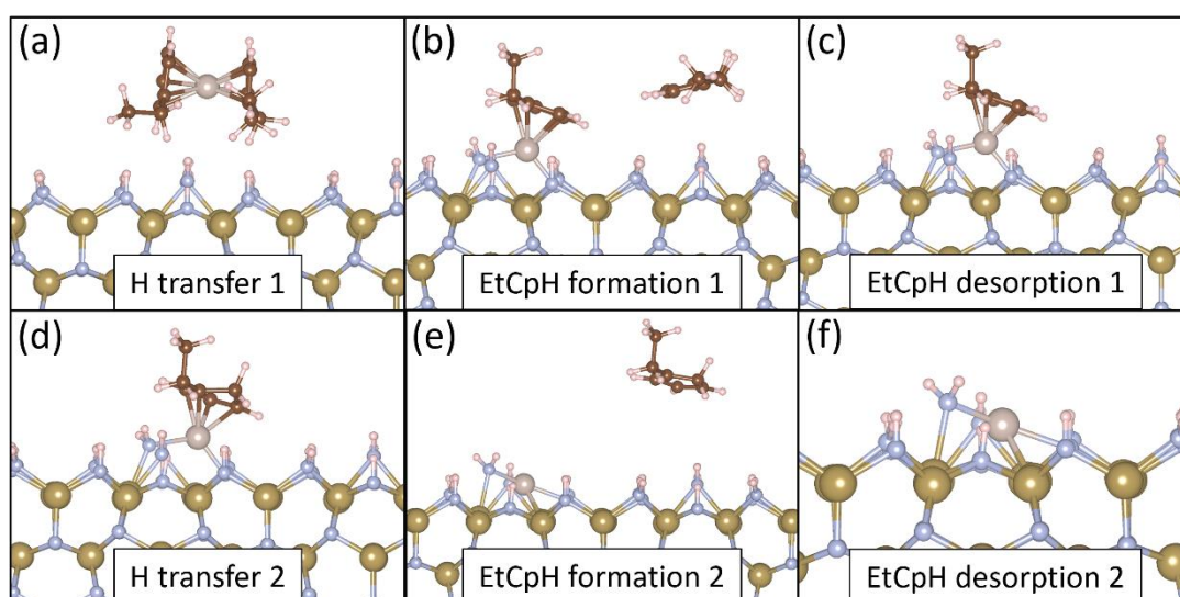
Figure 8.13. Geometries of the individual reaction pathway steps for the horizontal interaction mode of \text{Ru}(\text{EtCp})_2 on 0.5 ML N-H/0.5 ML \text{N-H}_2 \epsilon -TaN (110). Colour scheme is the same as in Figure 8.1.
