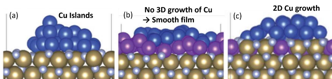
Figure 2.9 Cu morphology on (a) Bare TaN, (b) 1 ML Ru passivated TaN and (c) 50% Ru doped TaN. Colour coding: Ta = brown, N = light blue, Cu = dark and Ru = purple. Adapted from ref. 101 .
