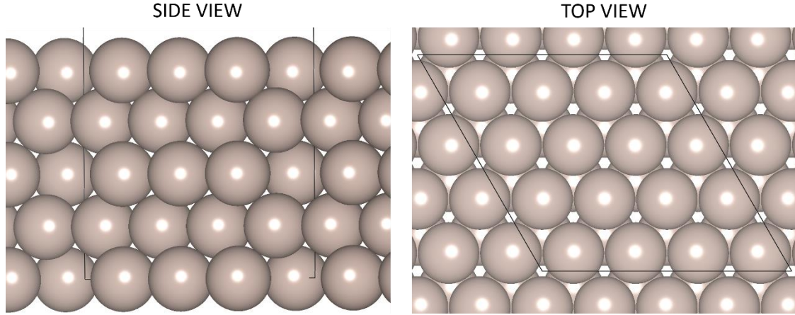
Figure 3.10: Side view and Top view of the Ru (001) surface. Colour scheme is Ru = grey.
