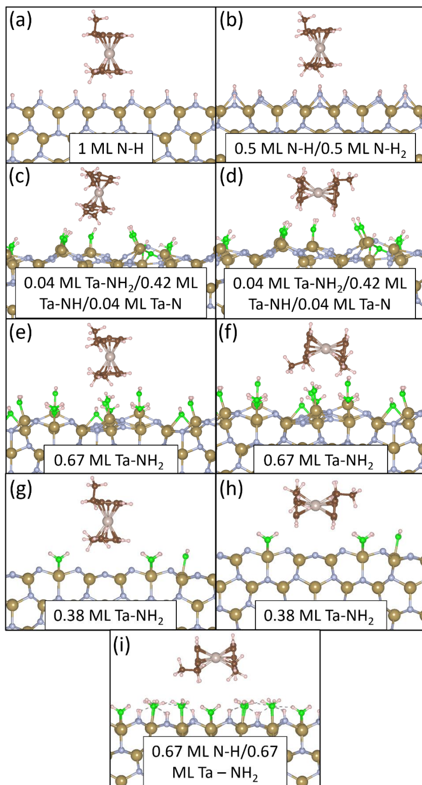
Figure A 5. Ru(EtCp) 2 adsorption at NH x -terminated TaN surfaces. Colour scheme is the same as in Figure A 4.
