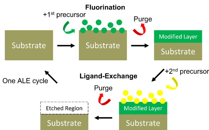
Figure 2.2. Schematic model of the thermal ALE process.
