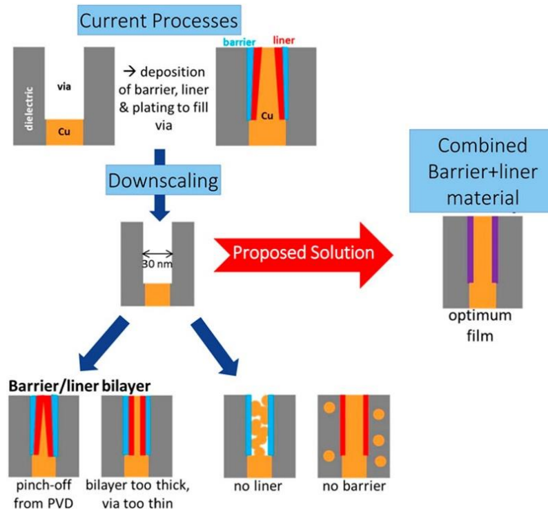
Figure 2.8: Challenges involved with the interconnect bottleneck and proposed solutions. Taken from ref 96 .
