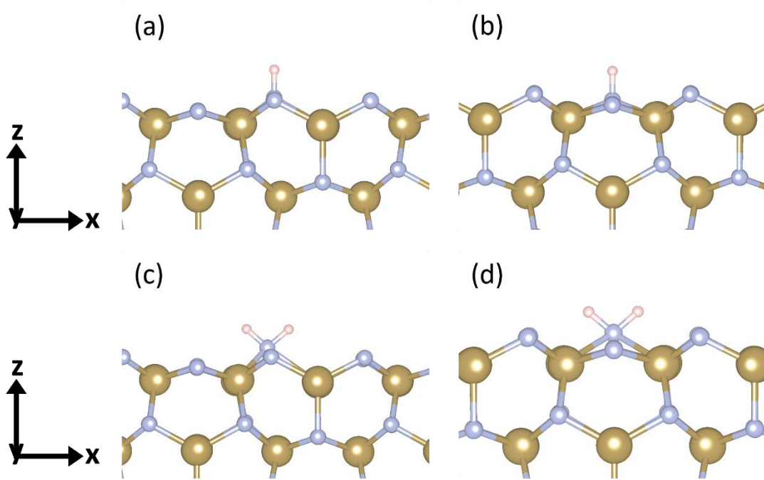
Figure 7.2: Single \text{N-H}_x adsorbed at different N sites on \varepsilon\text{-TaN}(110) surface. (a) \text{N-H} at \text{N}^a , (b) \text{N-H} at \text{N}^b , (c) \text{N-H}_2 at \text{N}^a and (d) \text{N-H}_2 at \text{N}^b . Colour scheme is: Ta = brown, N = blue and H = pink.
