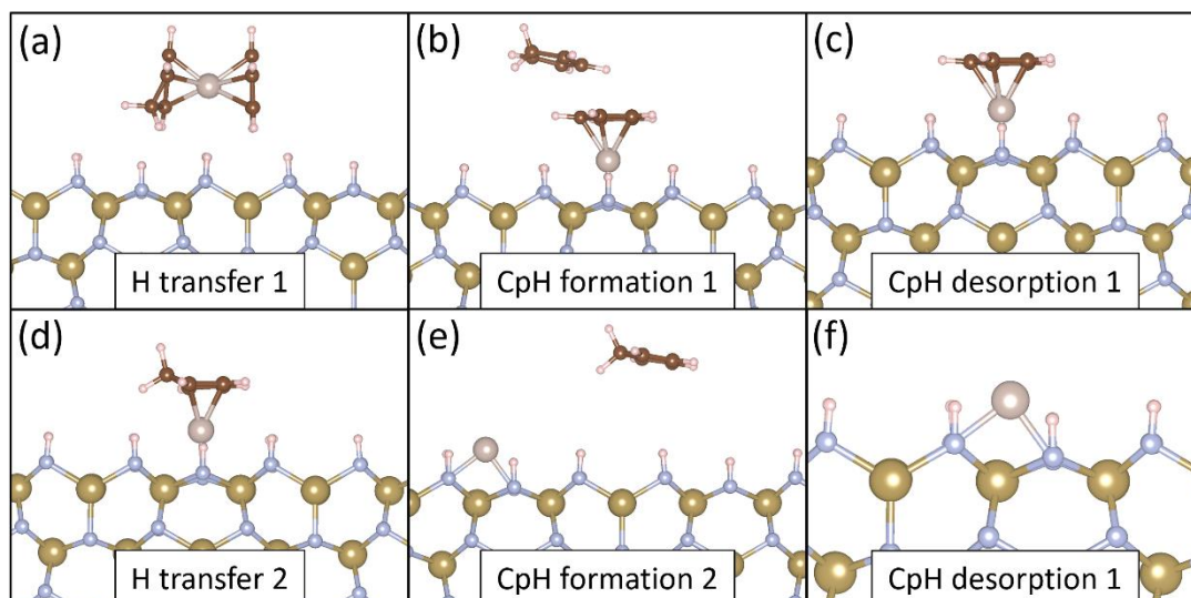
Figure 8.4. Geometries of the individual reaction pathway steps for the horizontal interaction mode of \text{RuCp}_2 on 1 ML N-H \epsilon -TaN (110). Colour scheme is the same as in Figure 8.1.
