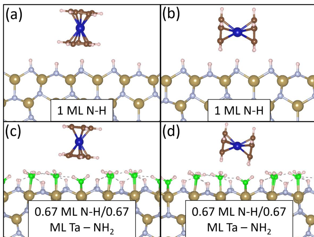
Figure 8.27. Atomic structure of CoCp 2 interaction modes on (a) Upright interaction mode on 1 ML N-H, (b) Horizontal interaction mode on 1 ML N-H, (c) Upright interaction mode on 0.67 ML Ta-NH 2 /0.67 ML N-H and (d) Horizontal interaction mode on 0.67 ML Ta-NH 2 /0.67 ML N-H \epsilon -TaN (110) surfaces.
