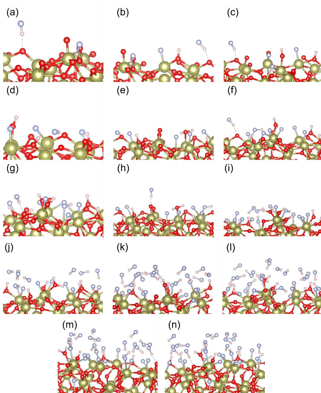
Figure A 3: Relaxed geometries for different HF coverages of amorphous \text{HfO}_2 where a mixture of molecular and dissociative adsorption of HF is observed. (a) 2HF A, (b) 3HF A, (c) 4HF A (d) 4HF C, (e) 5HF C, (f) 8HF A, (g) 8HF B, (h) 8HF C, (i) 16HF A, (j) 16HF B, (k) 28HF, (l) 30HF, (m) 32 HF and (n) 34 HF. Colour scheme same as in Error! Reference source not found..
