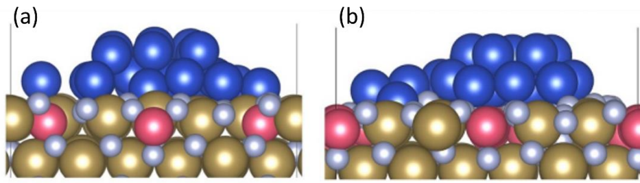
Figure 2.10 Cu morphology on (a) 25% Co doped TaN and (b) 50% Co doped TaN. Colour coding: Ta = brown, N = light blue, Cu = dark blue and Co = pink. Adapted from ref
