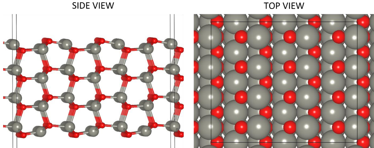
Figure 3.9: Side view and Top view of the ZnO (10\bar{1}0) surface. Colour scheme is: Zn = grey and O = red.
