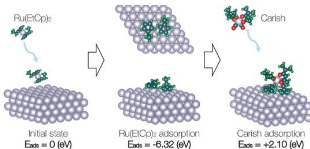
Figure 2.13: Ru(EtCp) 2 on Ru substrate and Carish on EtCp-terminated surface. Adapted from ref 179 .
