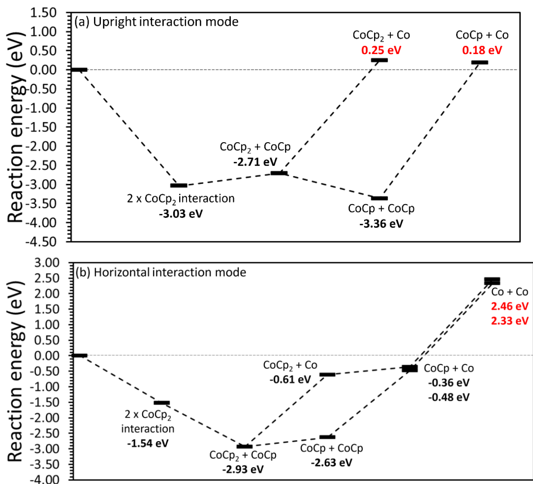
Figure 8.32: Reaction pathway for two CoCp 2 precursors on 1 ML N-H ε-TaN (110) surface for (a) upright interaction mode and (b) horizontal interaction mode.
