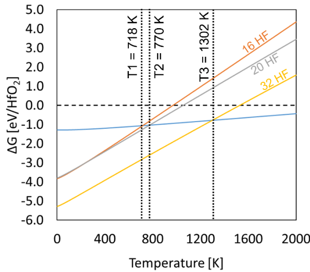
Figure 5.2: Free energy profiles of the spontaneous etching and self-limiting reactions for aHfO 2 . T1, T2, and T3 are the temperatures where the self-limiting and spontaneous etch reactions cross over for 8O/16F, 10O/20F, and 16O/32F models, respectively.
