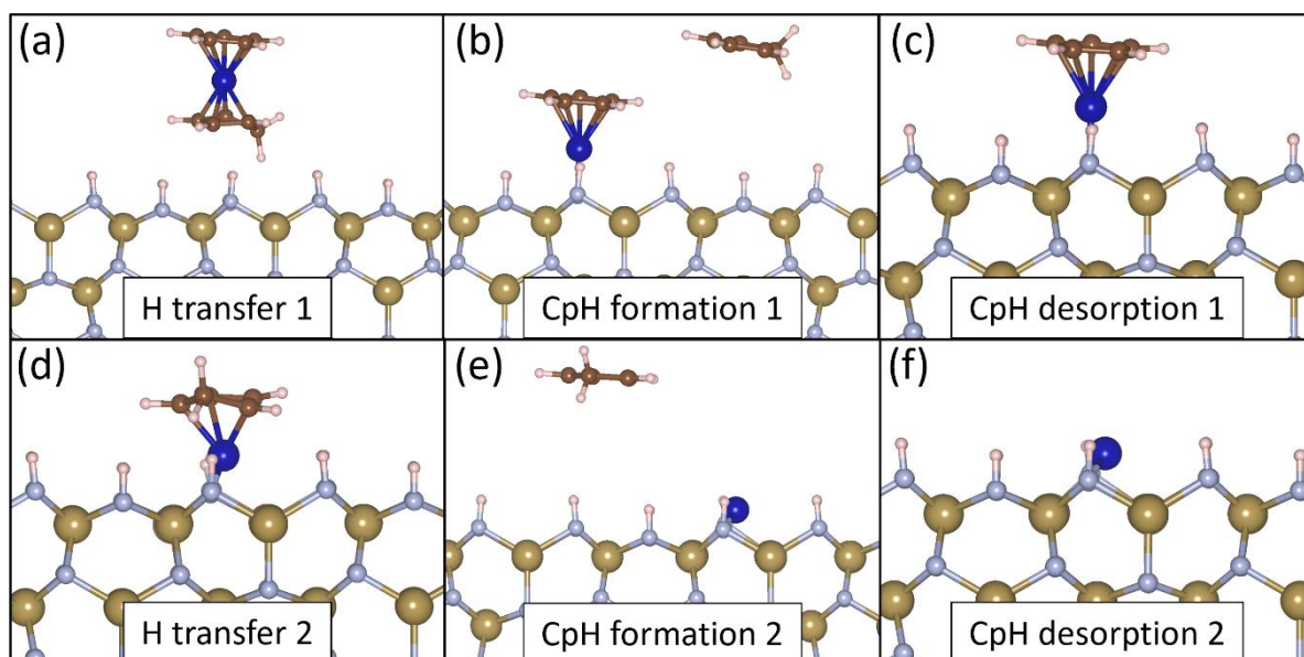
Figure 8.29: Geometries of the individual reaction pathway steps for the upright interaction mode of \text{CoCp}_2 on 1 ML N-H \epsilon - \text{TaN} (110). Colour scheme is the same as in Figure 8.27.
