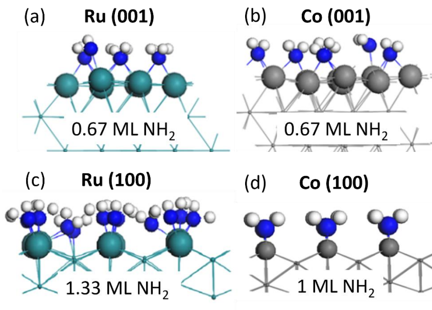
Figure 2.12: \text{NH}_2 coverage on (a) Ru(001), (b) Co(001), (c) Ru(100) and (d) Co(100) surface facets. Taken from ref 175 .
