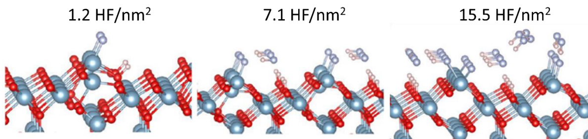
Figure 2.6: HF coverage on ( \bar{2} 0 1 ) \text{Al}_2\text{O}_3 surface. Adapted from ref 84 .
