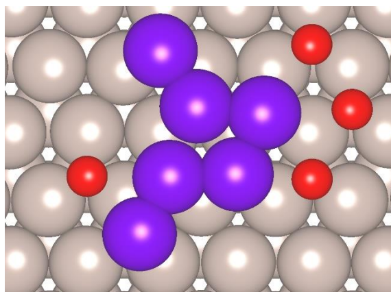
Figure 9.10: Ru (001) surface terminated with 6 \text{Ru}^{\text{P}} and four O atoms after the interaction of up to 20 \text{H}_2 molecules. Colour scheme is the same as in Figure 9.9.
