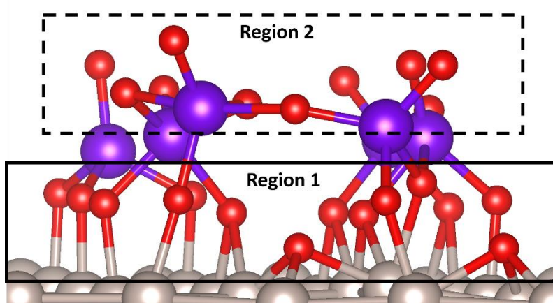
Figure 9.7 Side view of 6 x RuO 4 on Ru surface. Colour scheme is the same as in Figure 9.3.
