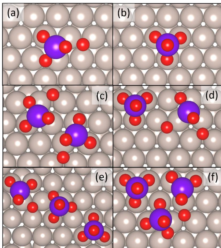
Figure 9.4 RuO 4 coverages for one RuO 4 (a) & (b), two RuO 4 (c) & (d) and three RuO 4 (e) & (f). Colour scheme is the same as in Figure 9.3.
