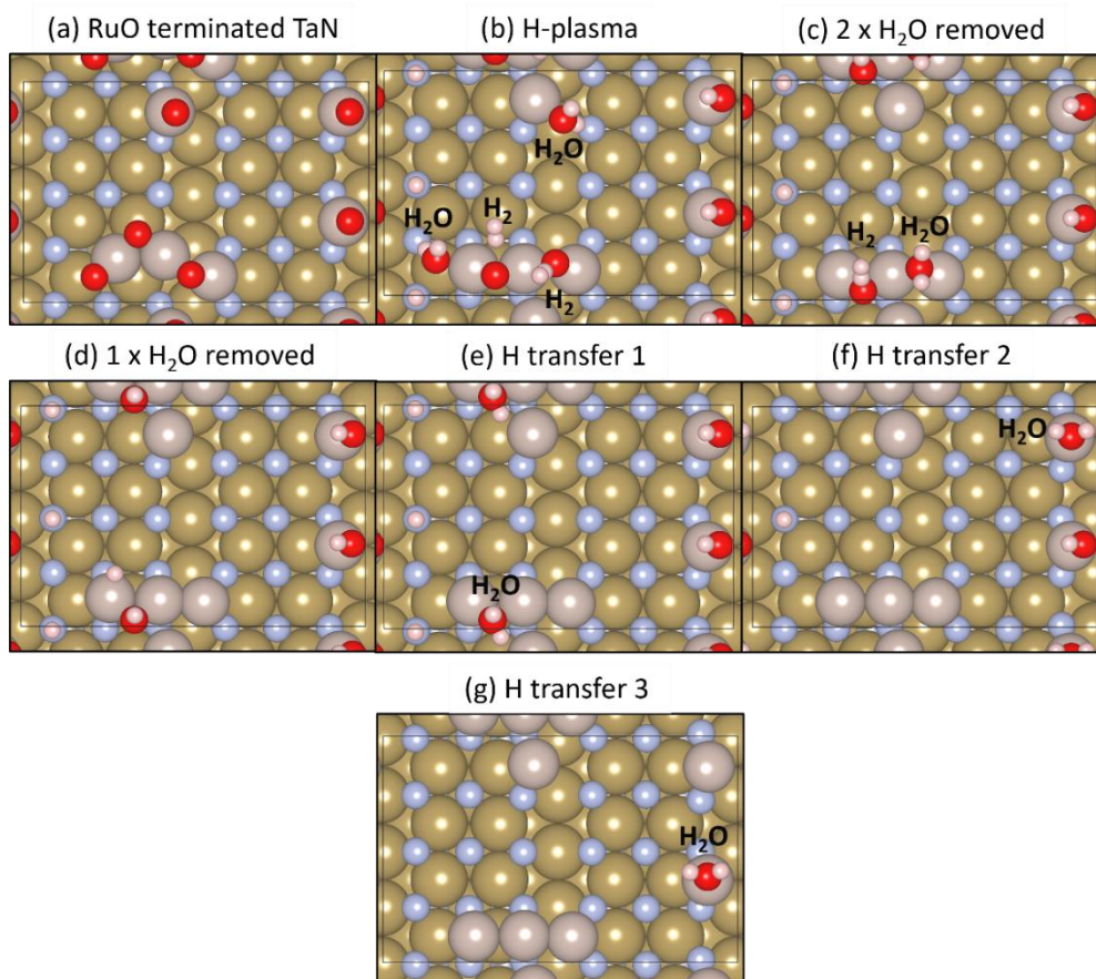
Figure 8.25. H-plasma on post metal precursor RuO 4 treated 0.5 ML N-H/0.5 ML N-H 2 \epsilon -TaN (110) surface. Colour scheme is the same as in Figure 8.19.
