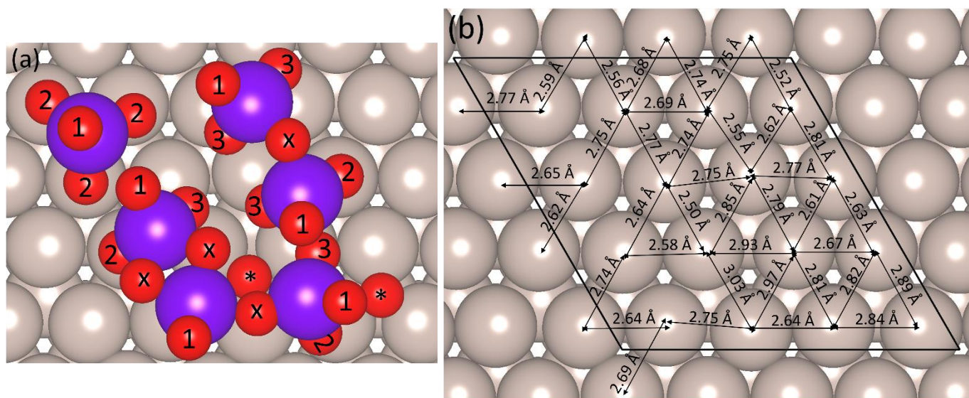
Figure 9.6 (a) Top view of 5.09 RuO 4 /nm 2 coverage on Ru surface. (b) Ru S -Ru S bond lengths in top surface layer. (note added Ru and O atoms removed for clarity). Colour scheme is the same as in Figure 9.3.
