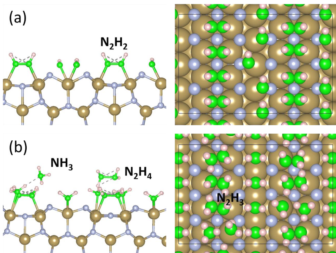
Figure 7.10: Side and top views of Ta-NH x terminated \epsilon -TaN. (a) 1 ML Ta-NH and (b) 1 ML Ta-NH 2 . Colour scheme is the same as in Figure 7.3.
