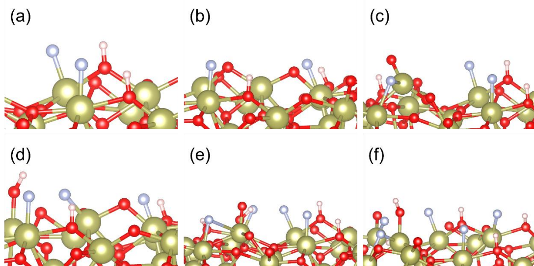
Figure 5.4: Relaxed geometries for HF coverages (a) 2HF B, (b) 2HF C, (c) 3HF B, (d) 3HF C, (e) 4HF B, and (f) 5HF A of amorphous \text{HfO}_2 , where complete dissociation of HF occurred spontaneously. Colour coding is the same as in Figure 5.3.
