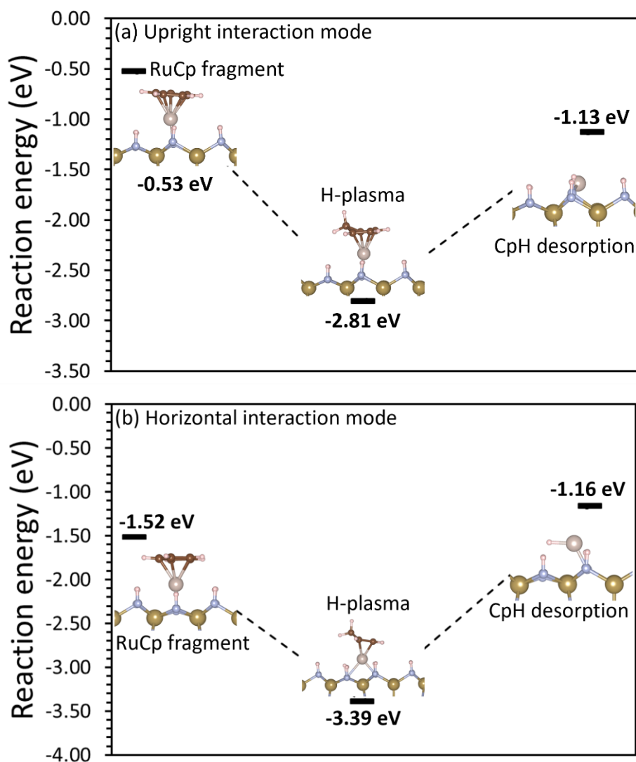
Figure 8.9. Reaction pathway of \cdot\text{H} radical treated RuCp terminated 0.96 ML N-H \epsilon -TaN (110) surface for (a) upright interaction mode and (b) horizontal interaction mode. Energies are relative to the energy of the RuCp adsorbed on the TaN surface. Colour scheme is the same as in Figure 8.1.
