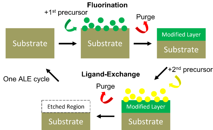
Figure 1.2: Schematic model of the thermal ALE process. 50
