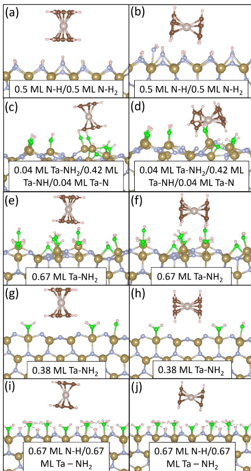
Figure A 4. RuCp 2 interaction at NH x -terminated TaN surfaces. Colour scheme is Ta = brown, N = blue & green, H = pink, C = dark brown and Ru = grey.
