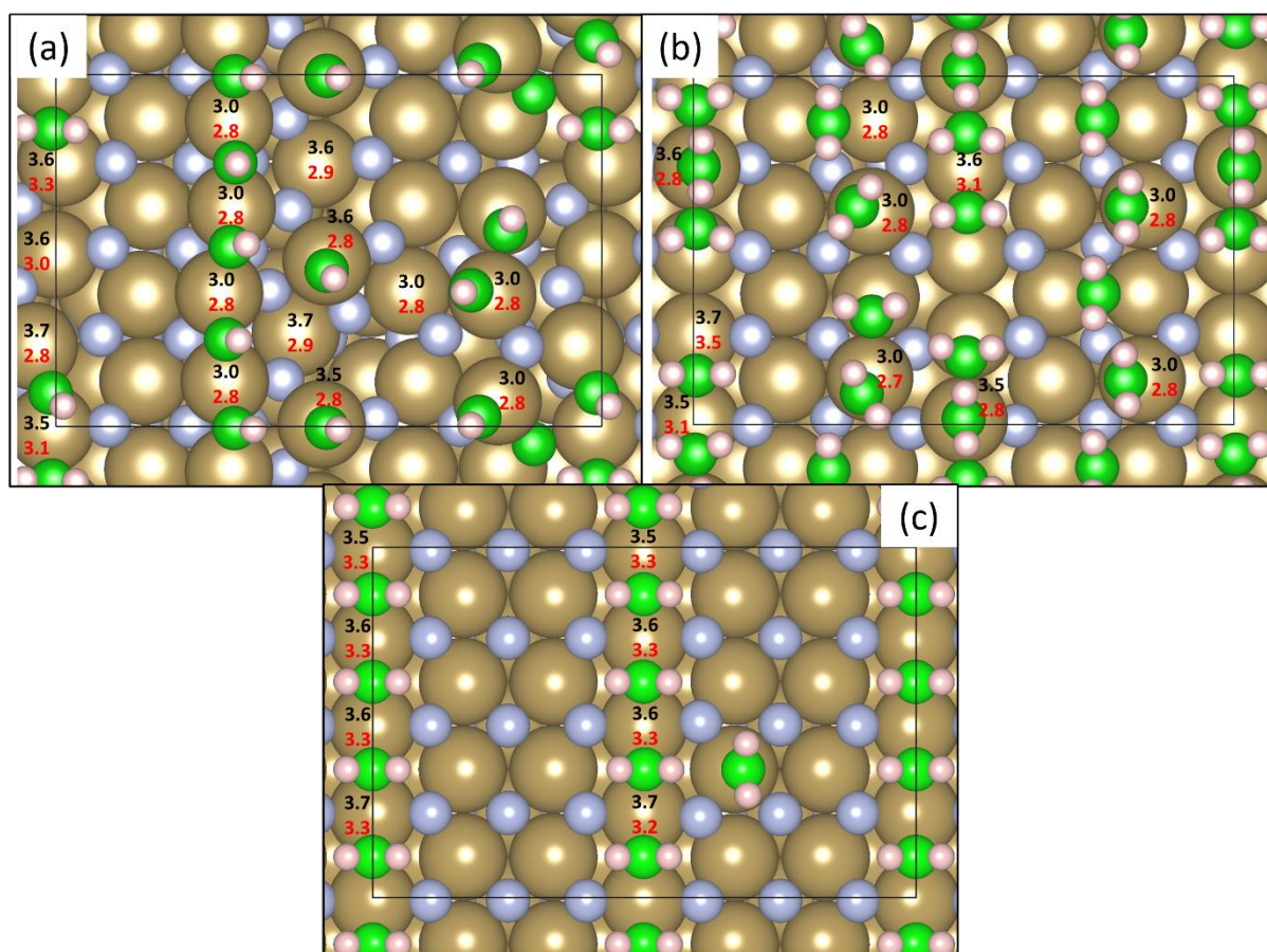
Figure 7.13: Oxidation of Ta atoms upon the adsorption of \text{NH}_x . Black is Ta charge for bare \epsilon -TaN (110) surface and red is Ta charge after \text{NH}_x adsorption for (a) 0.04 ML Ta- \text{NH}_2 /0.42 ML Ta-NH/0.04 ML Ta-N, (b) 0.67 ML Ta- \text{NH}_2 and (c) 0.38 ML Ta- \text{NH}_2 . Colour scheme is the same as in Figure 7.3.
