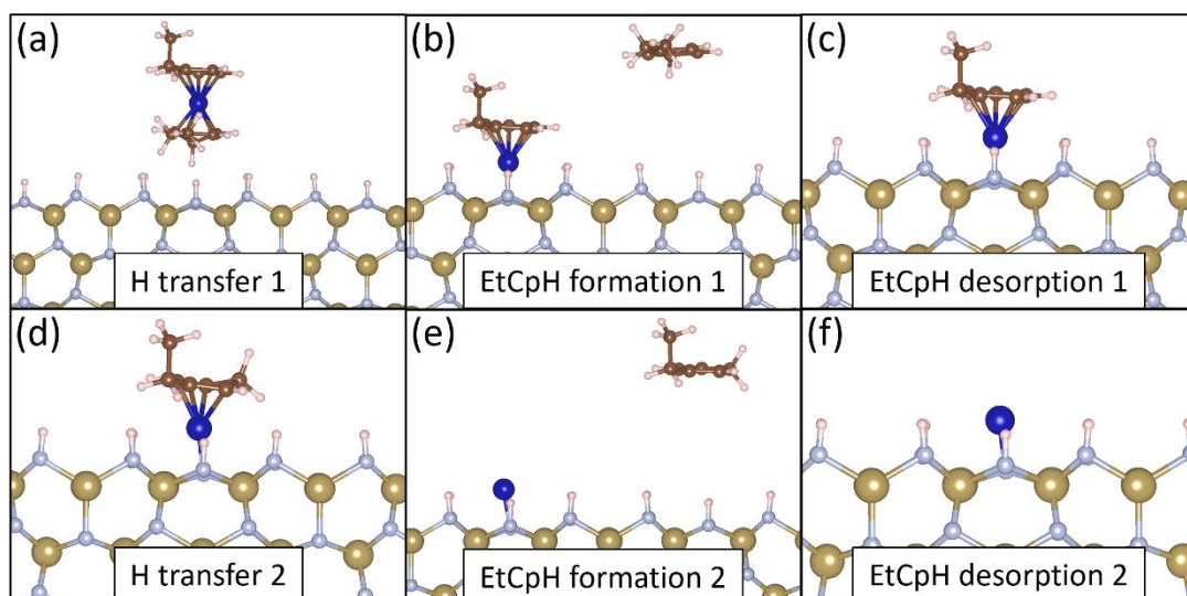
Figure 8.40. Geometries of the individual reaction pathway steps for the upright interaction mode of \text{Co}(\text{EtCp})_2 on 1 ML N-H \epsilon -TaN (110). Colour scheme is the same as in Figure 8.27.
