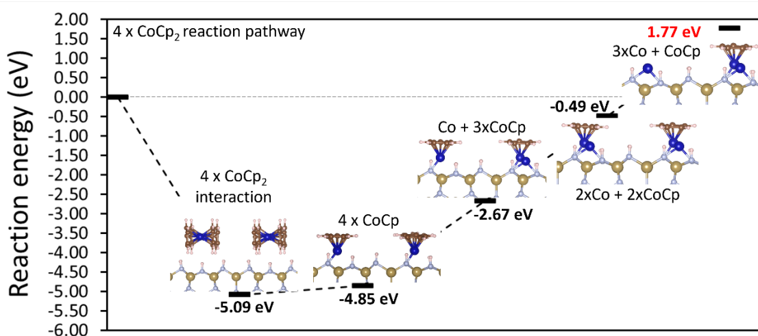
Figure 8.35 Reaction pathway for four CoCp 2 precursors adsorbed on the 1 ML N-H \epsilon -TaN (110) surface. Colour scheme is the same as in Figure 8.27.
