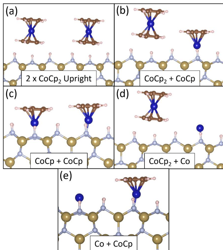
Figure 8.33: Geometries of the reaction pathway of two CoCp 2 precursors on 1 ML N-H \epsilon -TaN (110) surface for the reaction pathway shown in Figure 8.32 (a). Colour scheme is the same as in Figure 8.27
