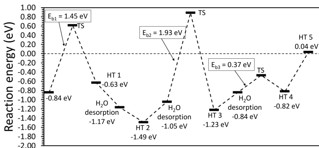
Figure 9.12 Reaction pathway for \text{H}_2\text{O} formation and desorption to remove oxygen from the Ru surface. HT = hydrogen transfer. TS = transition state.
