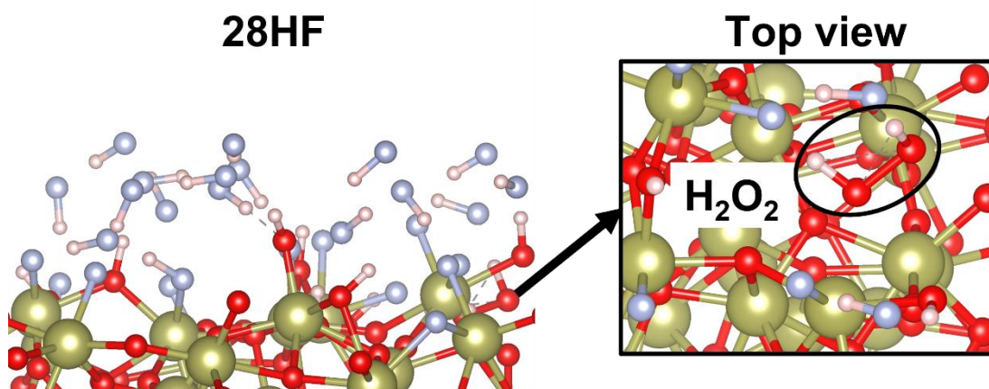
Figure 5.7: Relaxed geometry for 28HF, where H 2 O 2 formed spontaneously. Colour scheme same as in Figure 5.3.
