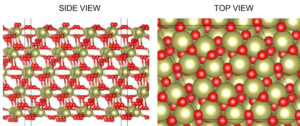
Figure 3.2: Side view and top view of monoclinic (111) surface supercell of HfO 2 . Colour scheme: Hf = gold and O = red.
