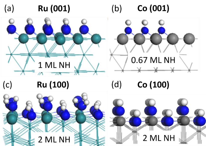
Figure 2.11: \text{NH} coverage on (a) \text{Ru}(001) , (b) \text{Co}(001) , (c) \text{Ru}(100) and (d) \text{Co}(100) surface facets. Adapted from ref 175 .
