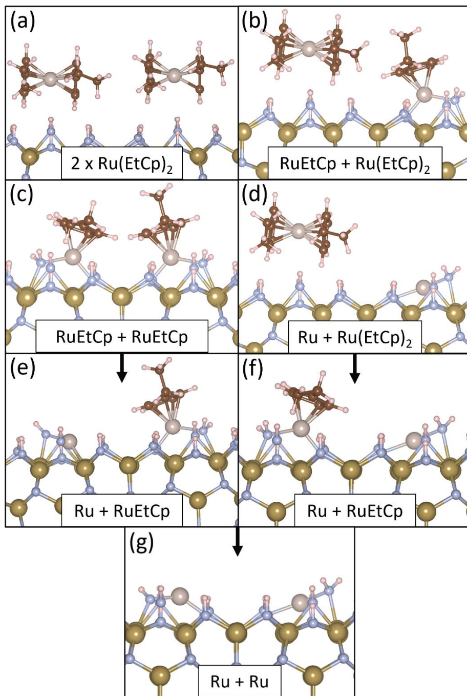
Figure 8.16 Geometries of two \text{Ru}(\text{EtCp})_2 on the 0.5 ML N-H/0.5 ML N-H 2 \epsilon -TaN (110) surface. Colour scheme is the same as in Figure 8.1.
