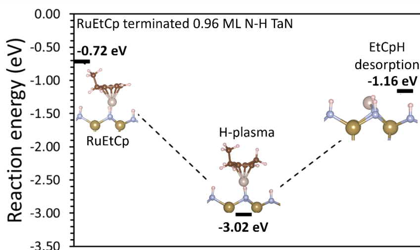
Figure 8.17 Reaction pathway of \cdot\text{H} radical treated RuEtCp terminated 0.96 ML N-H \epsilon -TaN (110) surface. Colour scheme is the same as in Figure 8.1.
