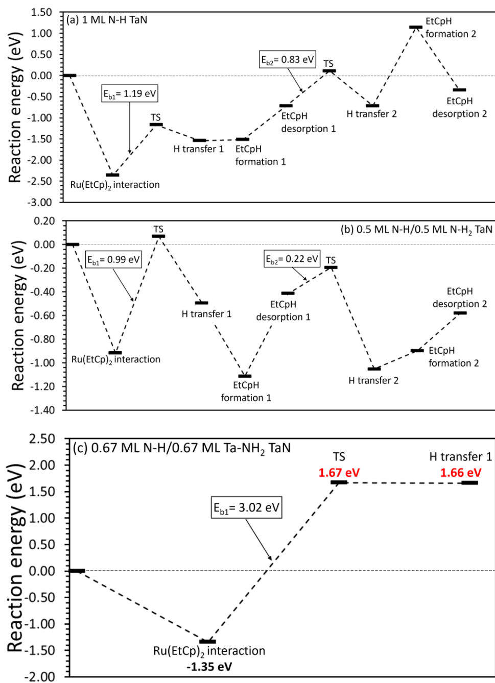
Figure 8.11. \text{Ru(EtCp)}_2 reaction pathway on (a) 1 ML N-H (horizontal interaction mode), (b) 0.5 ML N-H/0.5 ML N-H 2 (horizontal interaction mode) and (c) 0.67 ML N-H/0.67 ML Ta-NH 2 (upright interaction mode) \epsilon -TaN (110) surfaces.
