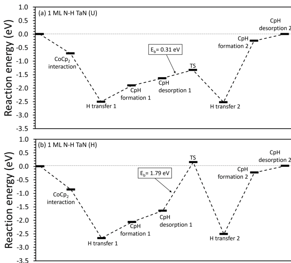
Figure 8.28: \text{CoCp}_2 reaction pathway on (a) 1 ML N-H (upright interaction mode) and (b) 1 ML N-H (horizontal interaction mode) \epsilon - \text{TaN} (110) surfaces.
