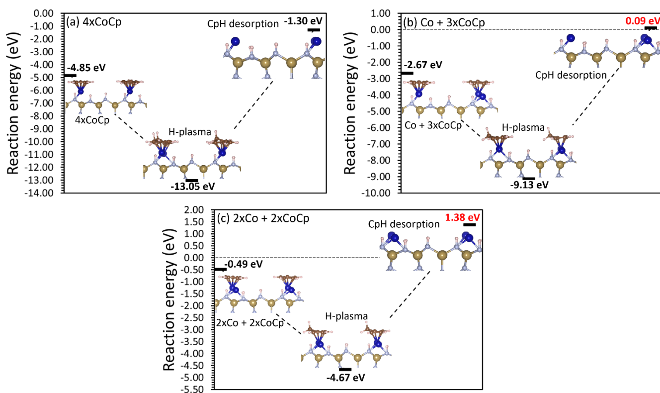
Figure 8.37: Reaction pathway of plasma generated hydrogen radicals at (a) (\text{CoCp})_4 0.83 ML N-H, (b) (\text{CoCp})_3 + \text{Co} 0.79 ML N-H and (c) (\text{CoCp})_2 + (\text{Co})_2 0.75 ML N-H \varepsilon -TaN (110).
