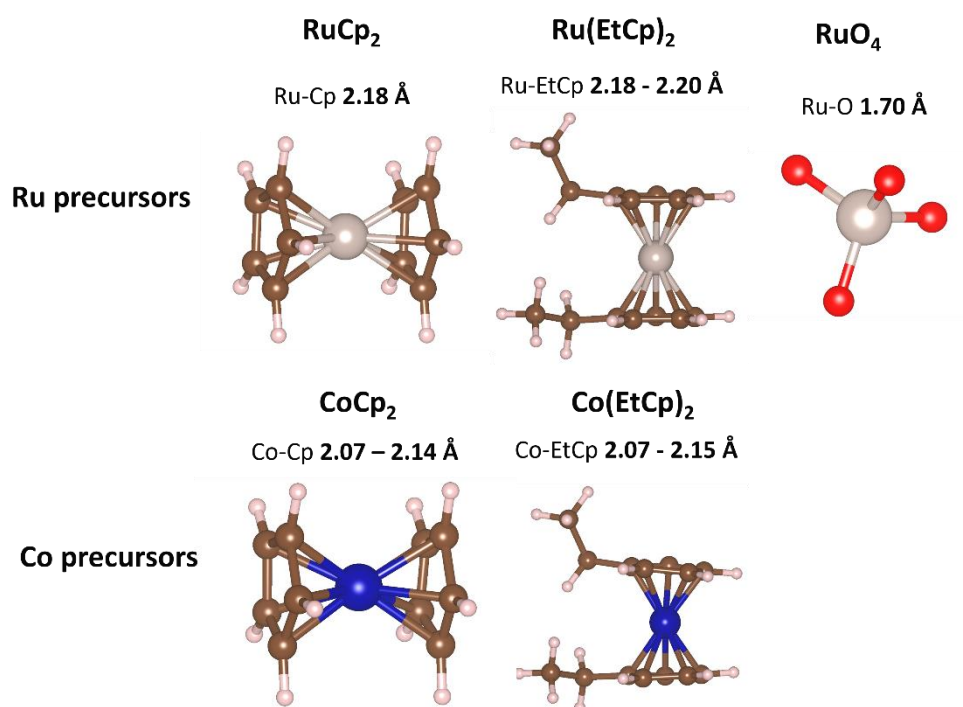
Figure A 10. Atomic structures of the ruthenium and cobalt precursors studied in chapter 8.
