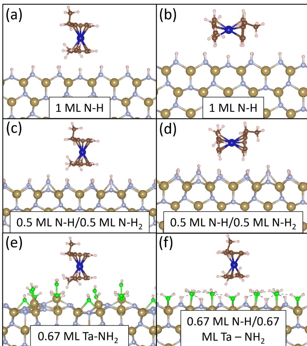
Figure 8.38. \text{Co}(\text{EtCp})_2 interaction on (a) 1 ML N-H upright interaction mode, (b) 1 ML N-H horizontal interaction mode, (c) 0.5 ML N-H/0.5 ML \text{N-H}_2 upright interaction mode, (d) 0.5 ML N-H/0.5 ML \text{N-H}_2 horizontal interaction mode, (e) 0.67 ML \text{Ta-NH}_2 and (f) 0.67 ML N-H/0.67 ML \text{Ta-NH}_2 ML upright interaction mode on the \epsilon\text{-TaN} (110) surfaces. Colour scheme is the same as in Figure 8.27.
