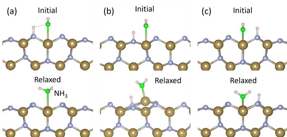
Figure 7.6: N-H and Ta- \text{NH}_2 terminations on \epsilon -Ta \text{N} (110). (a) Ta- \text{NH}_2 at \text{Ta}^{\text{B}} , (b) Ta- \text{NH}_2 at \text{Ta}^{\text{A}} and (c) Ta- \text{NH}_2 at \text{Ta}^{\text{BC}} . Colour scheme is the same as in Figure 7.3
