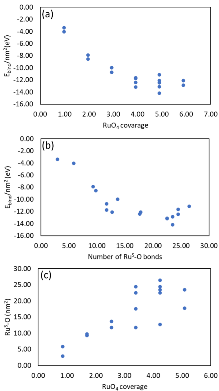
Figure 9.2 Scatter plots for (a) and (b) change in binding energy per square nanometre with change in \text{RuO}_4 coverage and coverage of \text{Ru}^{\text{S}}\text{-O} bonds respectively. (c) Coverage of \text{Ru}^{\text{S}}\text{-O} bonds versus \text{RuO}_4 coverage.
