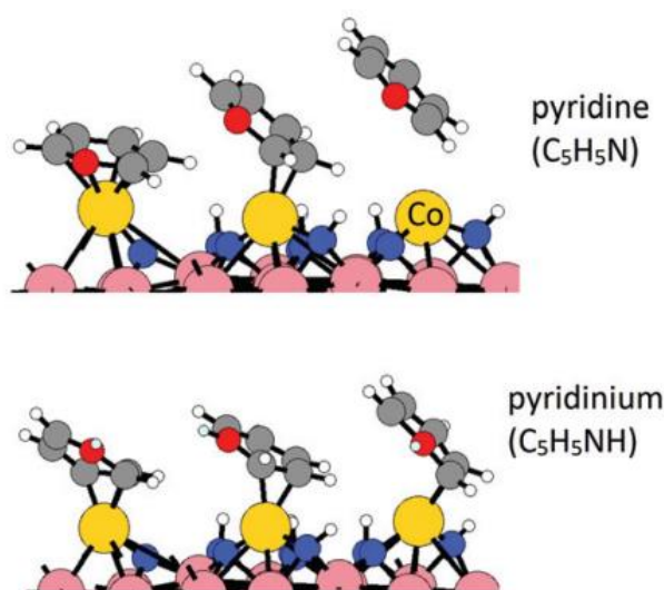
Figure 2.14: Formation of pyridine and pyridinium with N and NH radicals. Adapted from ref 182 .
