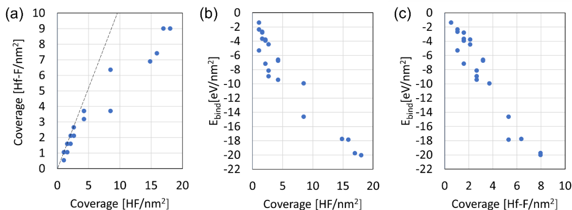
Figure 5.5: (a) Scatter plot for Hf–F coverage vs total HF coverage for the surface coverage values in Table 3. Plots (b) and (c) show the change in binding energy per square nanometer with an increase in HF and Hf–F coverage, respectively.
