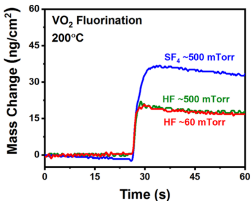
Figure 2.3 Mass changes during SF 4 and HF exposure on VO 2 . Taken from ref. 55 .
