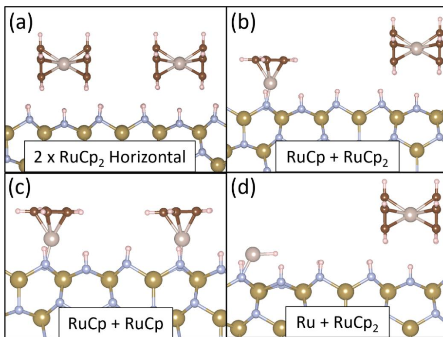
Figure 8.7. Geometries of the reaction pathway of two \text{RuCp}_2 precursors on 1 ML N-H \epsilon -TaN (110) surface for the horizontal interaction mode reaction pathway shown in panel (b) in Figure 8.5. Colour scheme is the same as in Figure 8.1.
