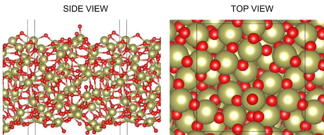
Figure 3.7: Side view and top view of aHfO 2 surface slab. Colour scheme is the same as in Figure 3.2.
