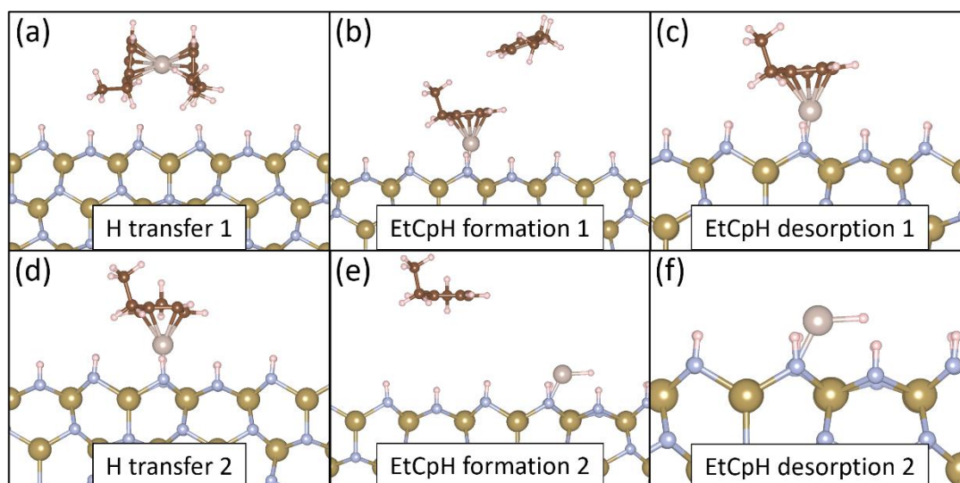
Figure 8.12. Geometries of the individual reaction pathway steps for the horizontal interaction mode of \text{Ru}(\text{EtCp})_2 on 1 ML N-H \epsilon -TaN (110). Colour scheme is the same as in Figure 8.1.
