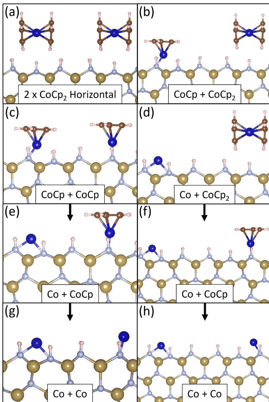
Figure 8.34: Geometries of the reaction pathway of two CoCp 2 precursors on 1 ML N-H \epsilon -TaN (110) surface for the reaction pathway shown in Figure 8.32 (b). Colour scheme is the same as in Figure 8.32.
