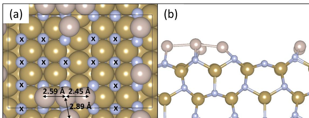
Figure 8.26. 6 x Ru on \epsilon -TaN (110) surface. (a) Top view and (b) side view. Colour scheme is Ta = brown, N = light blue and Ru = grey.
