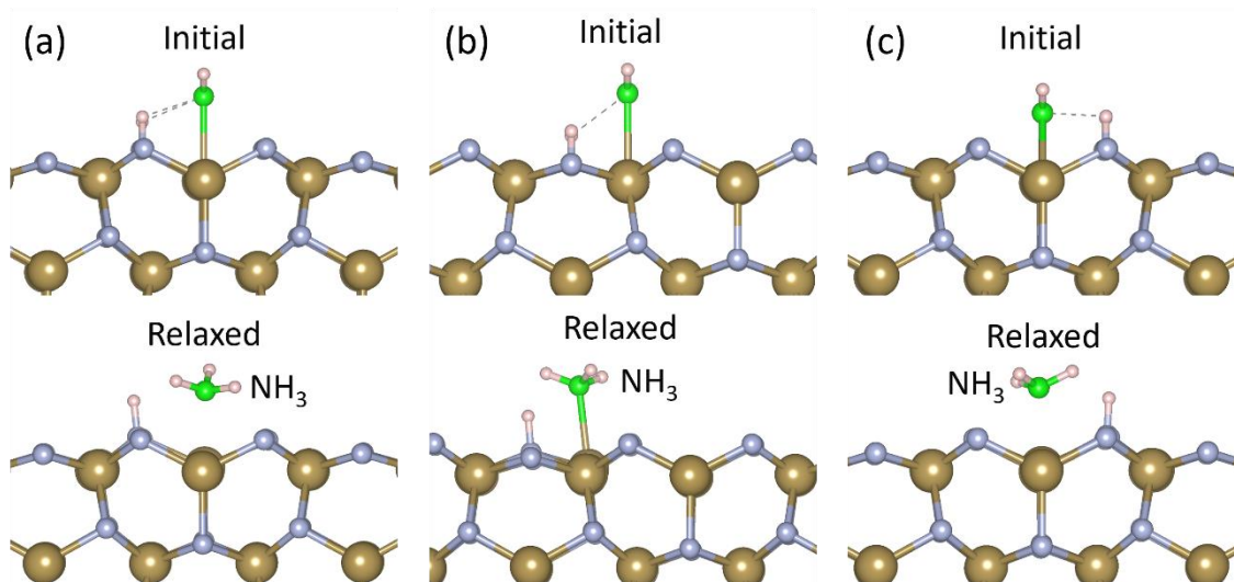
Figure 7.7: N-H 2 and Ta-NH 2 terminations on \epsilon -TaN (110). (a) Ta-NH 2 at Ta B , (b) Ta-NH 2 at Ta A and (c) Ta-NH 2 at Ta BC . Colour scheme is the same as in Figure 7.3.
