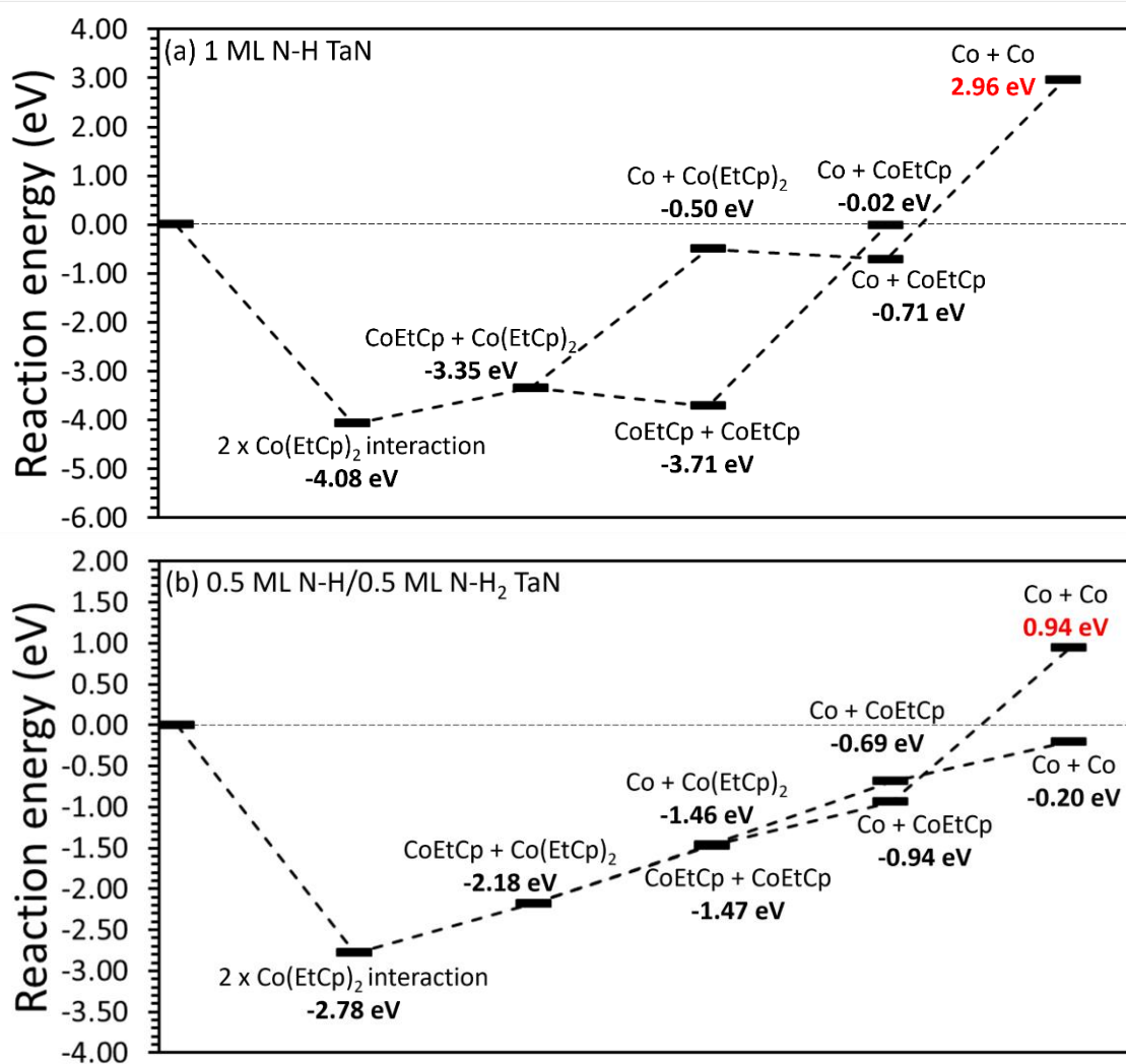
Figure 8.43 Reaction pathway for two Co(EtCp) 2 precursors on (a) 1 ML N-H surface and (b) 0.5 ML N-H/0.5 ML N-H 2 \epsilon -TaN (110) surfaces.
