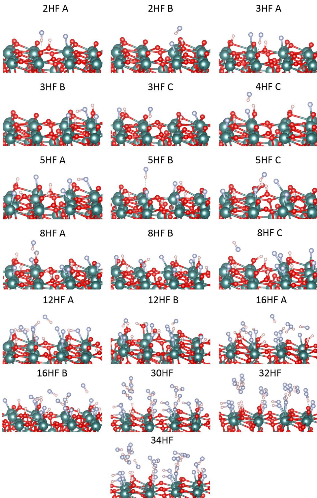
Figure A 2: Relaxed geometries for different HF coverages of \text{ZrO}_2 where a mixture of molecular and dissociative adsorption of HF is observed. Colour scheme: Zr = green, O = red and H = white.
