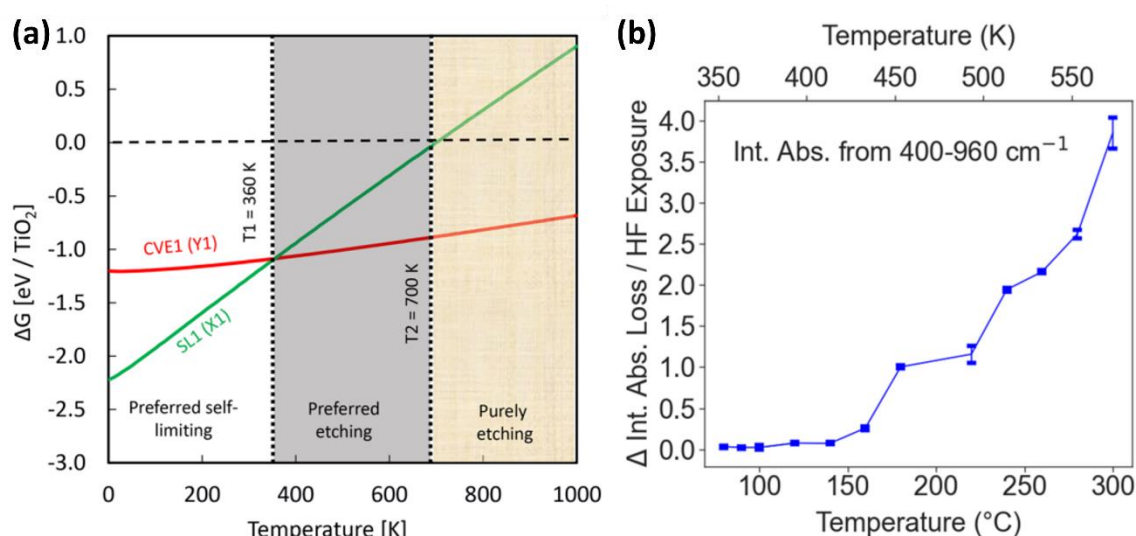
Figure 2.7: Combined computational and experimental TiO 2 thermal ALE study. (a) FEPs of continuous etch (CVE1 – red line) and self-limiting (SL1 – green line). (b) Etch rate measured by change in integrated FTIR absorbance of the Ti–O vibrational modes from 80 to 300 °C. Adapted from ref 53 .
