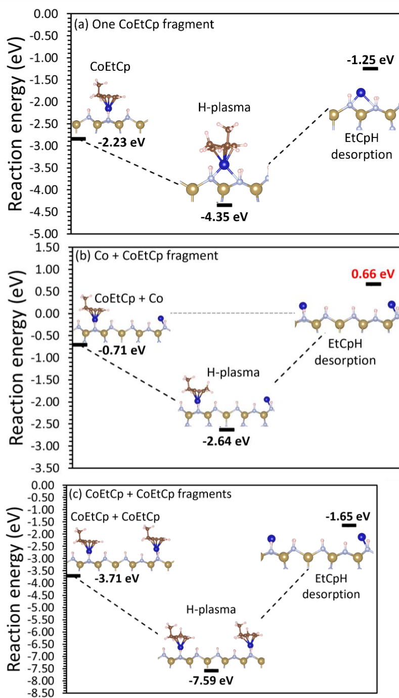
Figure 8.46 Reaction pathway of \cdot\text{H} radical treated (a) CoEtCp 0.96 ML N-H, (b) Co & CoEtCp 0.88 ML N-H and (c) (\text{CoEtCp})_2 0.92 ML N-H \epsilon -TaN (110) surfaces. Colour scheme is the same as in Figure 8.27.
