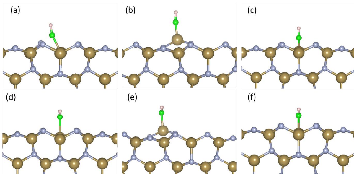
Figure 7.3: Single \text{Ta-NH}_x adsorbed at different Ta sites on \epsilon\text{-TaN}(110) surface with N atoms from \text{NH}_x species highlighted in green for clarity. (a) \text{Ta-NH} at Ta c.n. 3, (b) \text{Ta-NH} at Ta c.n. 6, (c) \text{Ta-NH} bridging between two surface Ta c.n. 3 atoms, (d) \text{Ta-NH}_2 at Ta c.n. 3, (e) \text{Ta-NH}_2 at Ta c.n. 6 and (f) \text{Ta-NH}_2 bridging between two surface Ta c.n. 3 atoms. Colour scheme is: Ta = brown, N = blue & green and H = pink.
