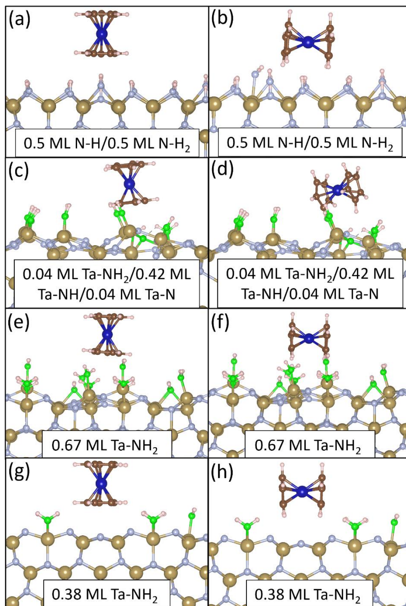
Figure A 8. CoCp 2 adsorption at NH x -terminated TaN surfaces. Colour scheme is Ta = brown, N = blue & green, H = pink, C = dark brown and Co = dark blue.
