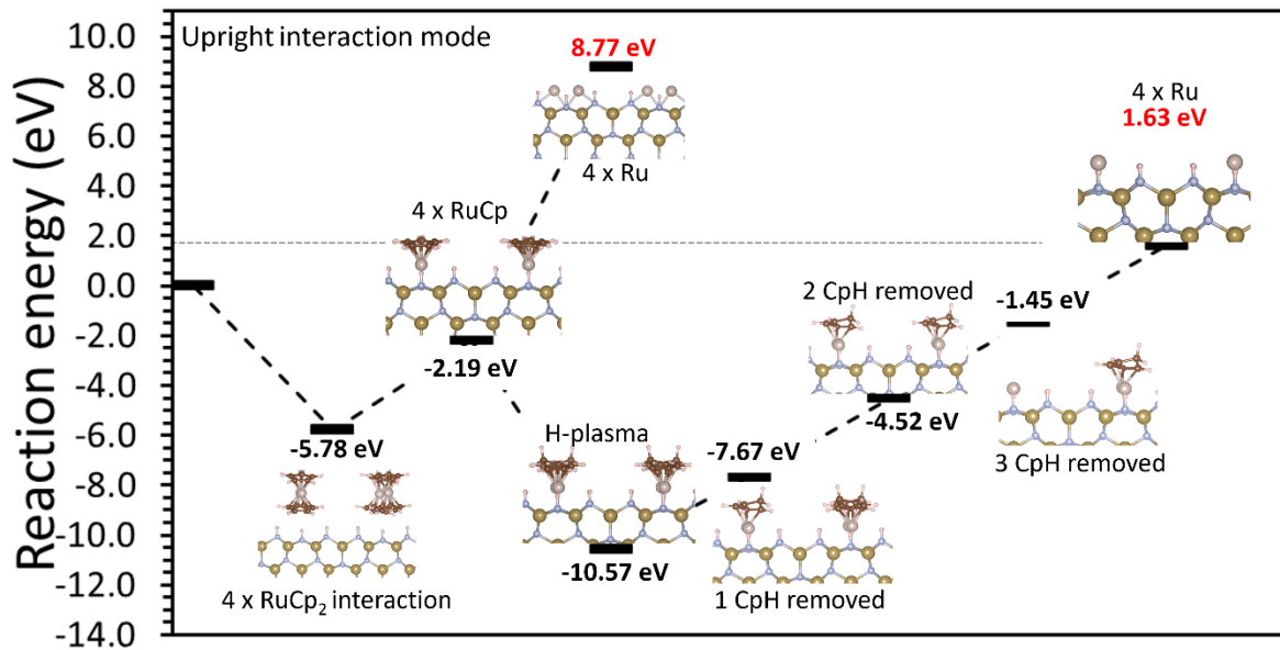
Figure 8.8. Reaction pathway for H plasma chemistry at four \text{RuCp}_2 precursors on the 1 ML N-H \epsilon -TaN (110) surface. Colour scheme is the same as in Figure 8.1.
