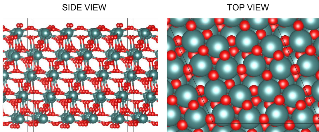
Figure 3.6: Side view and top view of monoclinic (111) surface supercell of ZrO 2 . Colour scheme: Zr = green and O = red.
