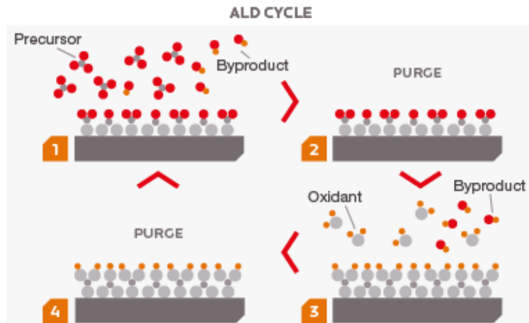
Figure 1.1: Schematic representation of ALD cycle. Source ASM 51 .
