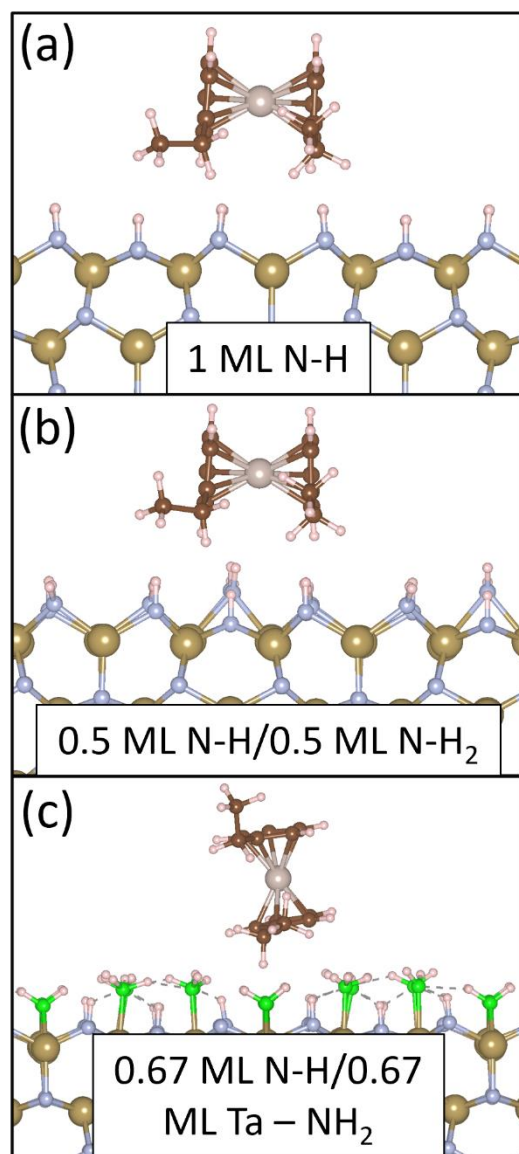
Figure 8.10. Ru(EtCp) 2 interaction on (a) 1 ML N-H horizontal interaction mode, (b) 0.5 ML N-H/0.5 ML N-H 2 horizontal interaction mode and (c) 0.67 ML N-H/0.67 ML Ta-NH 2 upright interaction mode \epsilon -TaN (110) surfaces.
