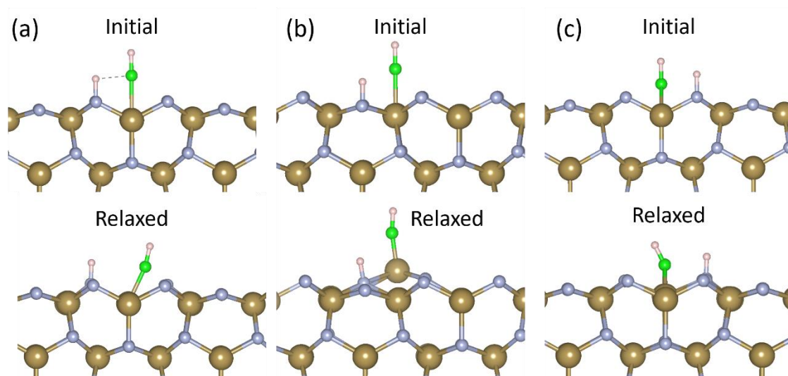
Figure 7.4: N-H and Ta-NH terminations on \epsilon -TaN(110). (a) Ta-NH at Ta B , (b) Ta-NH at Ta A and (c) Ta-NH at Ta BC . Colour scheme is the same as in Figure 7.3
