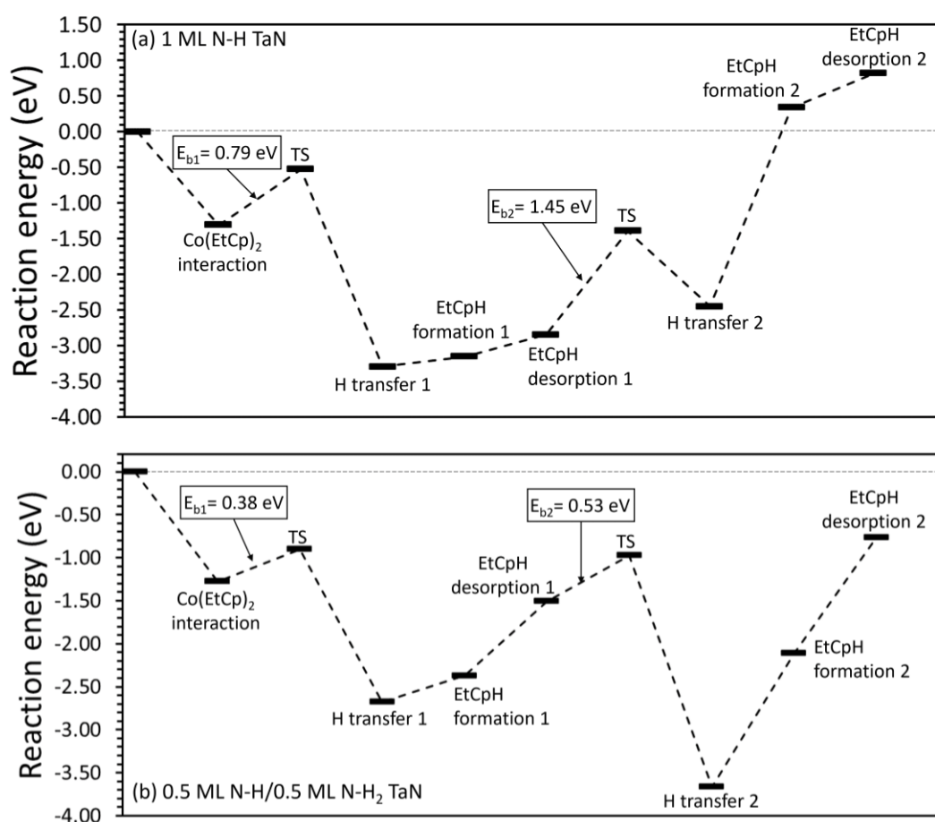
Figure 8.39. \text{Co}(\text{EtCp})_2 reaction pathway on (a) 1 ML N-H and (b) 0.5 ML N-H/0.5 ML N-H 2 \epsilon -TaN (110) for the upright interaction mode.
