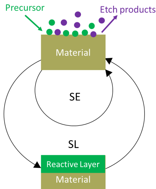
Figure 2.5: Schematic representation of the bulk to gas continuous spontaneous etch (SE) and surface to surface self-limiting (SL).
