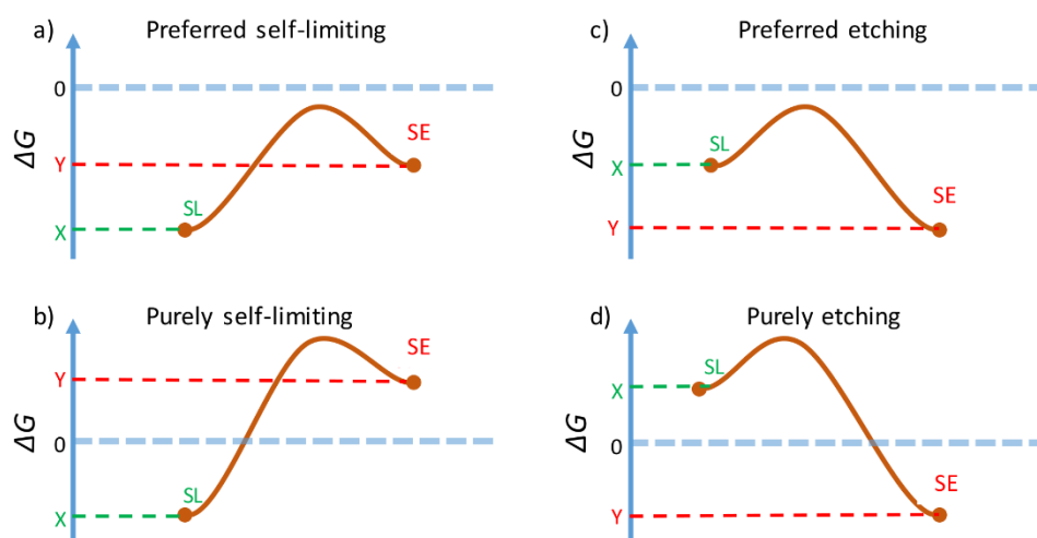
Figure 3.13: Schematic energy profiles representing (a) preferred self-limiting, (b) purely self-limiting, (c) preferred etching, and (d) purely etching.
