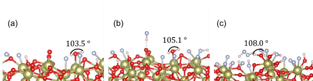
Figure 5.6: Relaxed geometries for HF coverages (a) 5HF C, (b) 8HF C, and (c) 16HF A where H 2 O formed spontaneously. Colour scheme same as in Figure 5.3.
