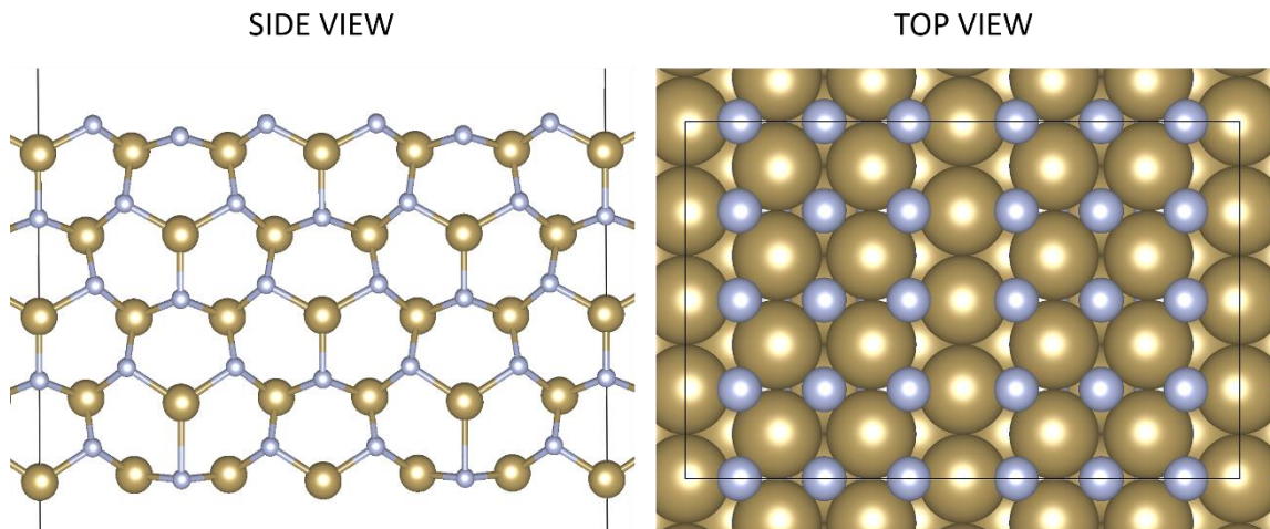
Figure 3.11: Side view and Top view of the TaN (110) surface. Colour scheme is: Ta = brown and N = blue.
