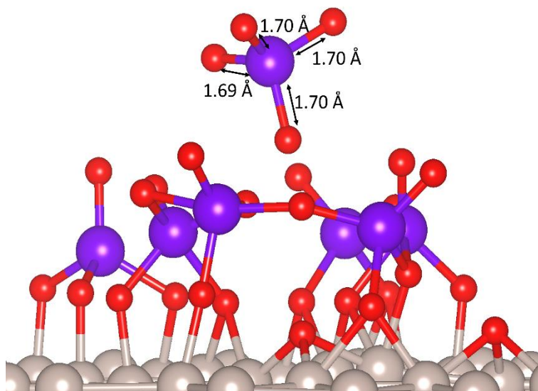
Figure 9.3 Atomic structure after interaction of the 7th \text{RuO}_4 on the 6 \times \text{RuO}_4 terminated Ru surface. Colour scheme is: Ru = grey, O = red and Ru from \text{RuO}_4 = purple.
