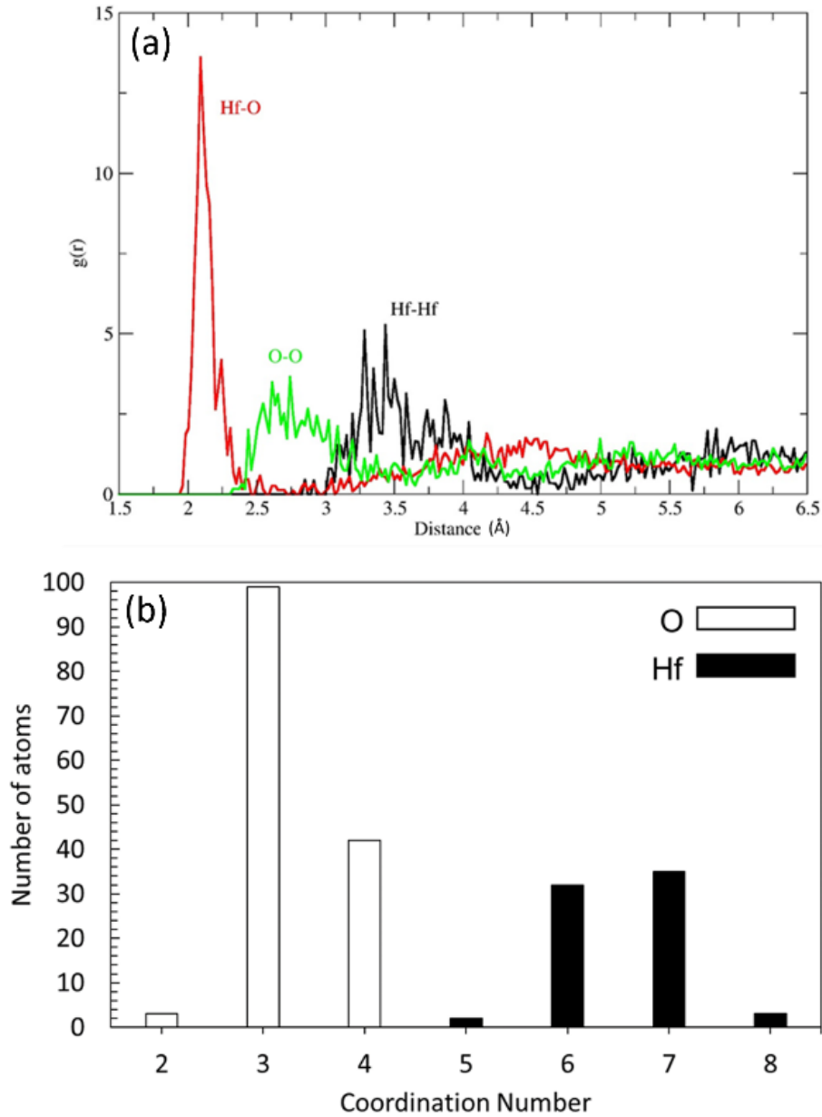
Figure 3.8: (a) Pair distribution function (PDF) of amorphous \text{HfO}_2 bulk model structure quenched at 10 K/ps rate and the plot uses 300 data points (b) distribution of coordination numbers for the bulk \text{aHfO}_2 model used in this thesis that was prepared using classical molecular dynamics.
