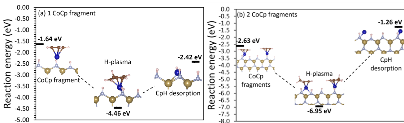
Figure 8.36 Reaction pathways of \cdot\text{H} radical treated (CoCp) x terminated (a) 0.96 ML N-H and (b) 0.92 ML N-H \epsilon -TaN (110) surfaces. Colour scheme is the same as in Figure 8.27.
