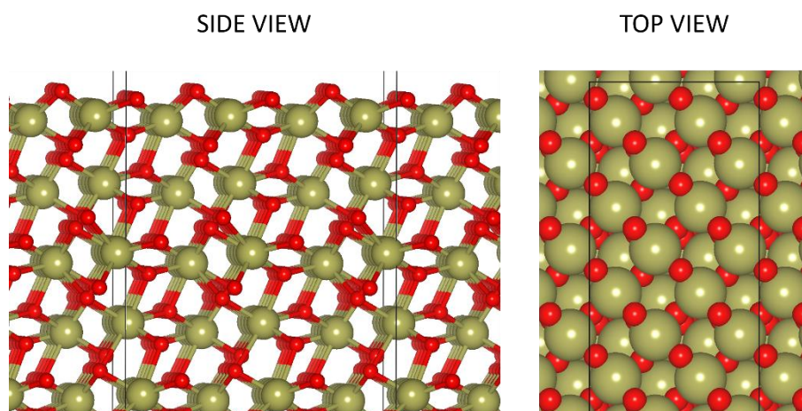
Figure 3.3: Side view and top view of monoclinic (001) surface supercell of \text{HfO}_2 . Colour scheme is the same as in Figure 3.2.
