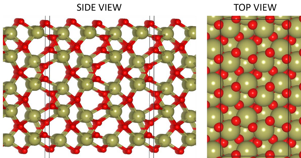
Figure 3.5: Side view and top view of orthorhombic (001) surface supercell of HfO 2 . Colour scheme is the same as in Figure 3.2.
